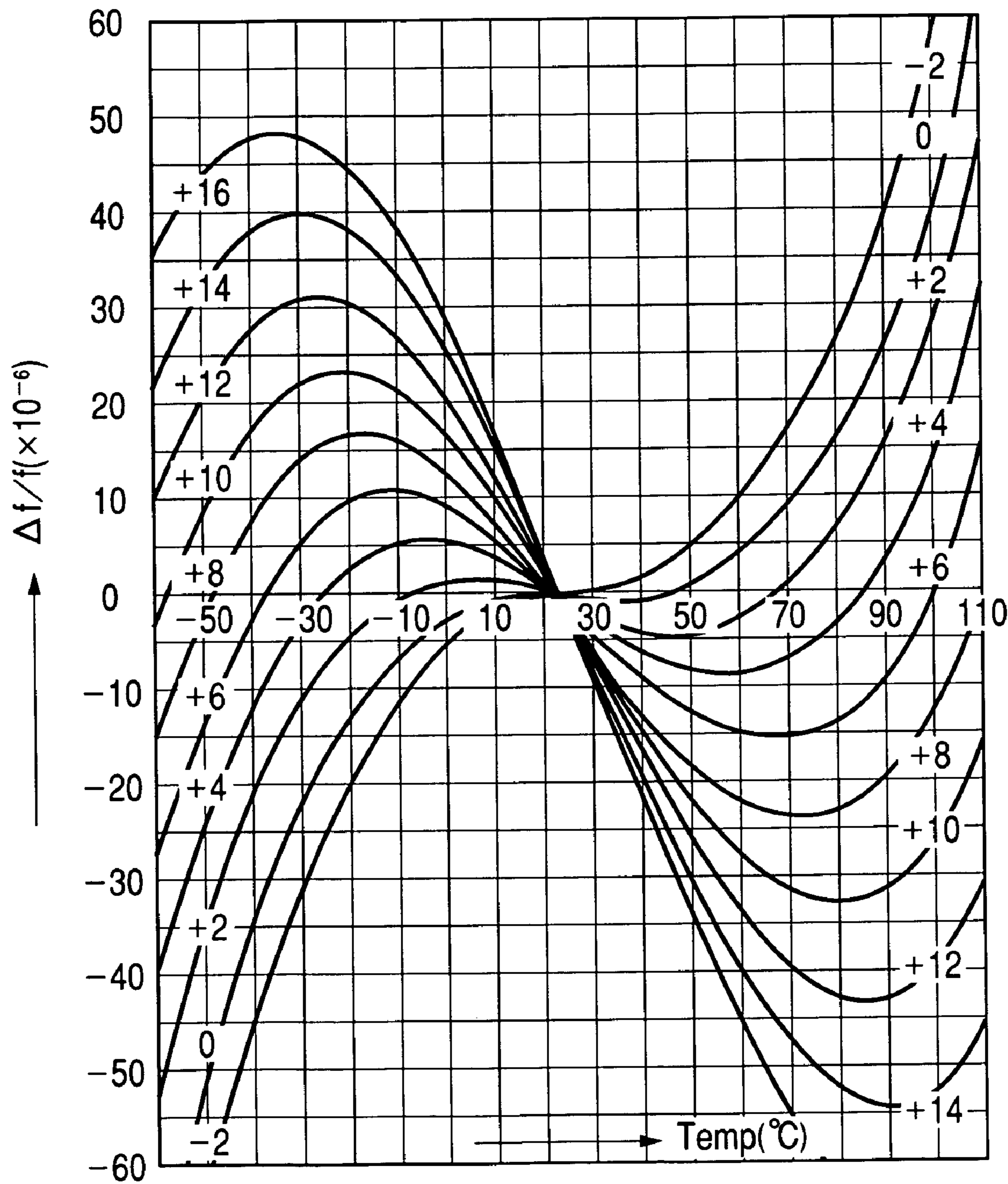
EXAMPLE OF FREQUENCY-TEMPERATURE CHARACTERISTIC OF AT-CUT
