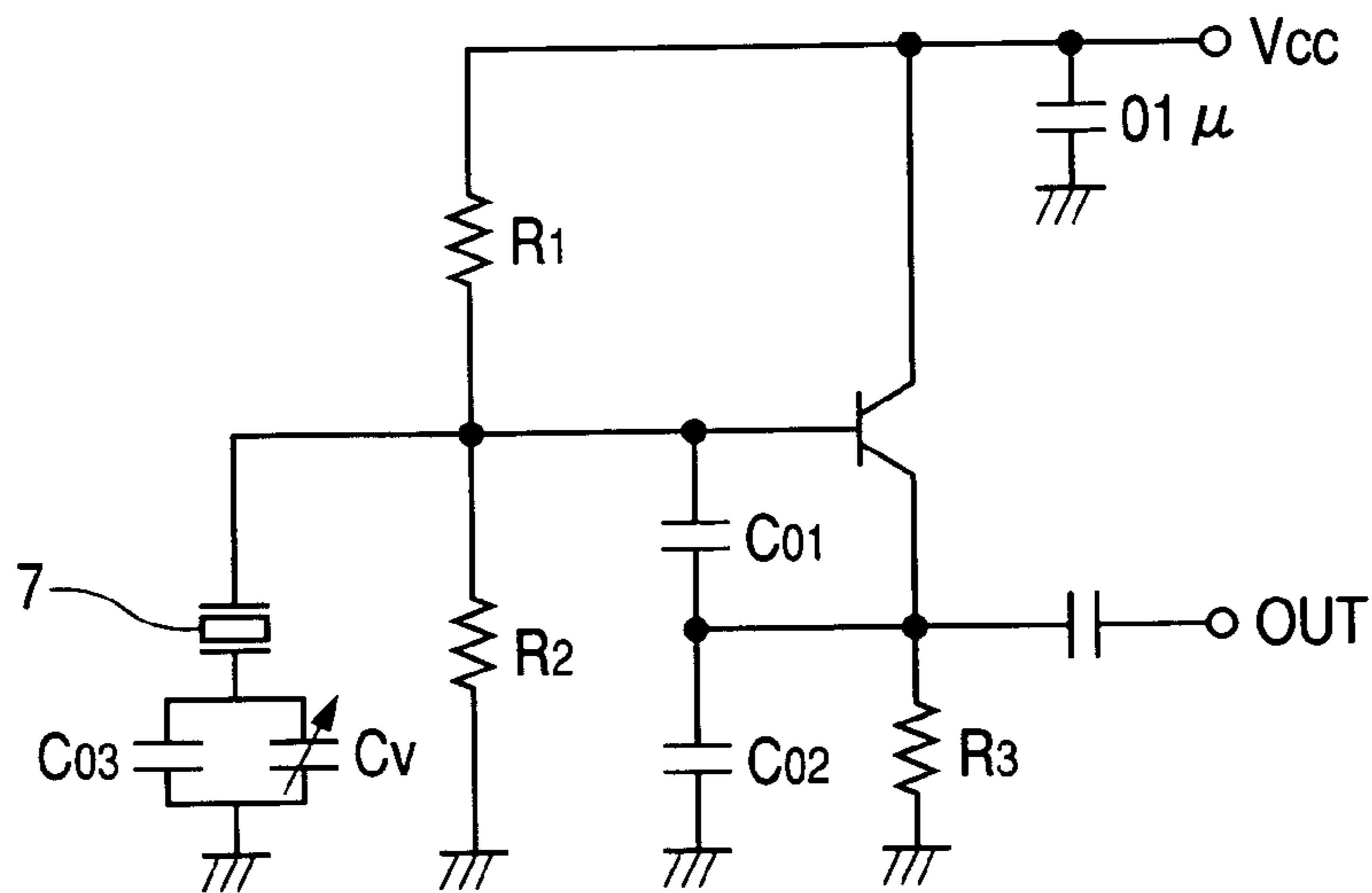
STANDARD BASIC-WAVE OSCILLATOR CIRCUIT
