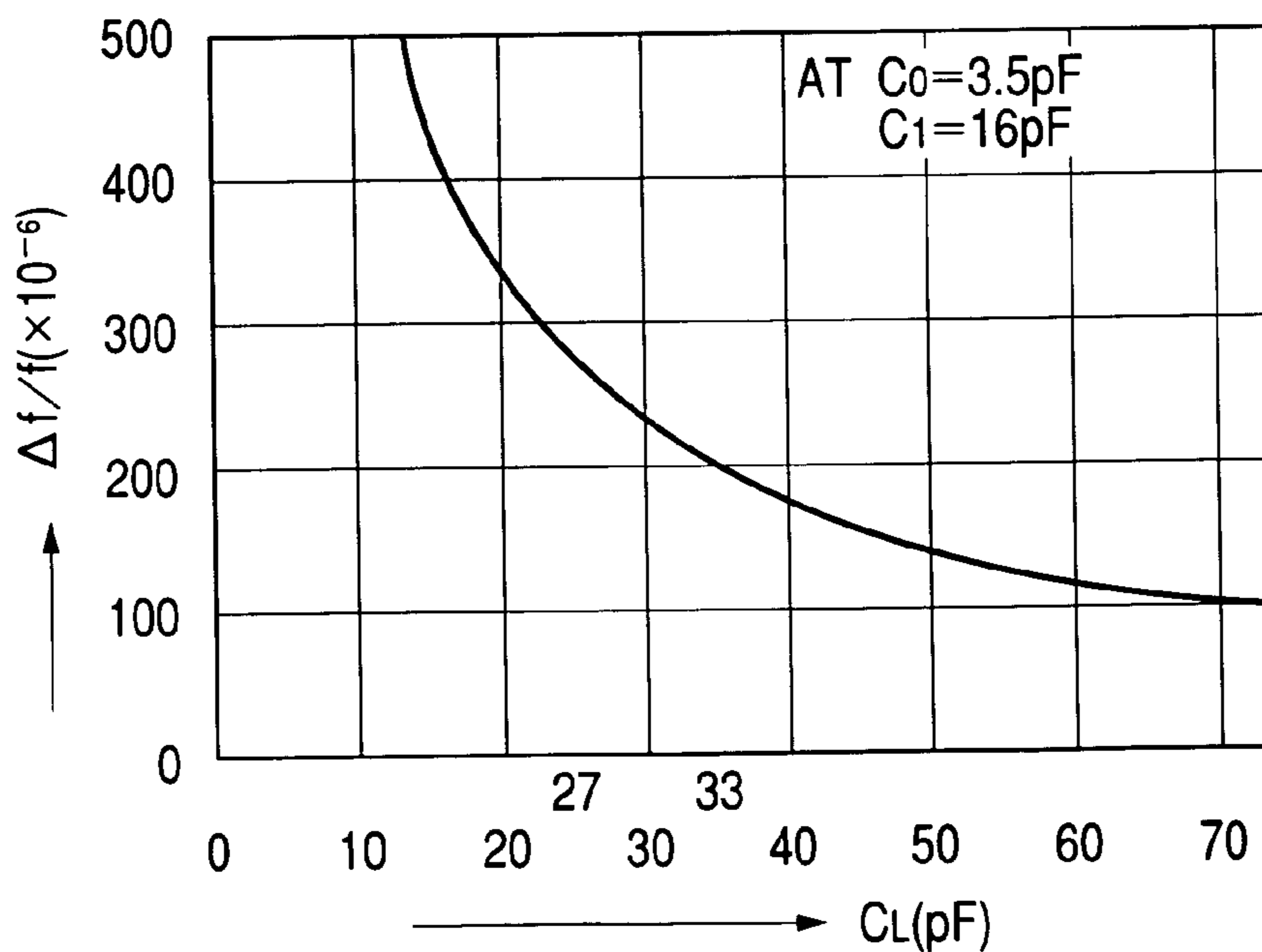
LOAD-CAPACITANCE CHARACTERISTIC OF OSCILLATOR
