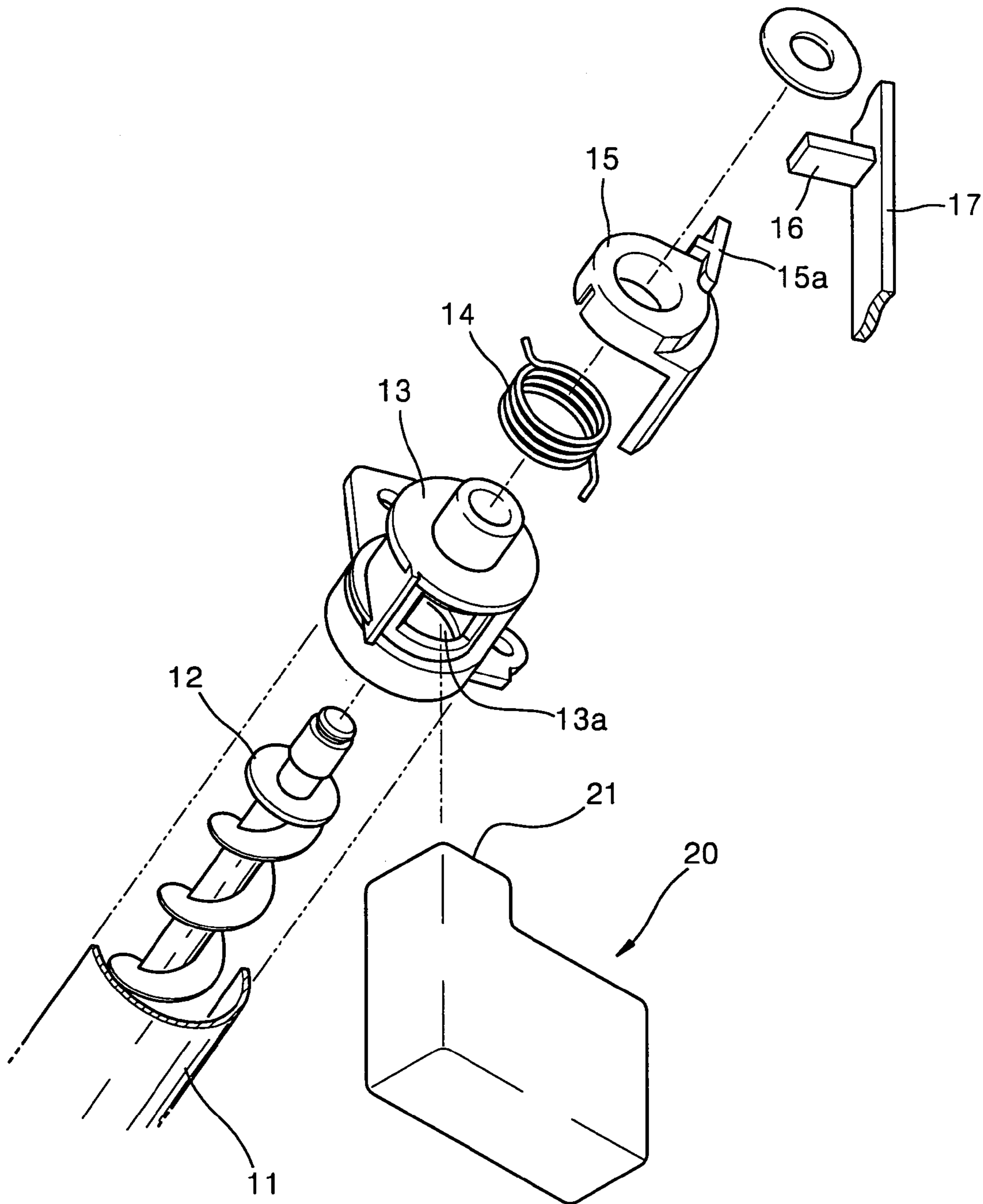
FIG. 2 (PRIOR ART)
