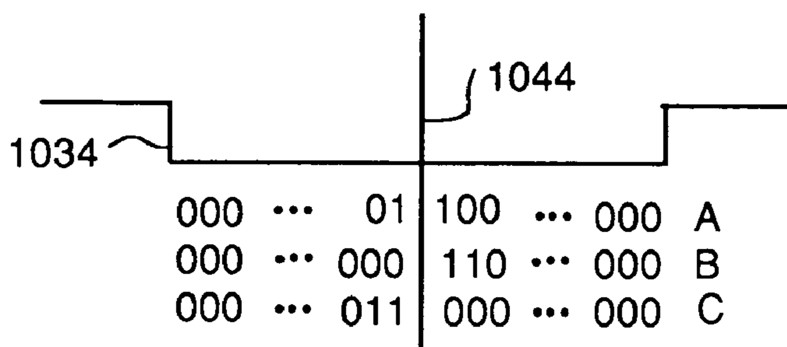
FIG. 37 FINE TUNING TO CENTER BARKER CODE
