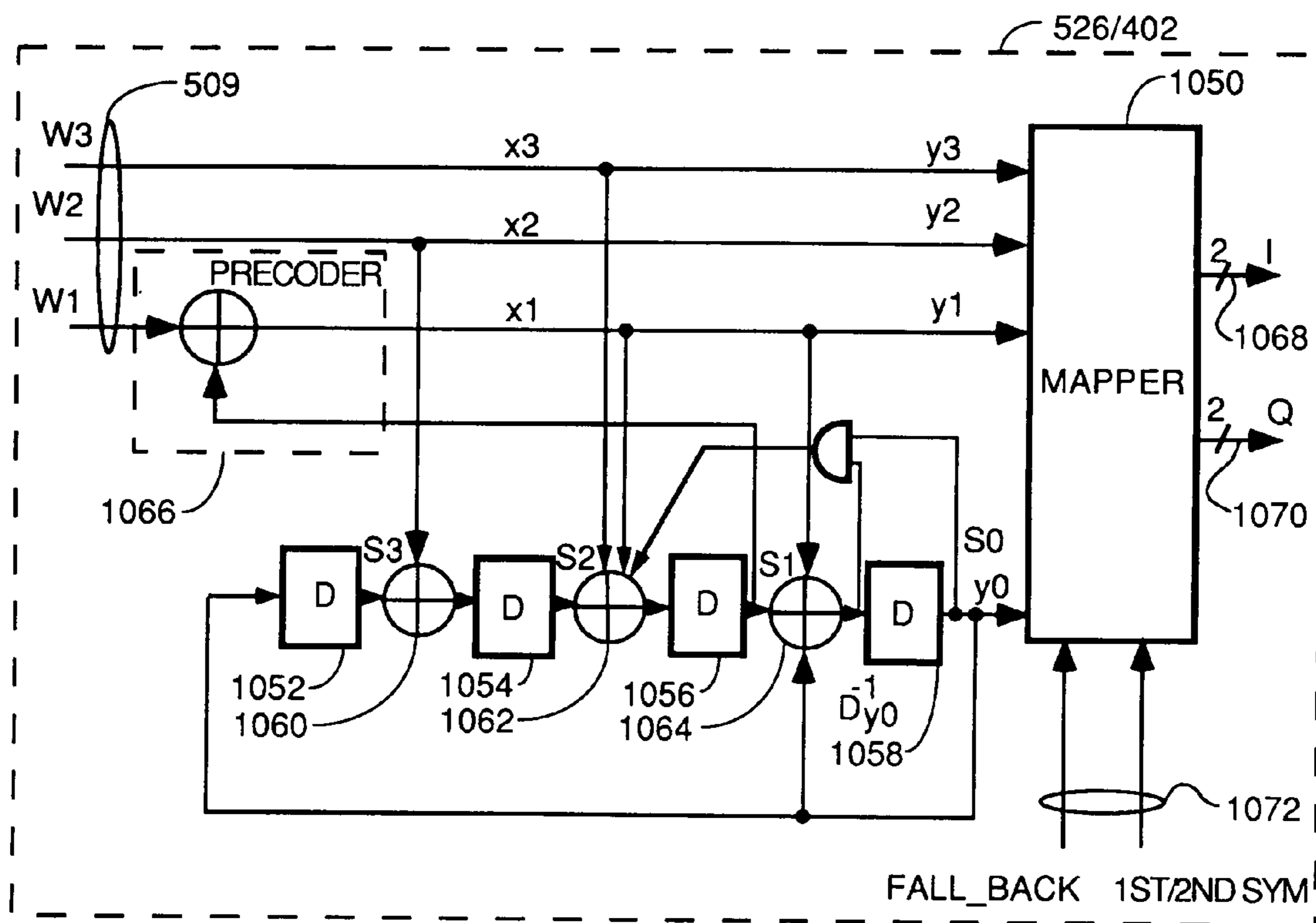
PREFERRED TRELIS ENCODER
