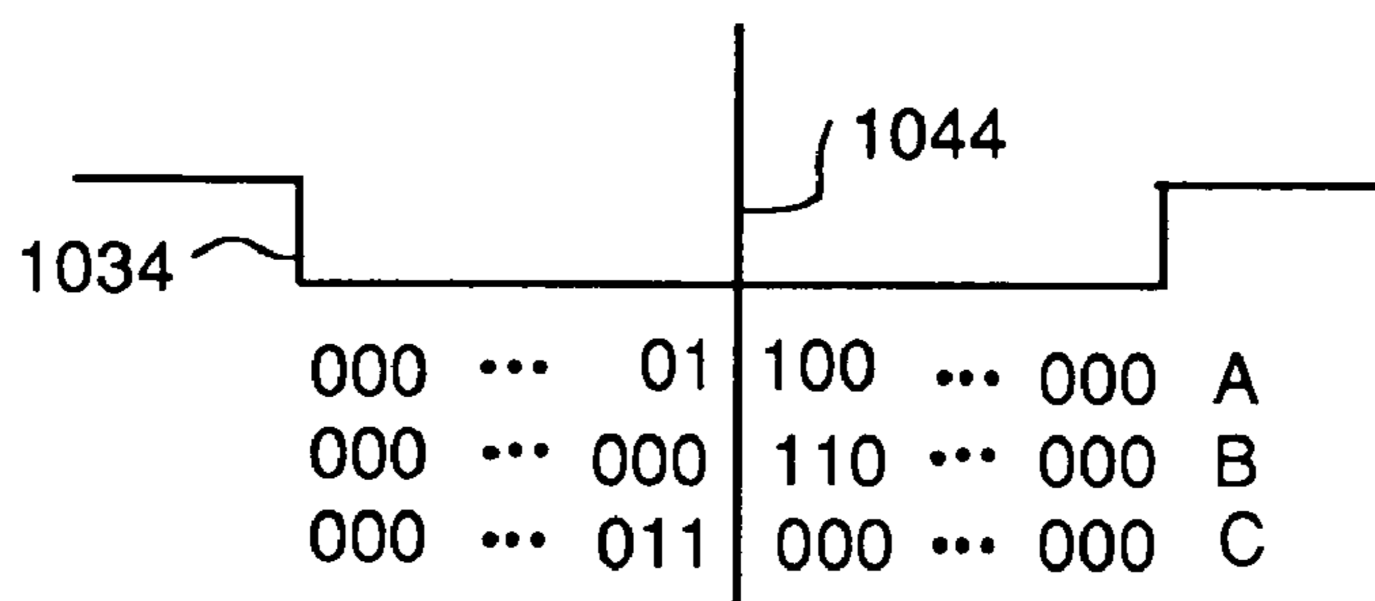
FIG. 37 FINE TUNING TO CENTER BARKER CODE
