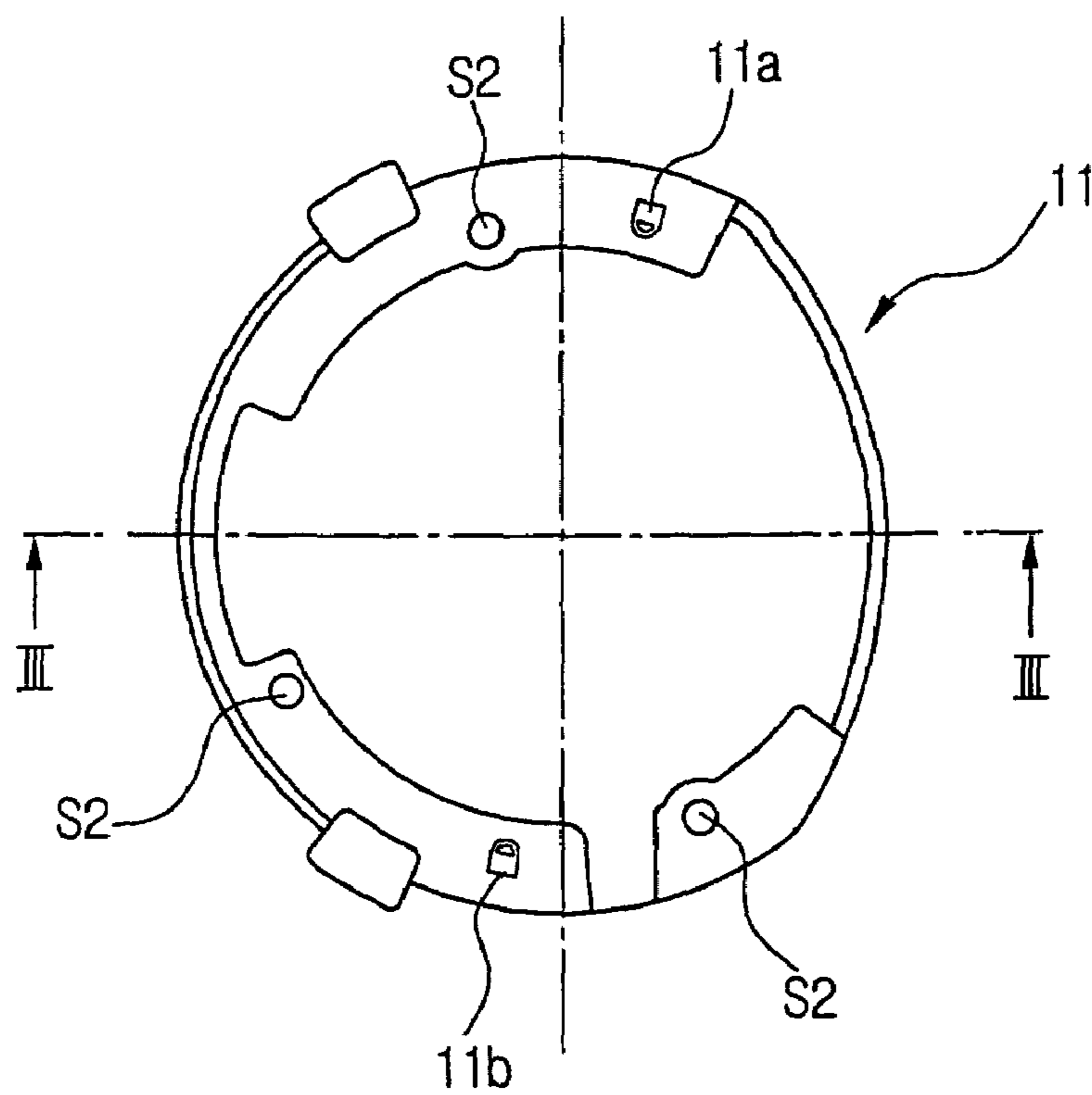
FIG. 2 (PRIOR ART)
