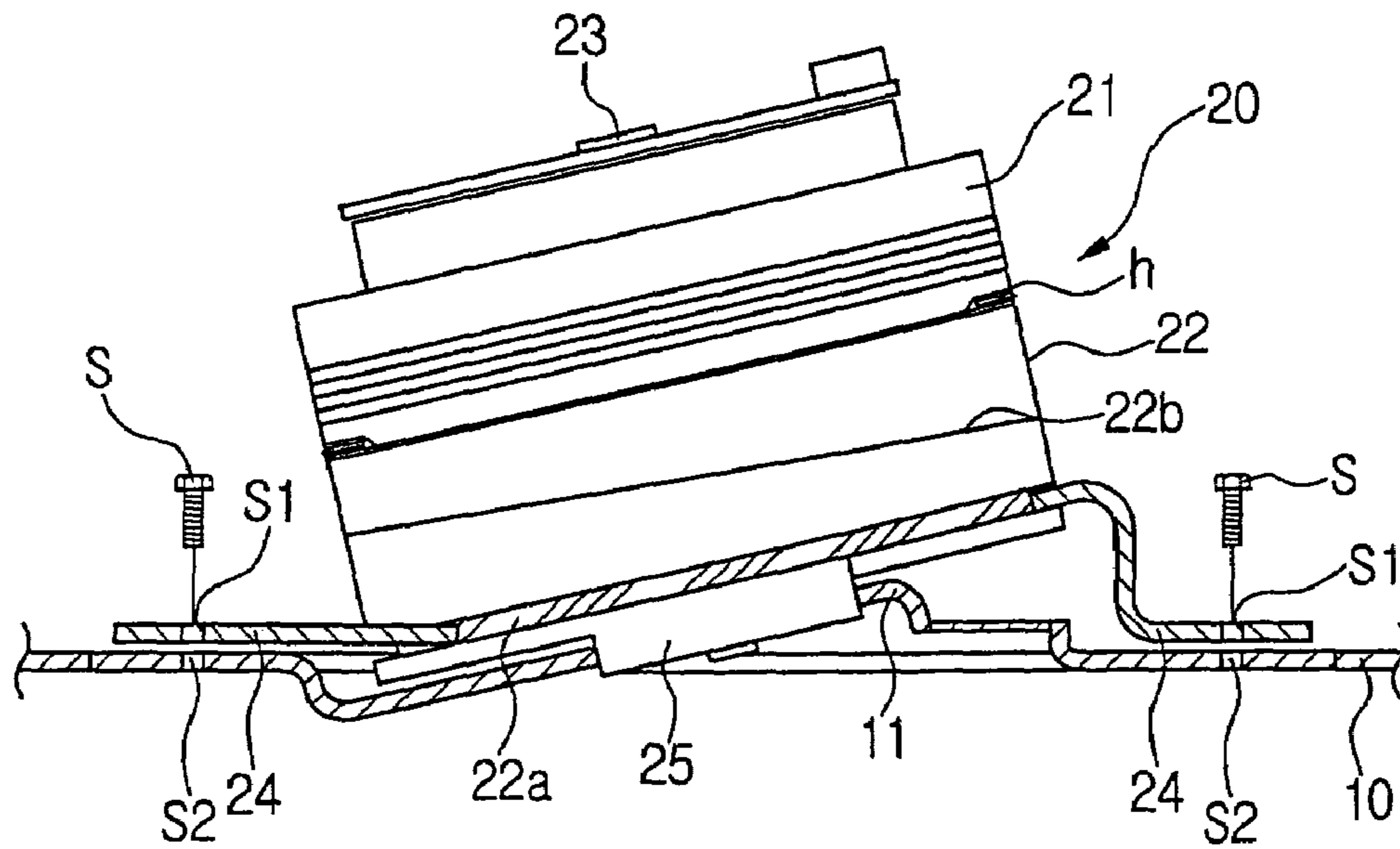
FIG. 2 (PRIOR ART)
