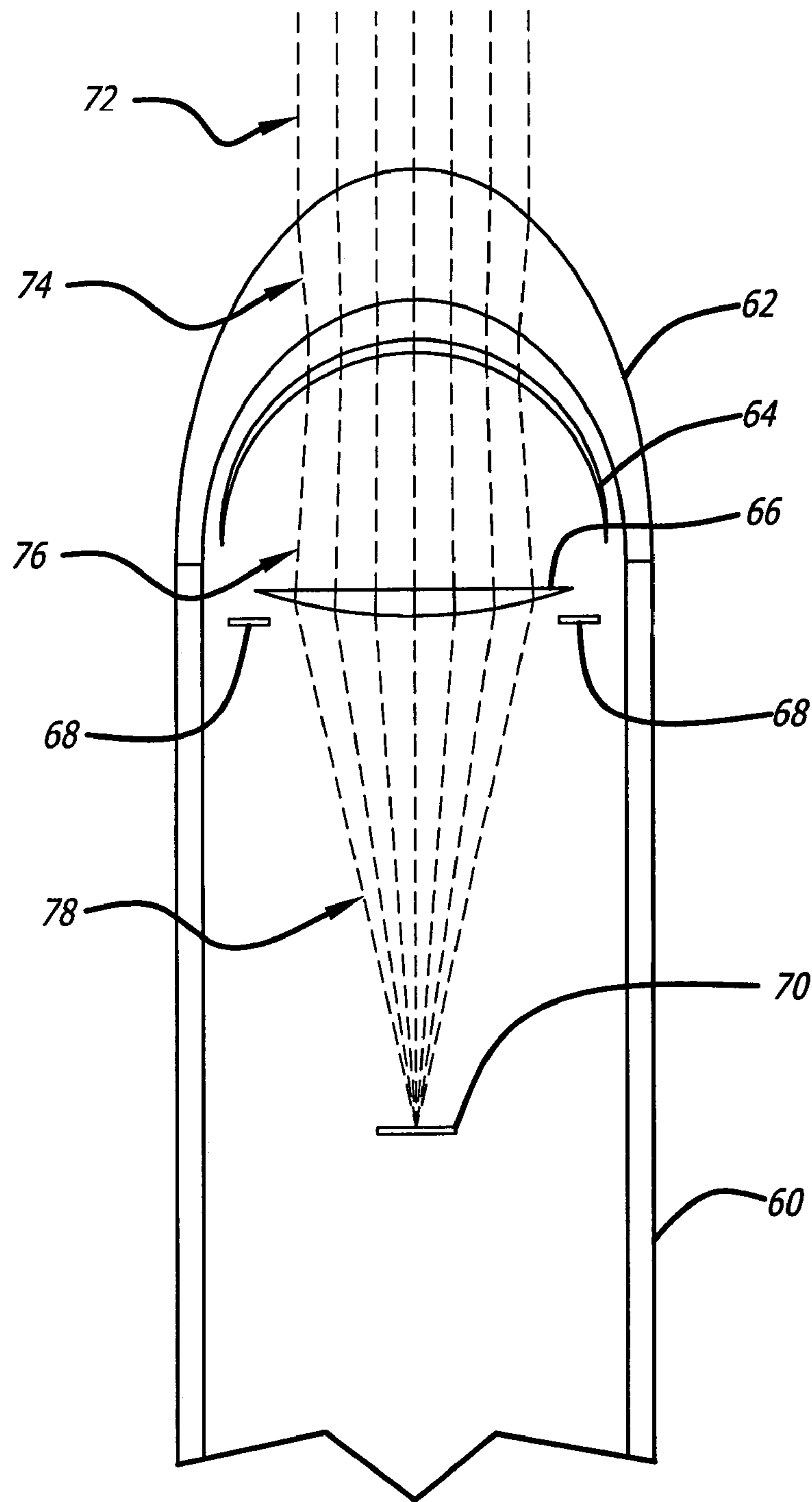
FIG. 4 (Prior Art)
