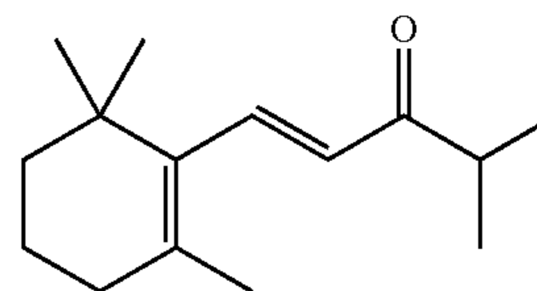
2,4-dimethyl-1-(2,6,6-trimethylcyclohex-1-en-1-yl)pent-1-en-3-one
