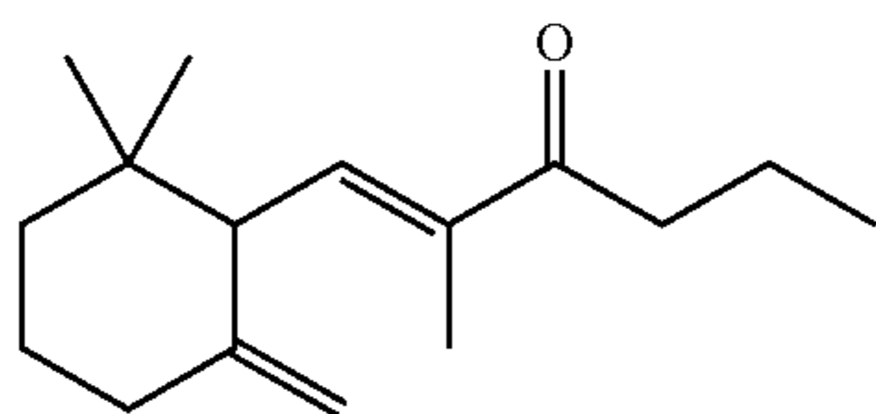
3-ethyl-4-(2,6,6-trimethylcyclohex-1-en-1-yl)but-3-en-2-one
