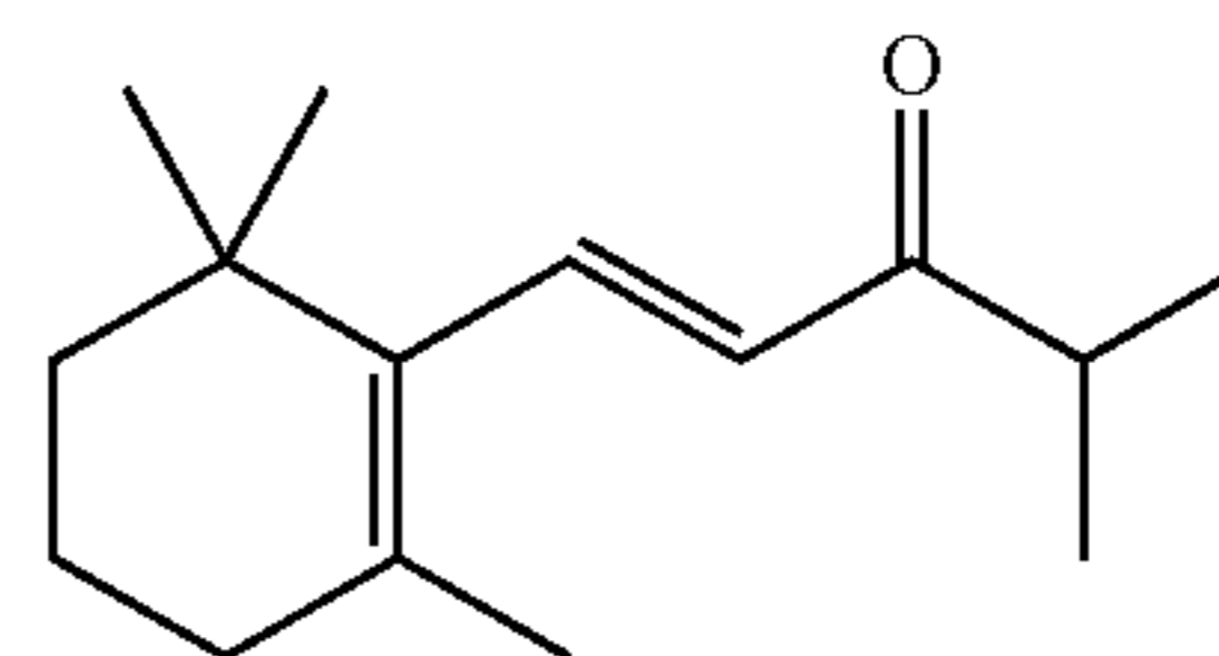
2,4-dimethyl-1-(2,6,6-trimethylcyclohex-1-en-1-yl)pent-1-en-3-one
