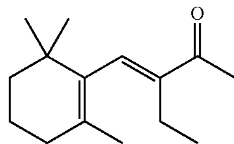
1-(2,6,6-trimethylcyclohex-2-en-1-yl)hex-1-en-3-one
