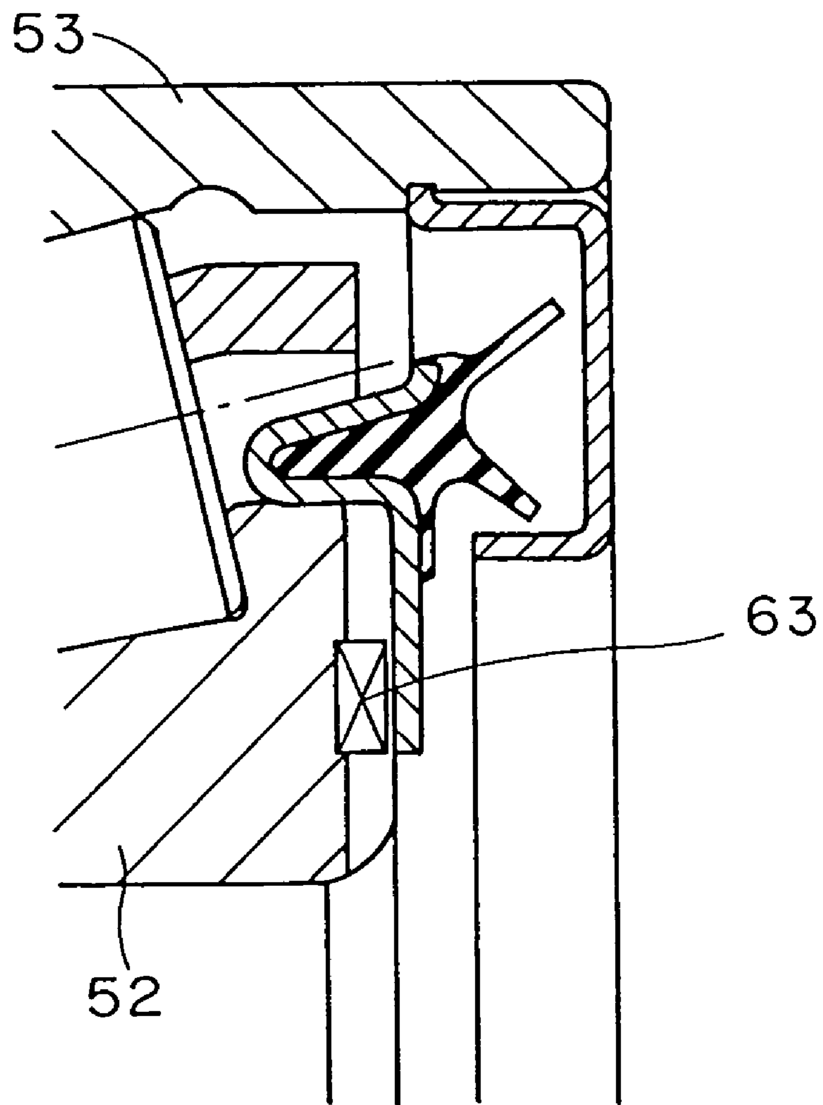
Fig. 8 PRIOR ART
