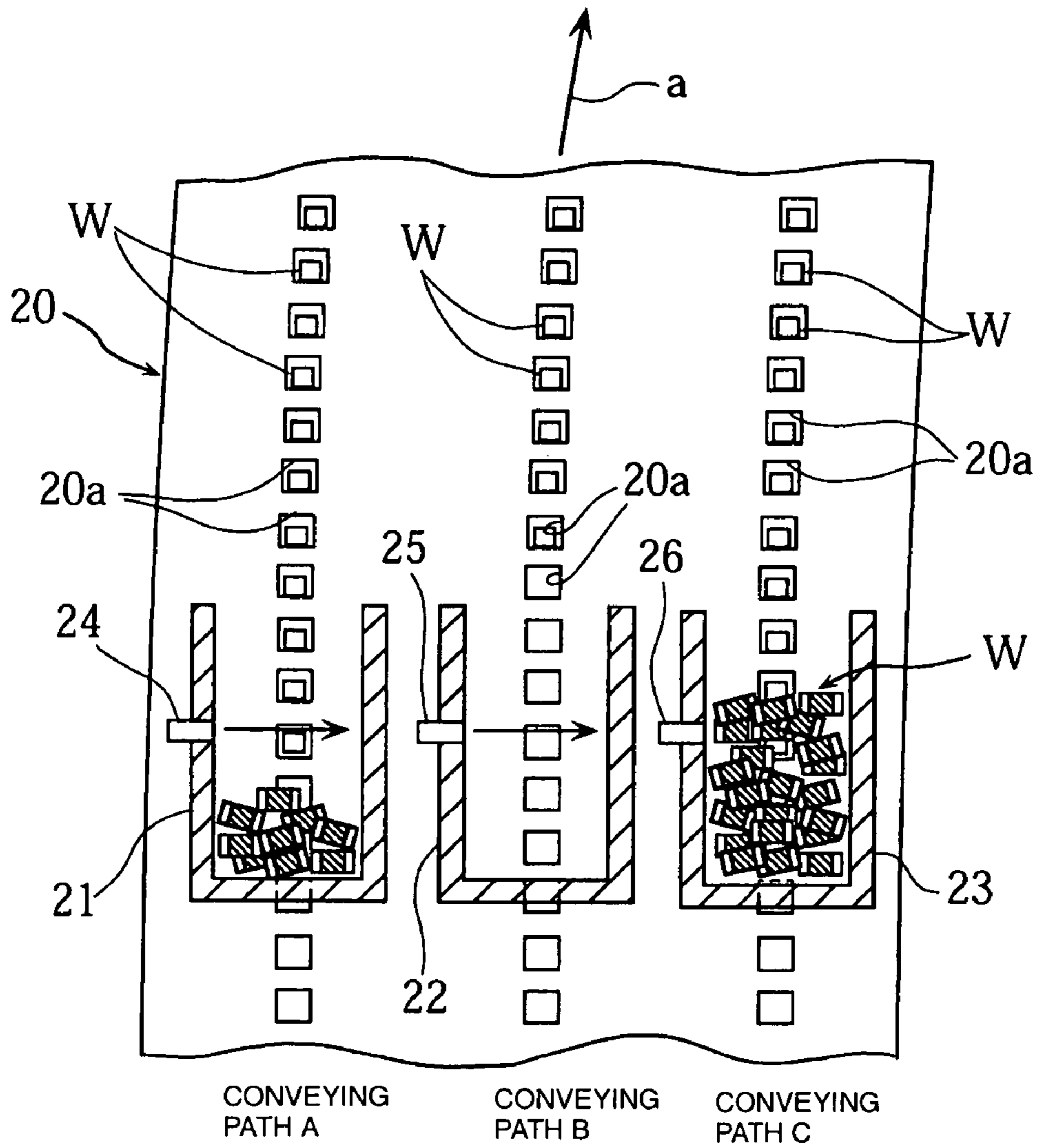
FIG. 5 PRIOR ART
