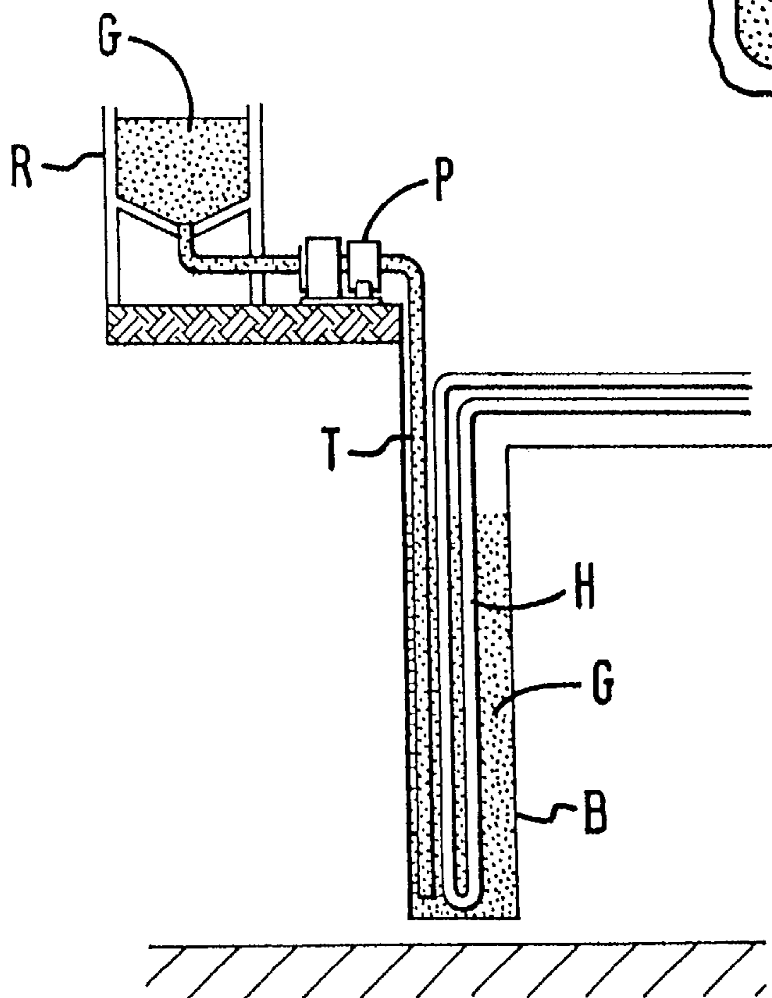
FIG. 2 Prior Art
