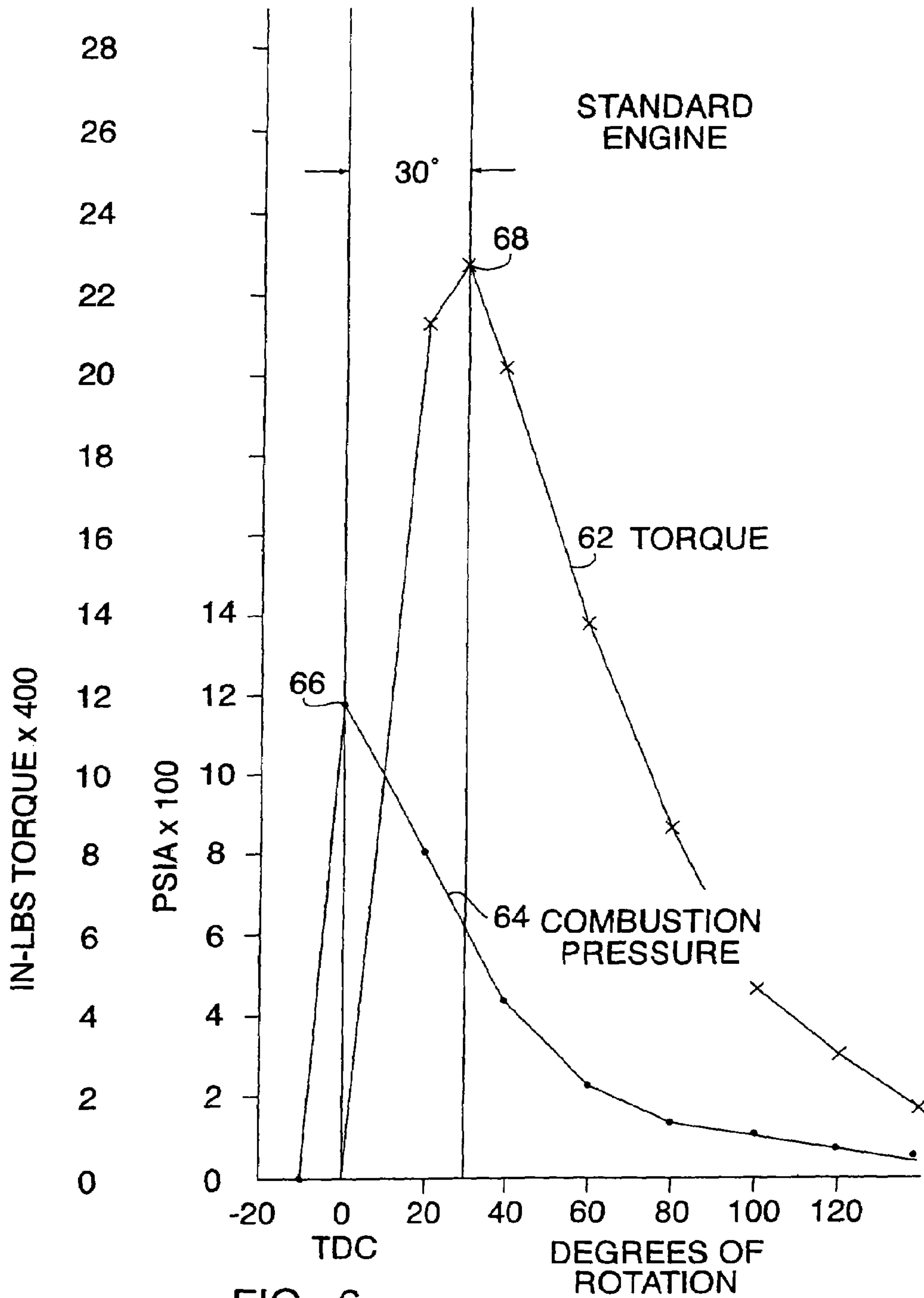
FIG. 6 PRIOR ART
