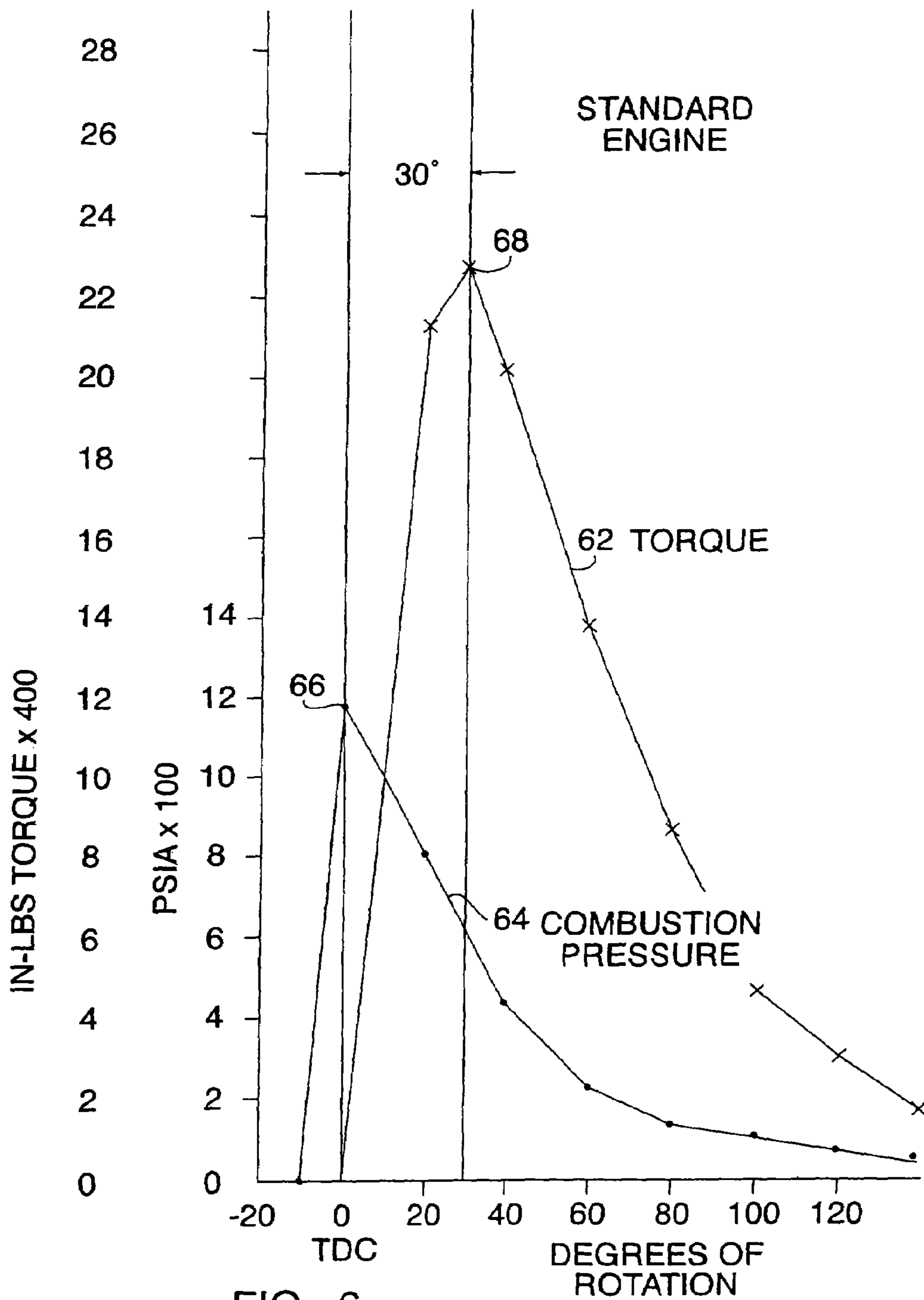
FIG. 6 PRIOR ART
