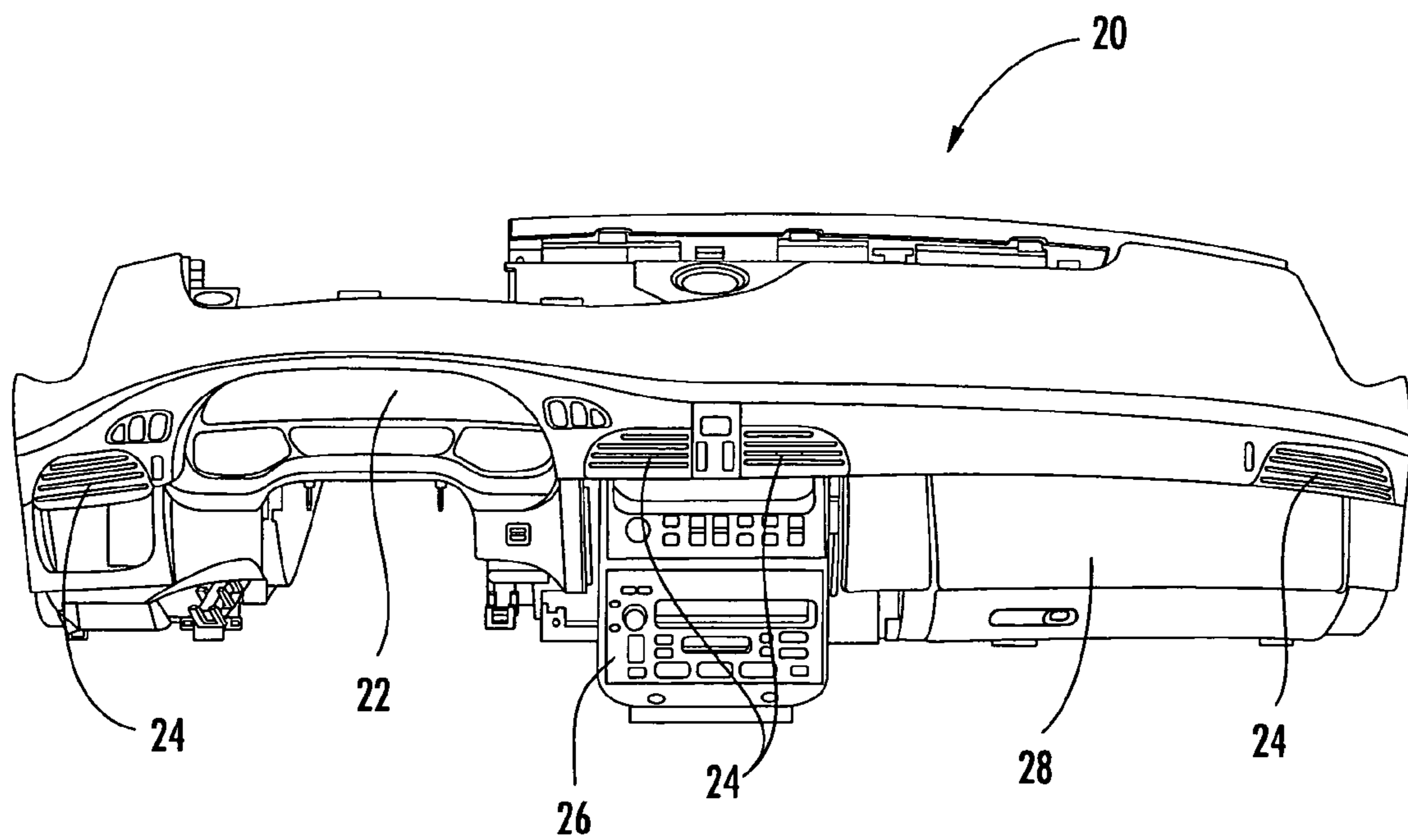
FIG. 2. PRIOR ART
