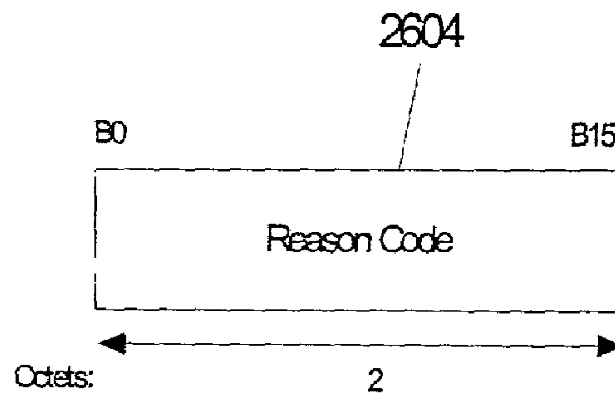
Figure 26B (Reason Code Fixed Field)
