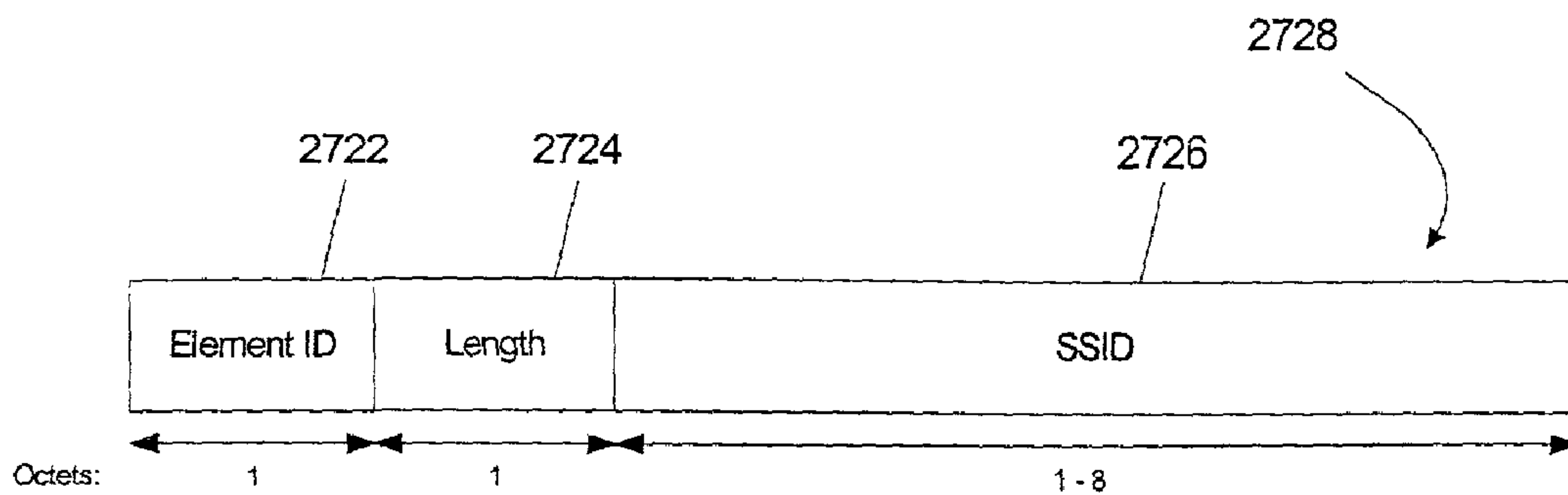
Figure 27B (SSID Information Element Format)
