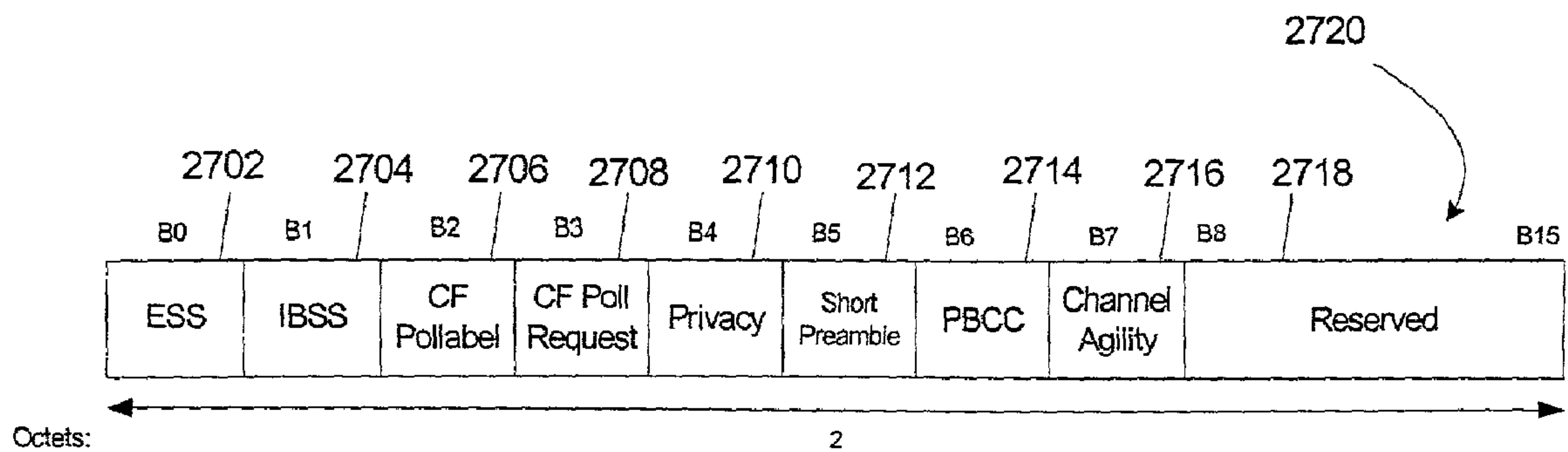
Figure 27A (Capability Information Fixed Field)
