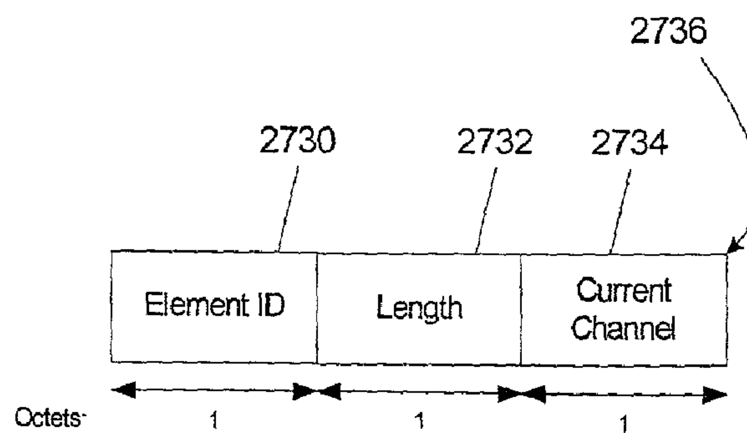
Figure 27C (DS Parameter Set Information Element Format)
