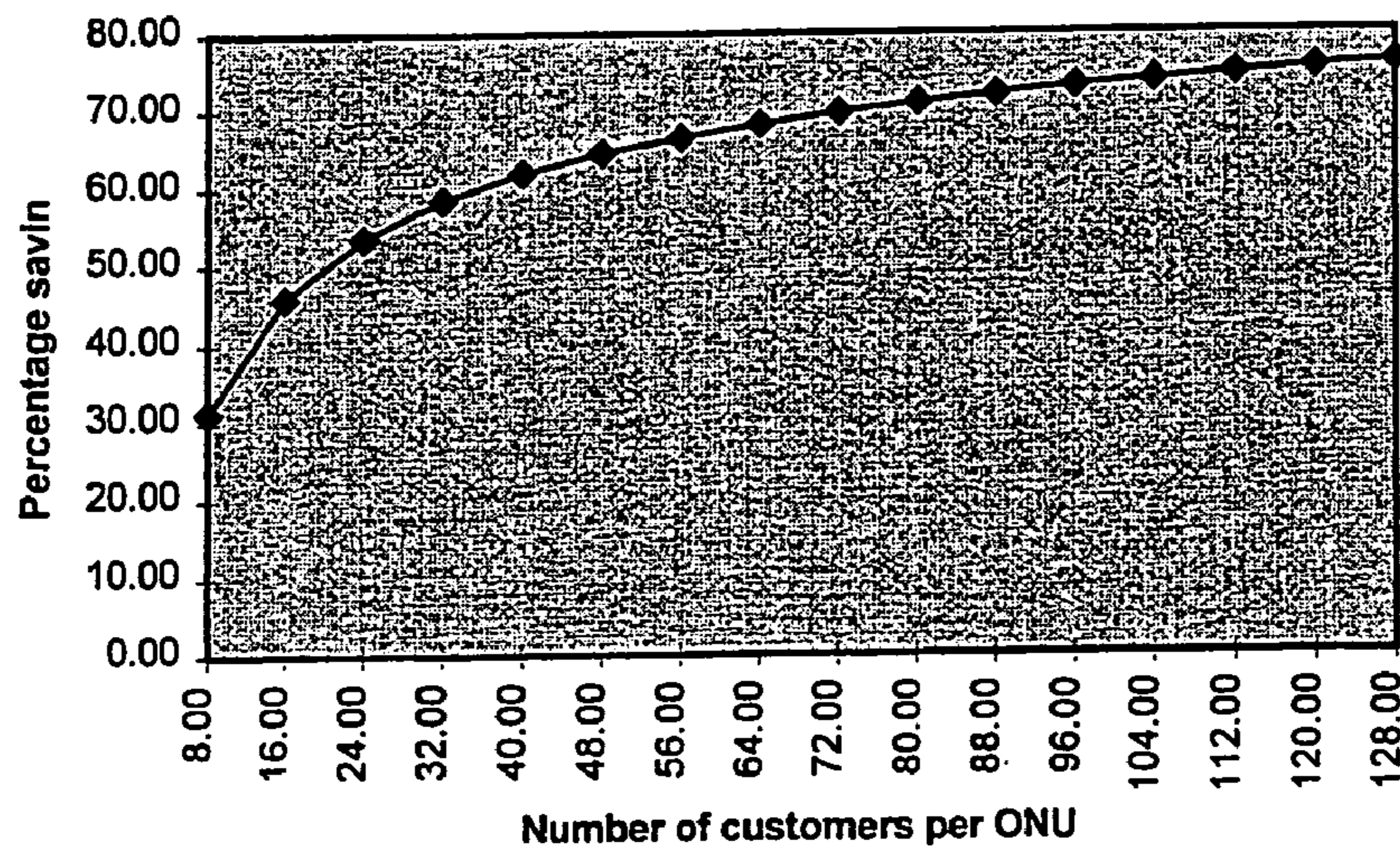
Percentage bandwidth saving against number of customers per ONU
