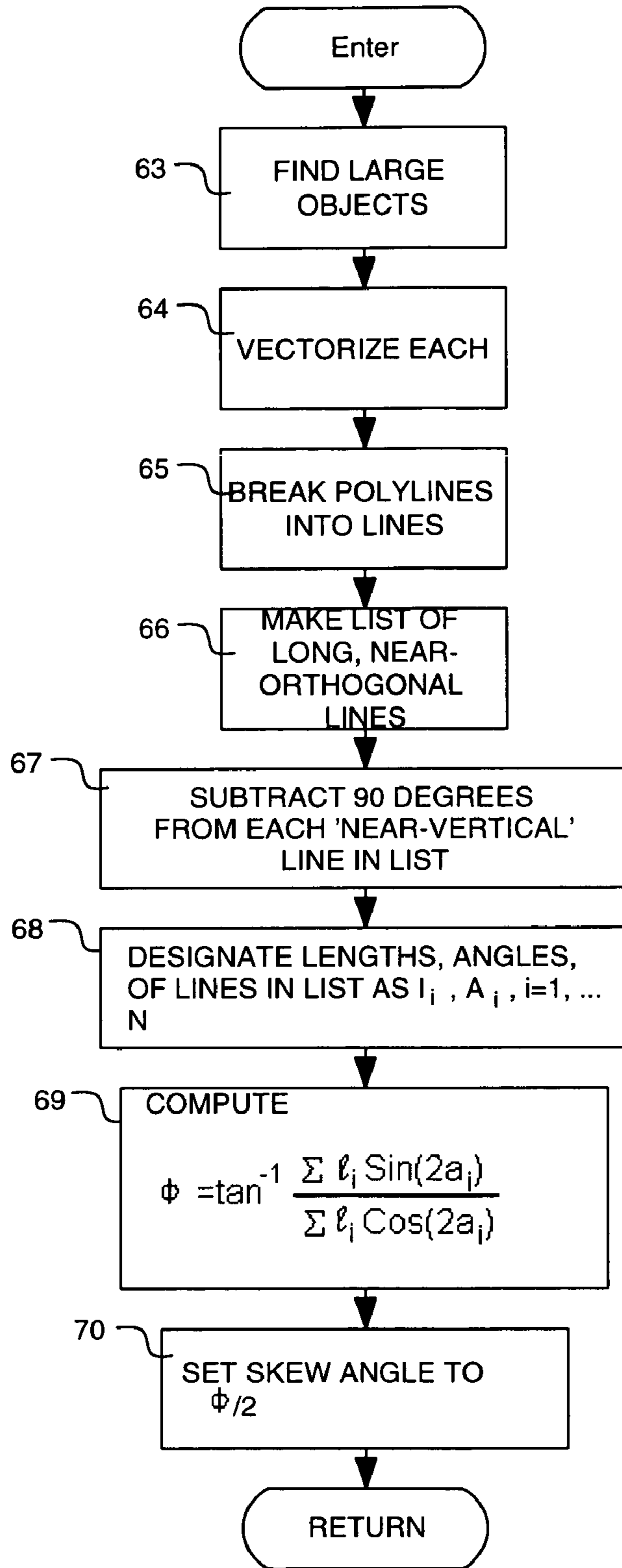
FIND SKEW ANGLE (GEOMETRIC)
