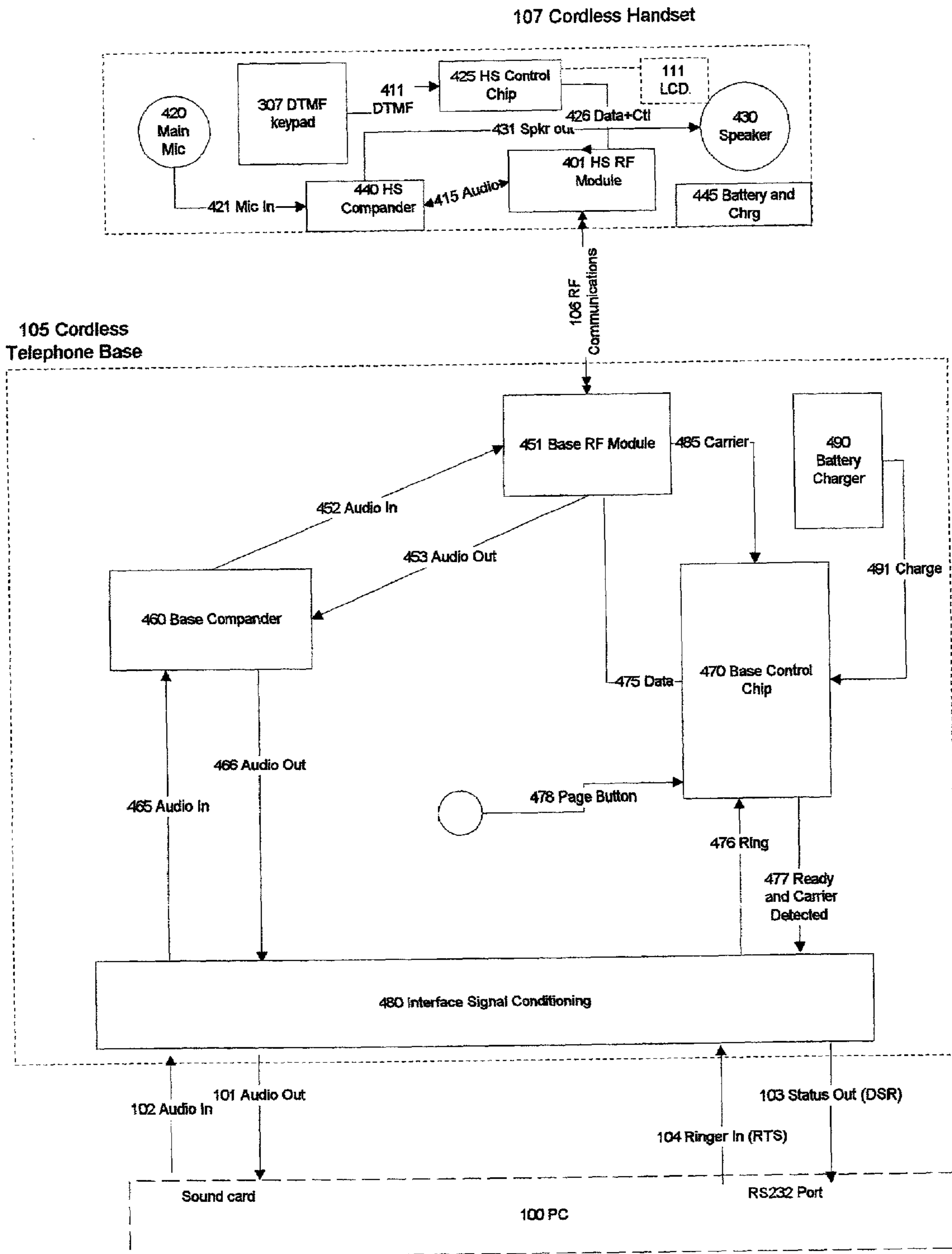
Figure 4 Simplified Block Diagram
