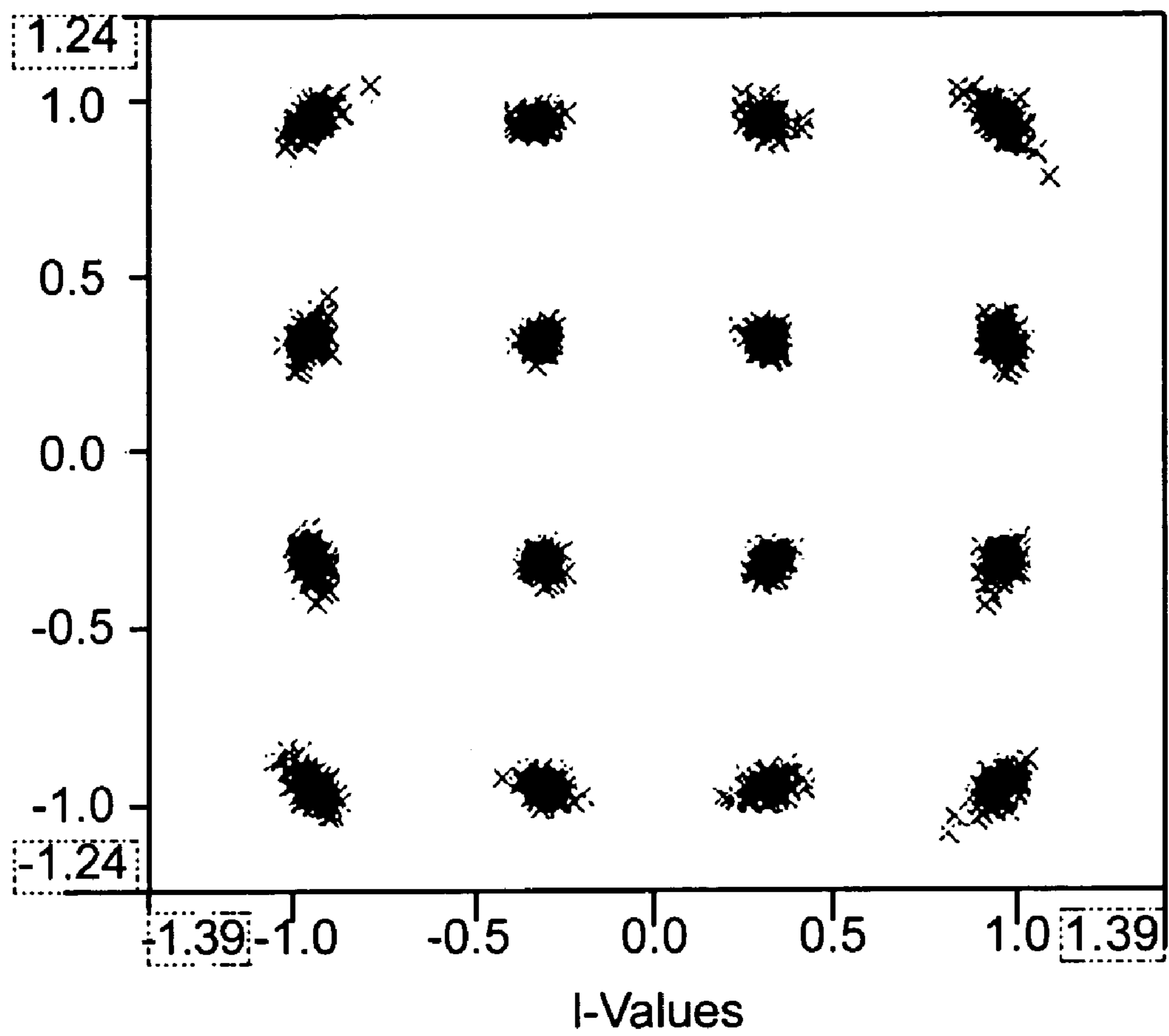
Received 16QAM Signal after amplitude correction Q-Values
