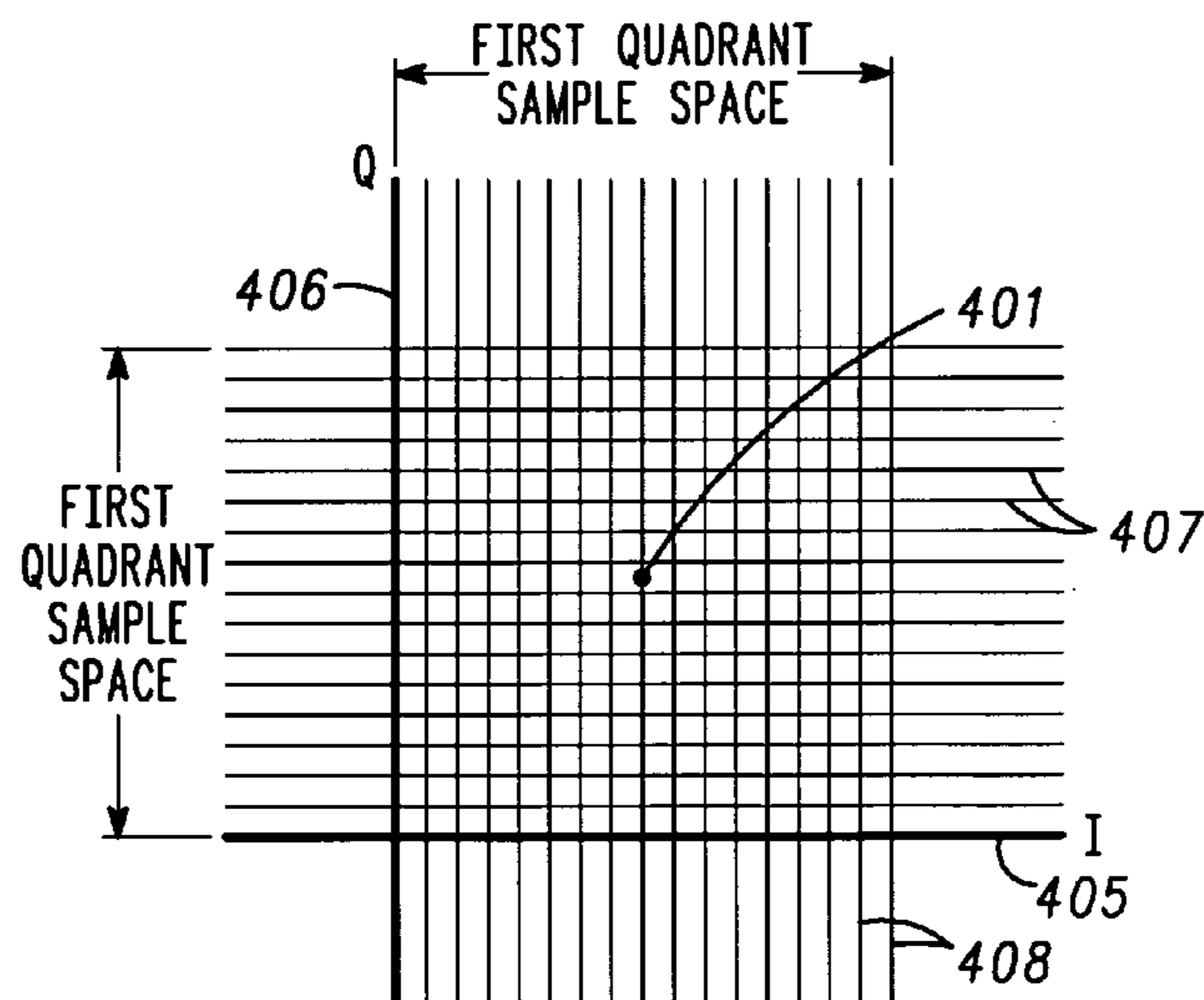
FIG. 4 -PRIOR ART-
