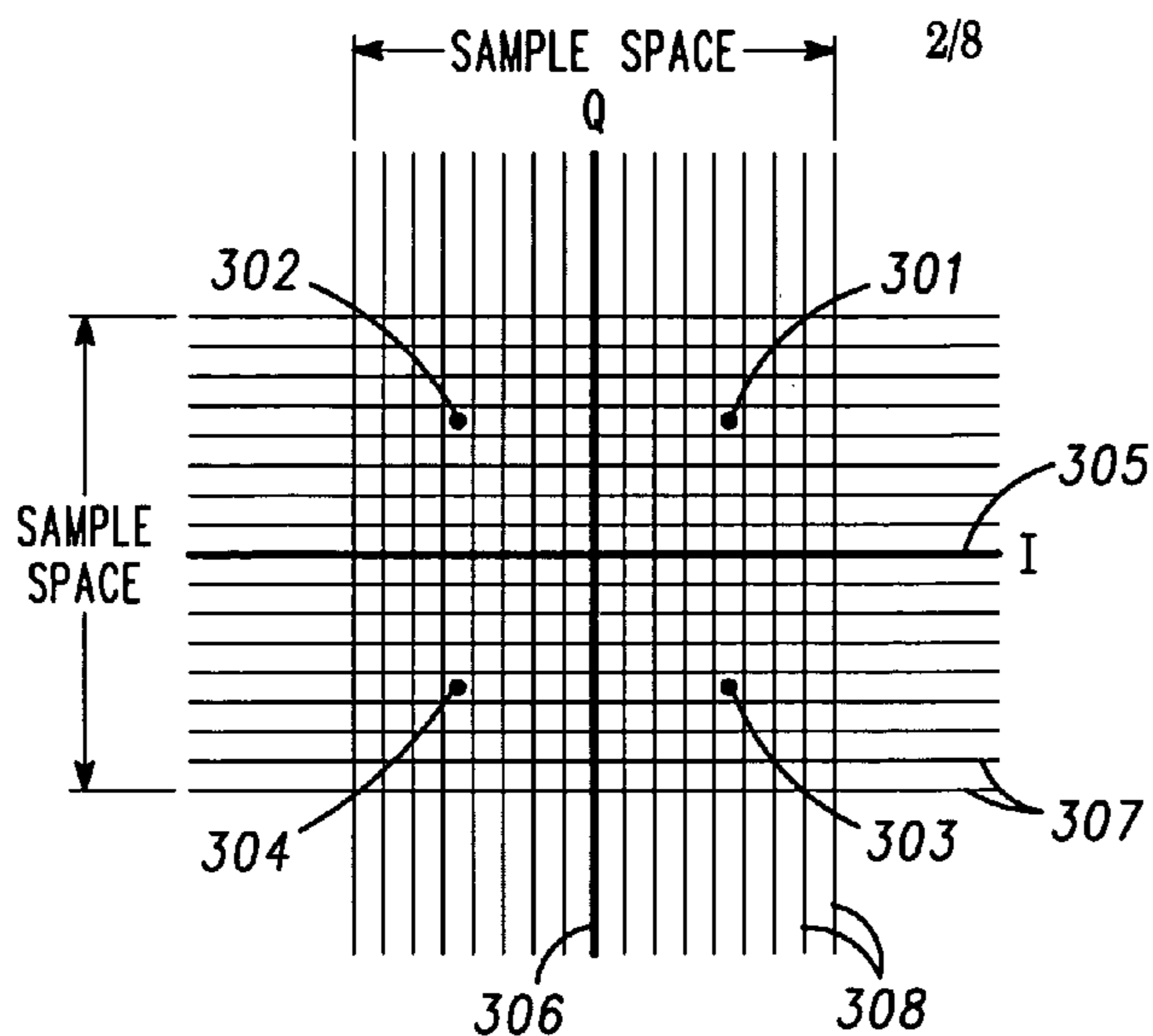
FIG. 3 -PRIOR ART-
