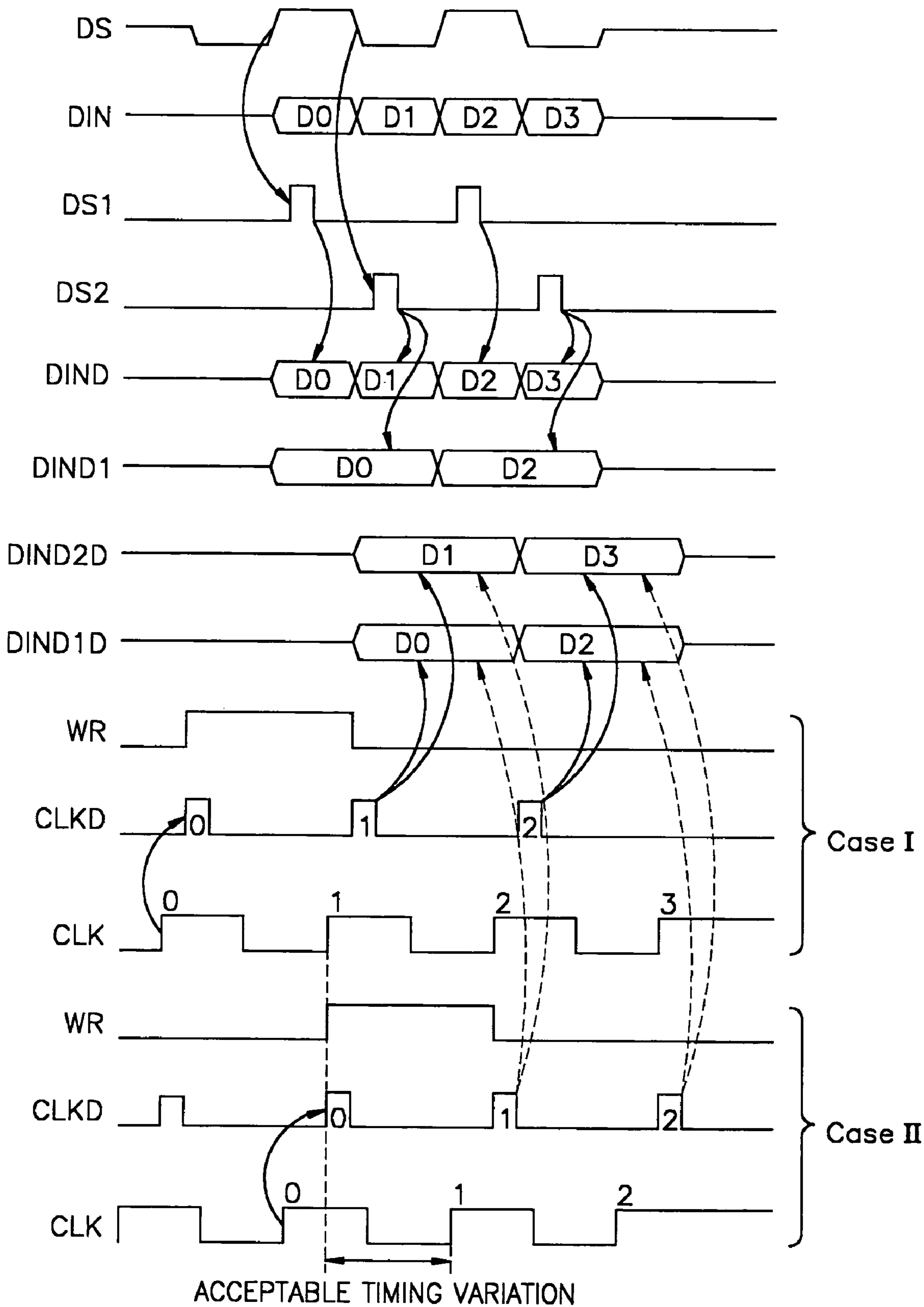
FIG. 2 (PRIOR ART)
