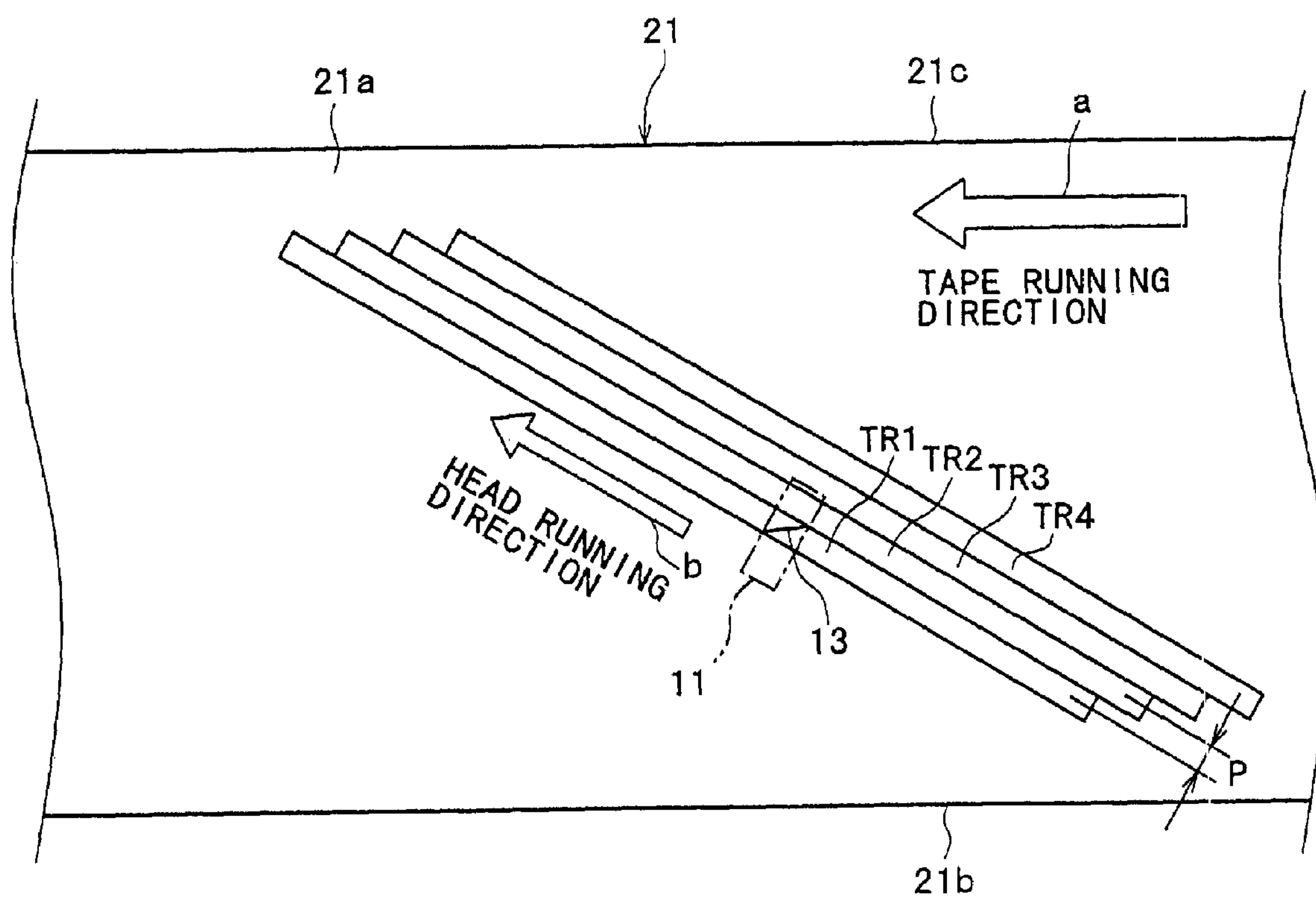
FIG. 16 (PRIOR ART)
