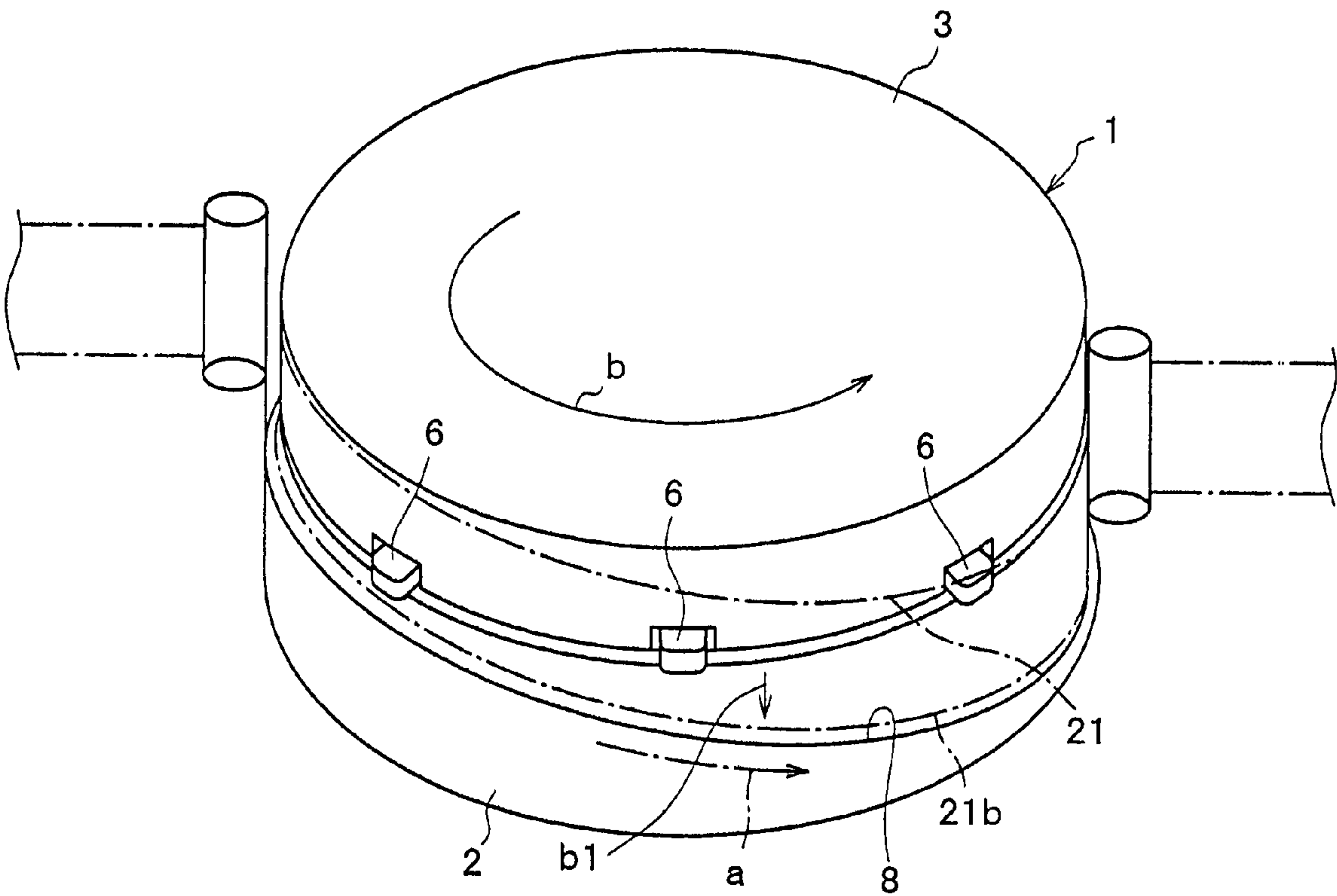
FIG. 12 (PRIOR ART)
