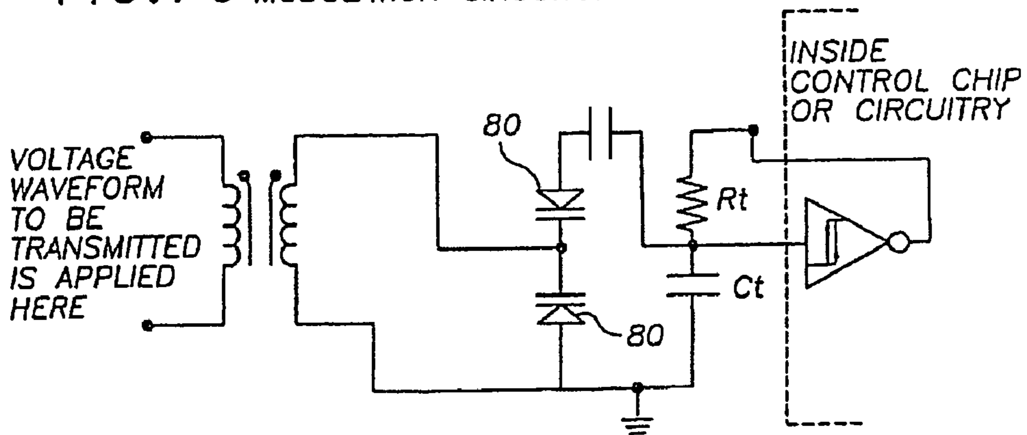
FIG. 7c MODULATION CIRCUITS.
