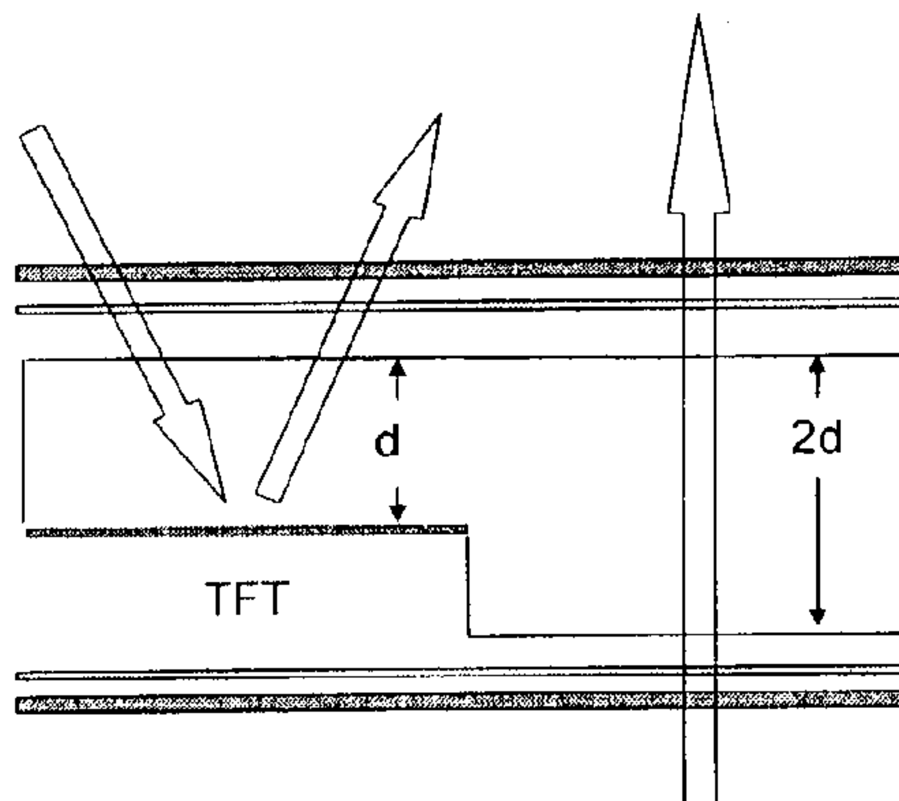
Fig. 1b Double Cell Gap (PRIOR ART)
