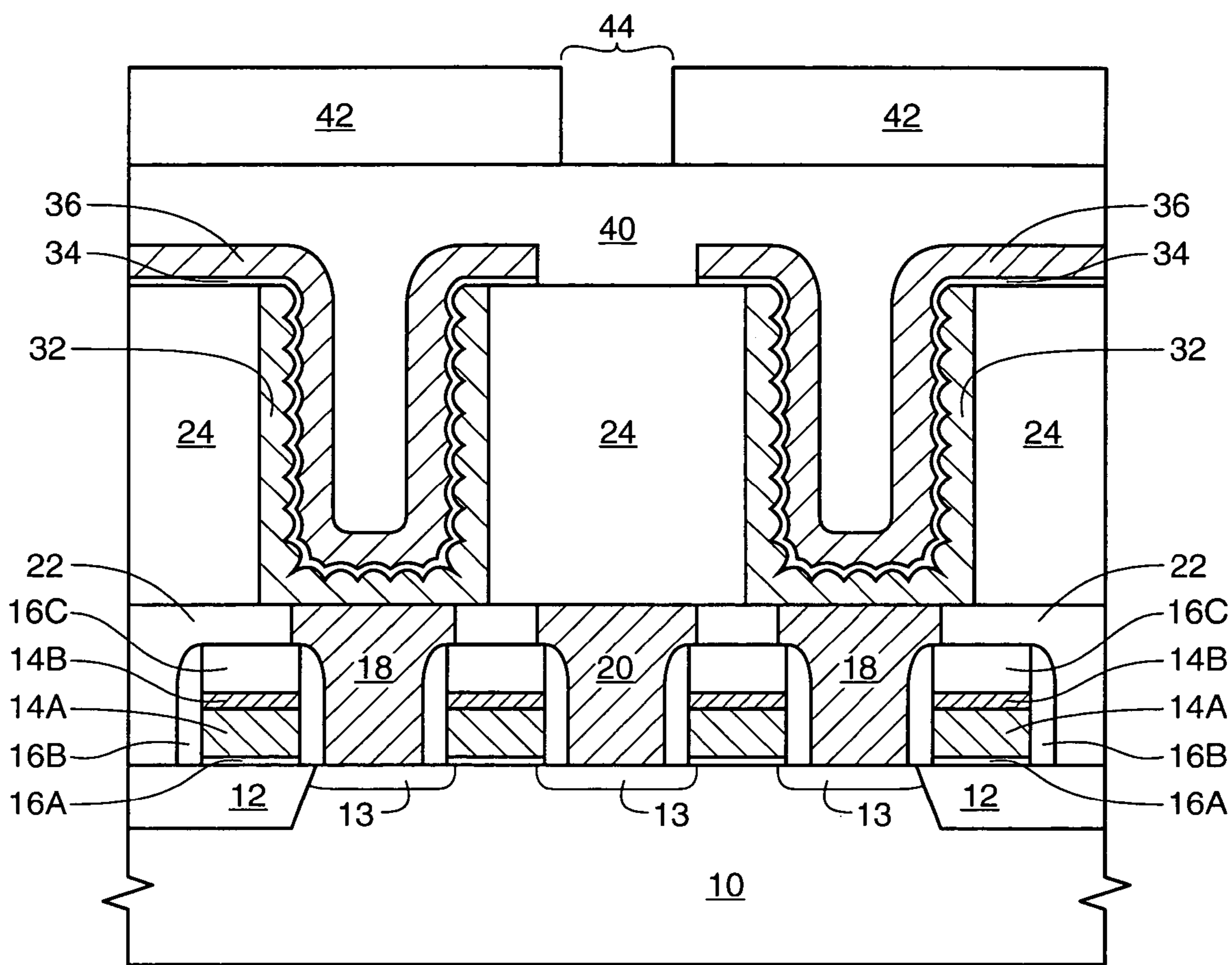
FIG. 4 (RELATED ART)
