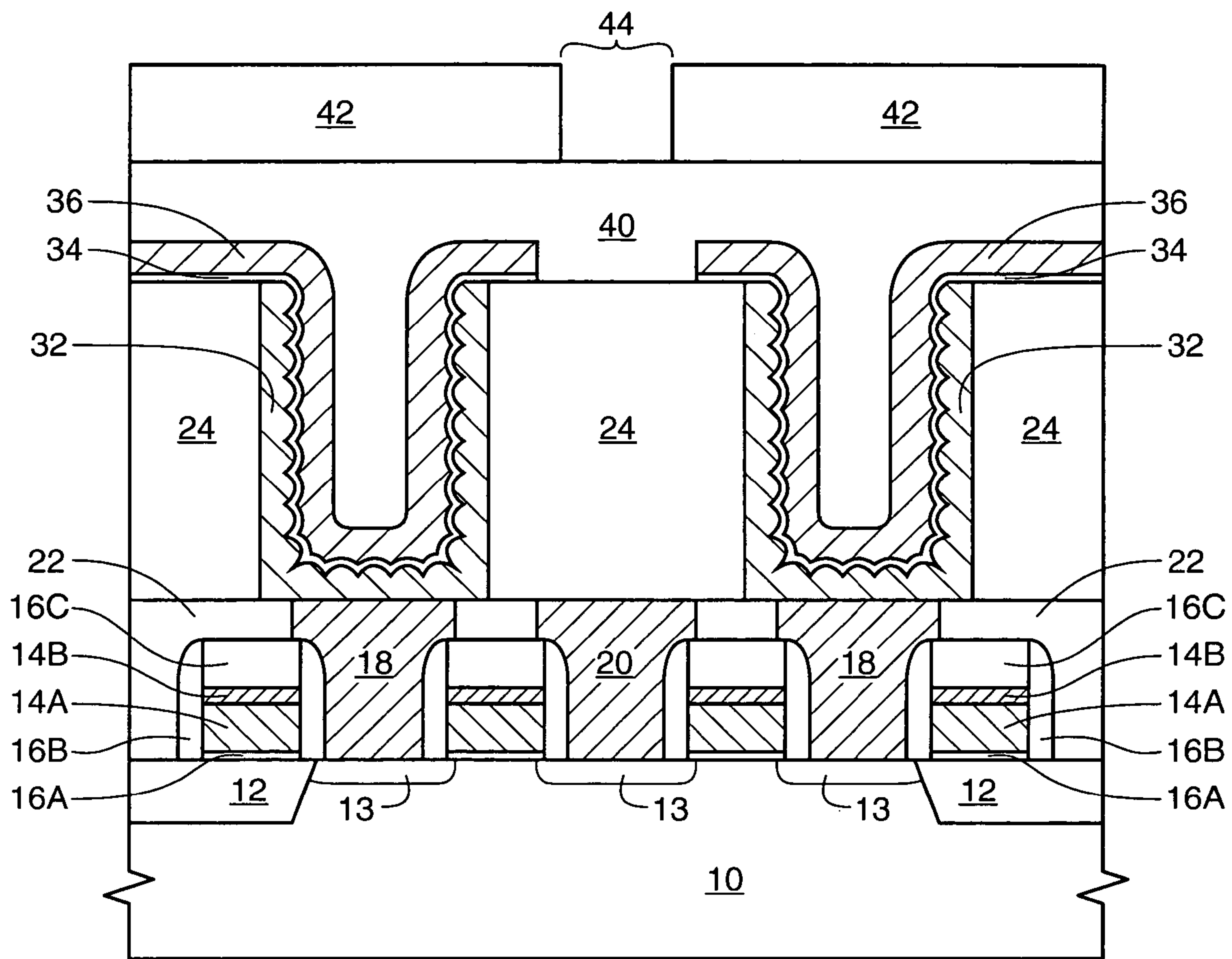
FIG. 4 (RELATED ART)
