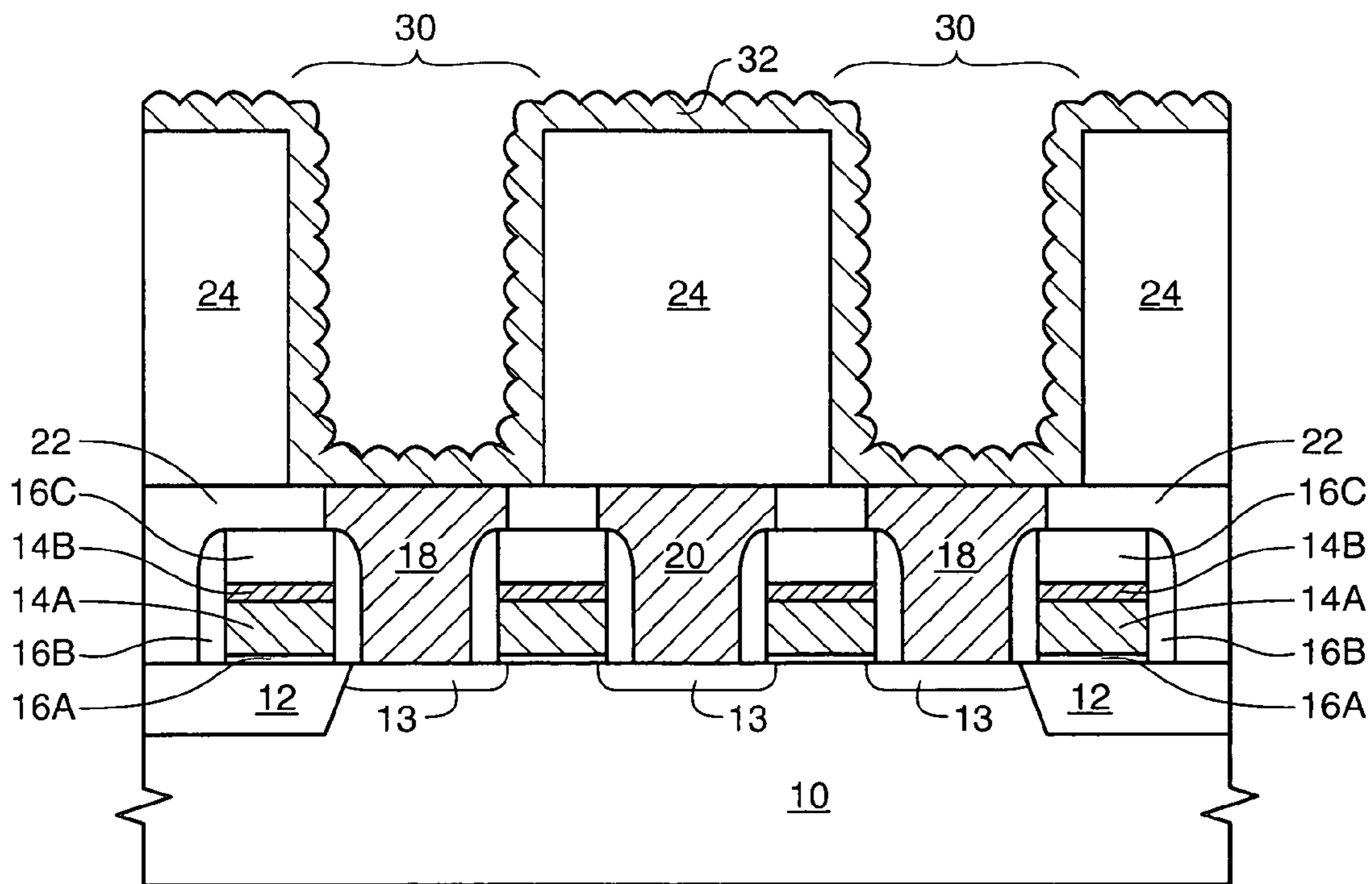
FIG. 2 (RELATED ART)
