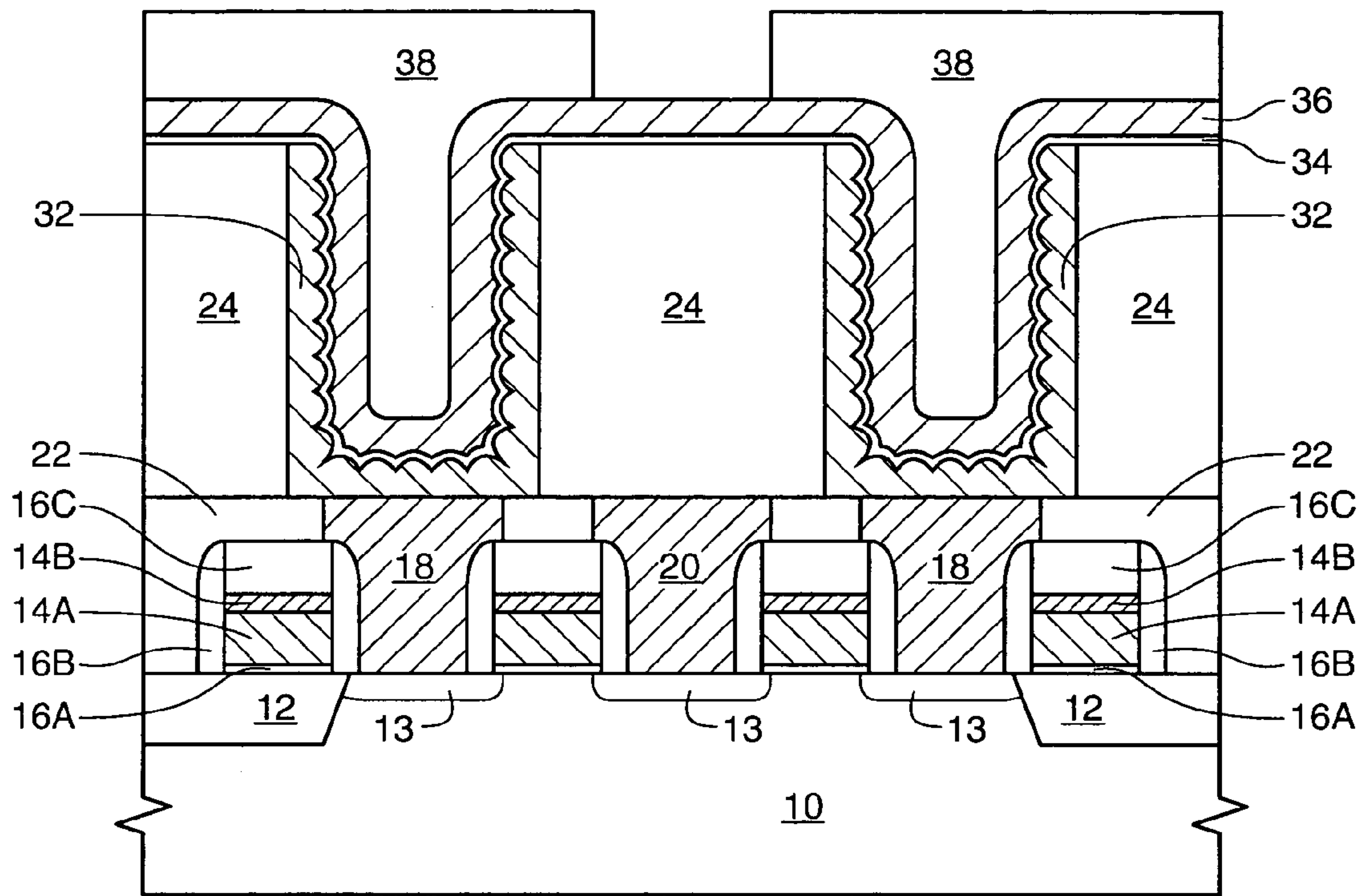
FIG. 3 (RELATED ART)
