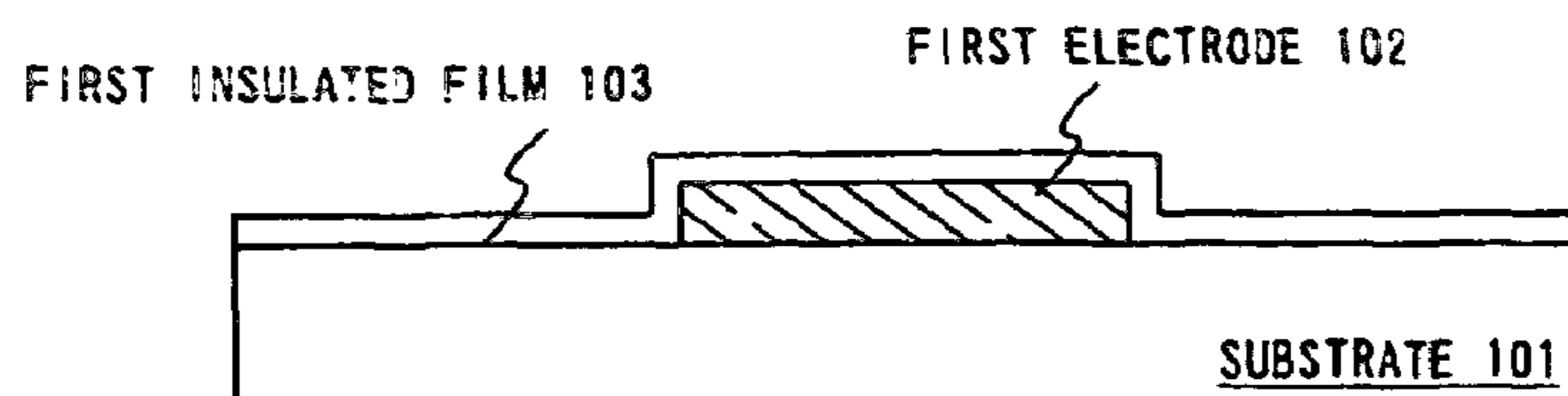
Fig. 2A FORMATION OF GATE ELECTRODE AND GATE INSULATING FILM
