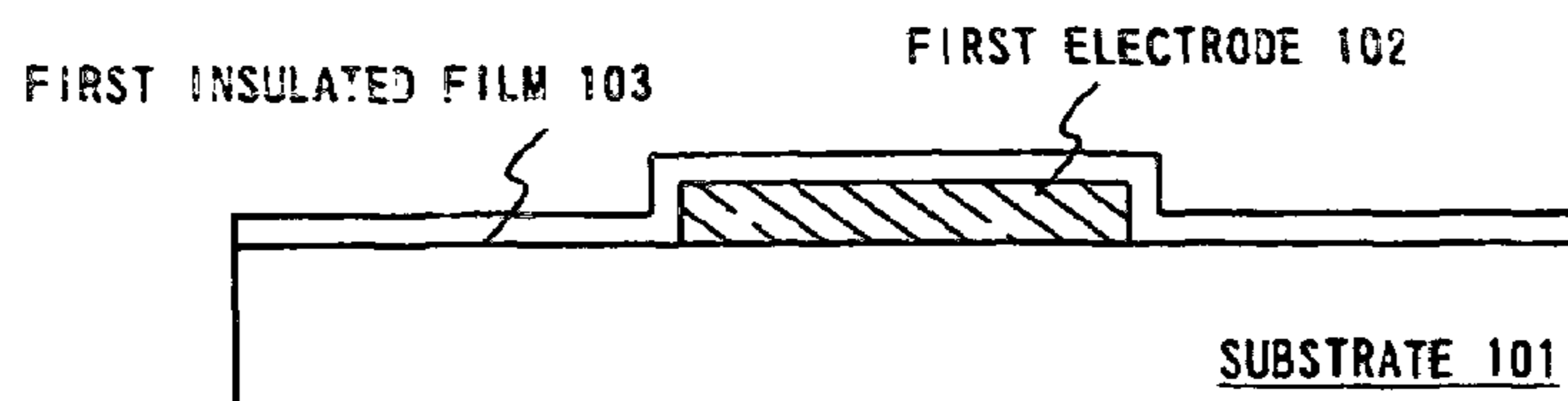
Fig. 2A FORMATION OF GATE ELECTRODE AND GATE INSULATING FILM
