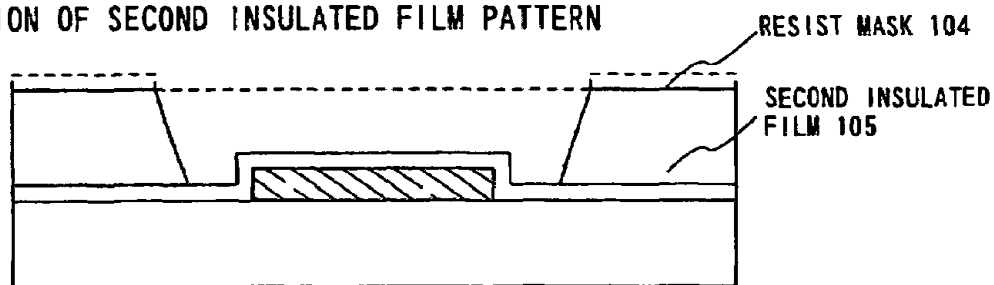
Fig. 2C FORMATION OF SECOND INSULATED FILM PATTERN
