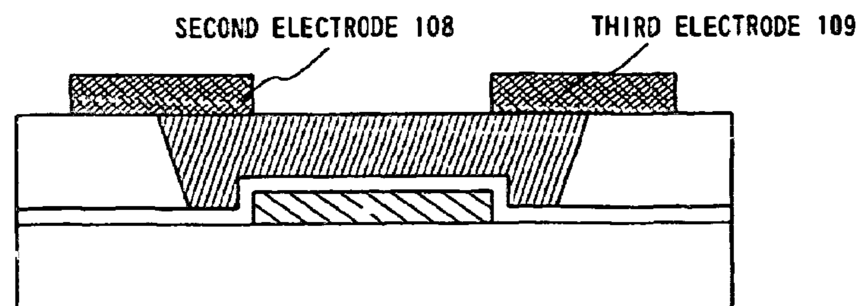
Fig. 2E FORMATION OF SECOND ELECTRODE AND THIRD ELECTRODE
