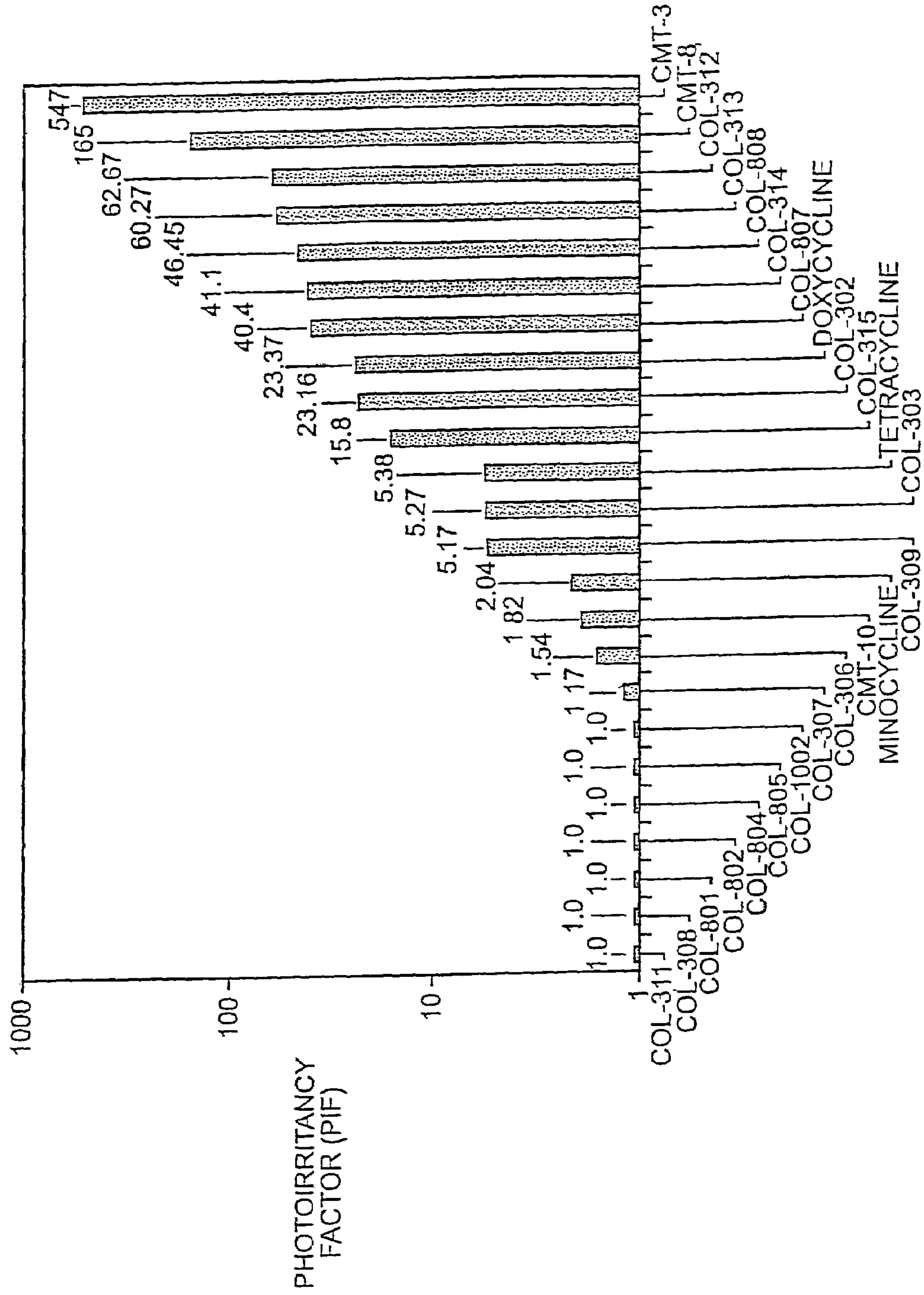
FIG. 1 PHOTOTOXICITY INDEX
