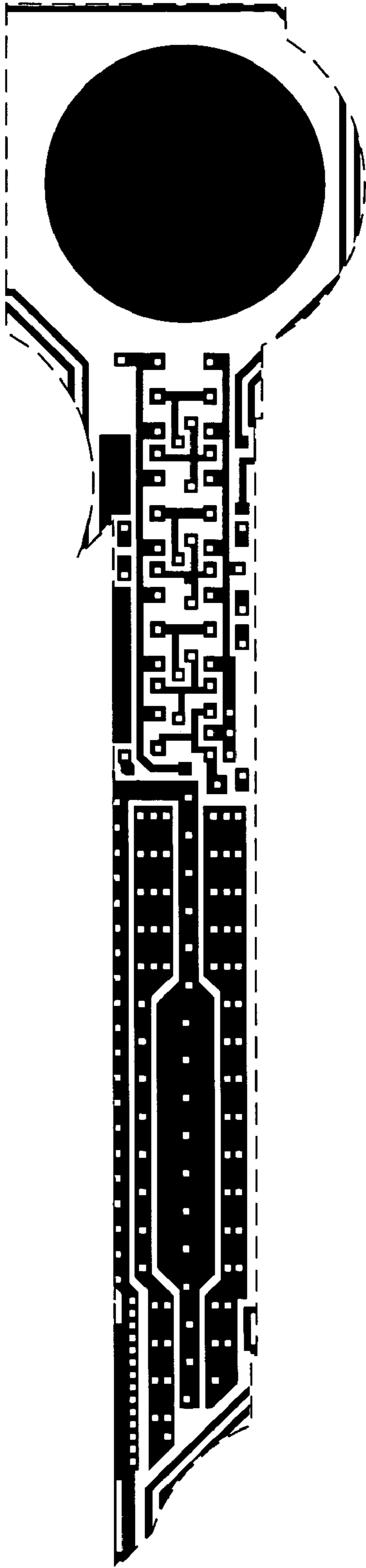
Metal 1 mask
