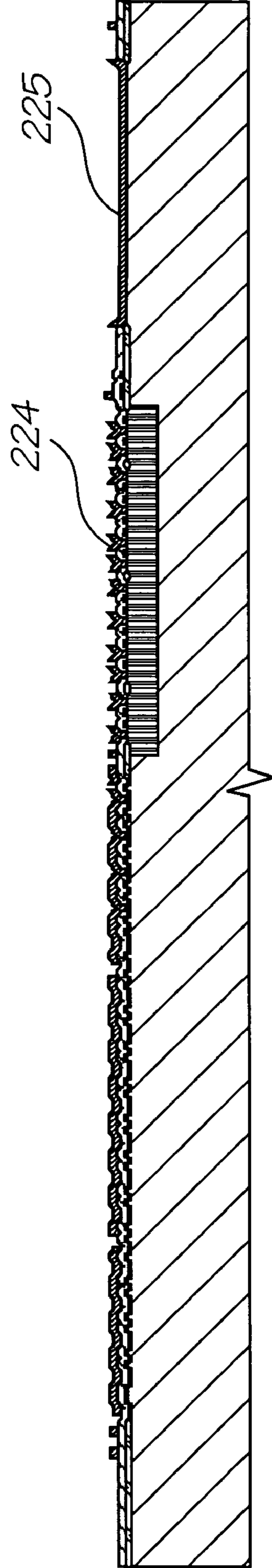
Deposit Metal 1
