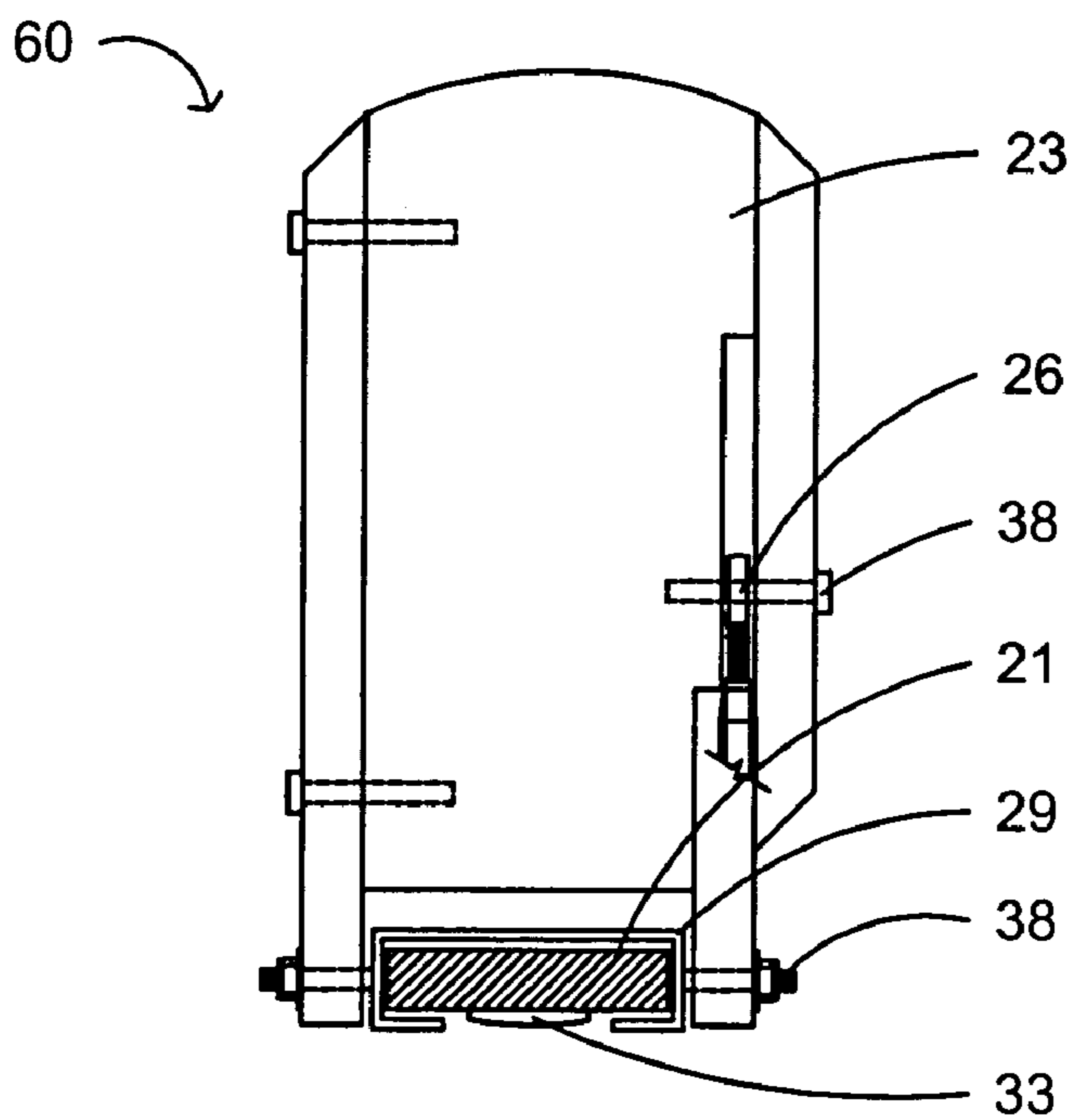
Foot Paddle - Front View
