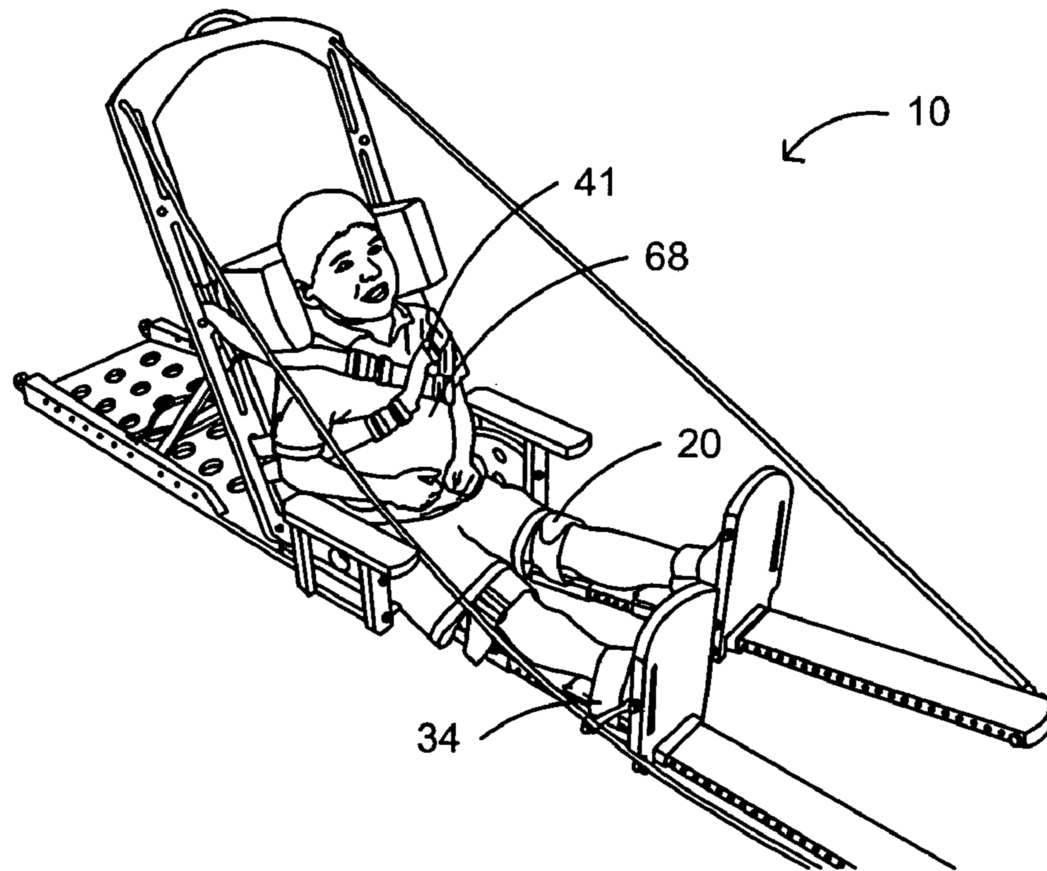
FIG. 19 Stretching Demonstration
