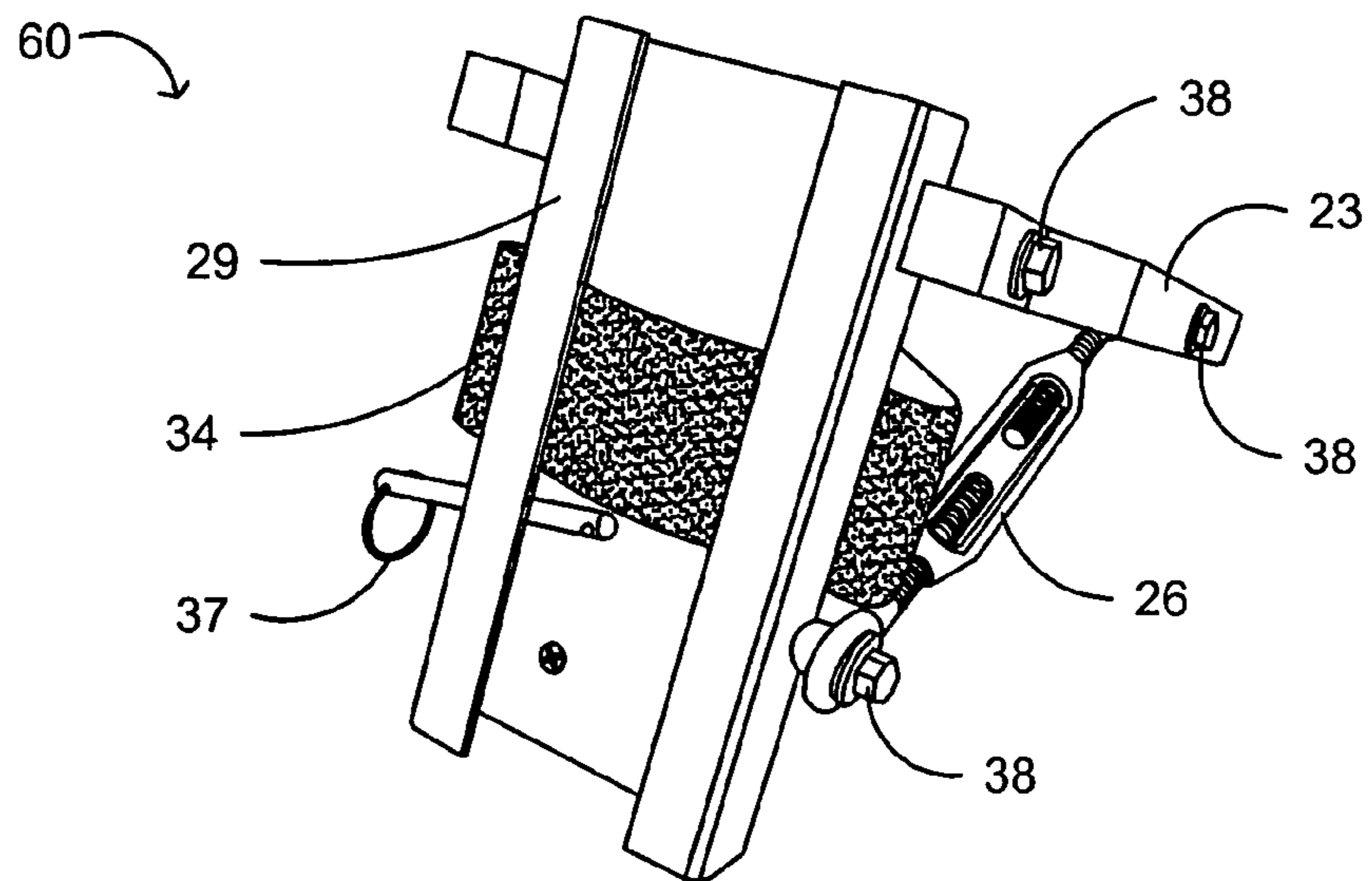
FIG. 11 Bottom View
