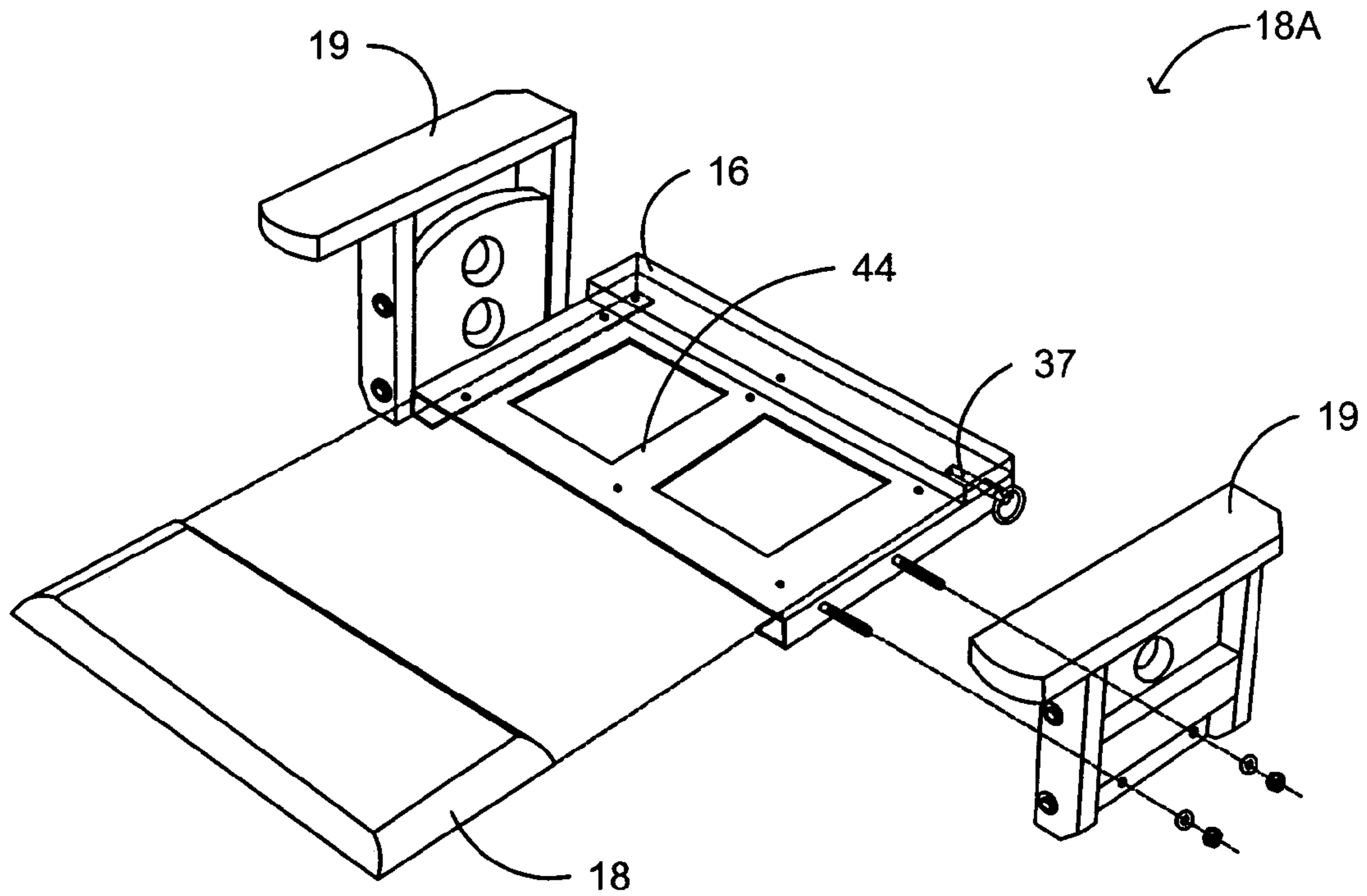
Sliding Seat Rail
