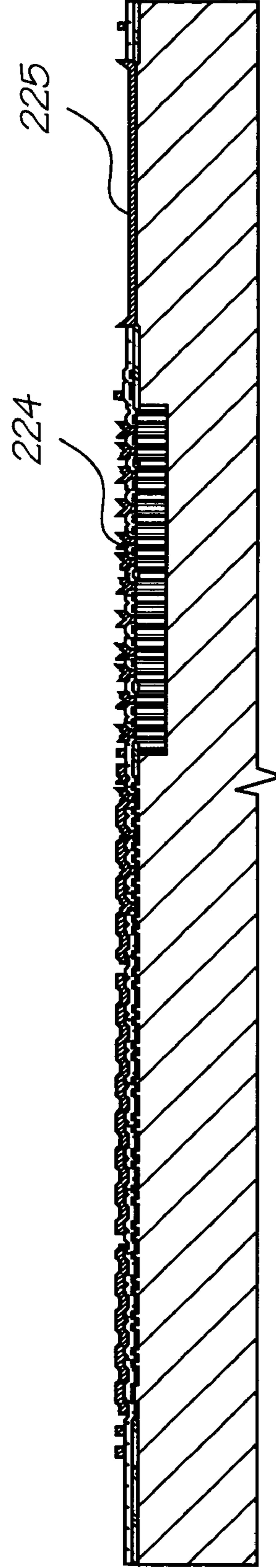
Deposit Metal 1
