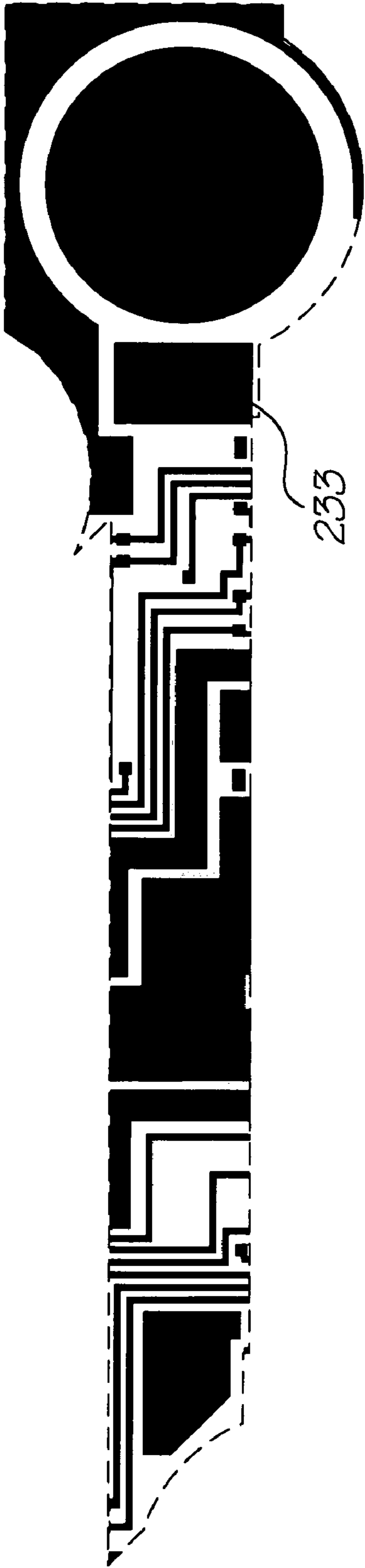
Metal 2 mask
