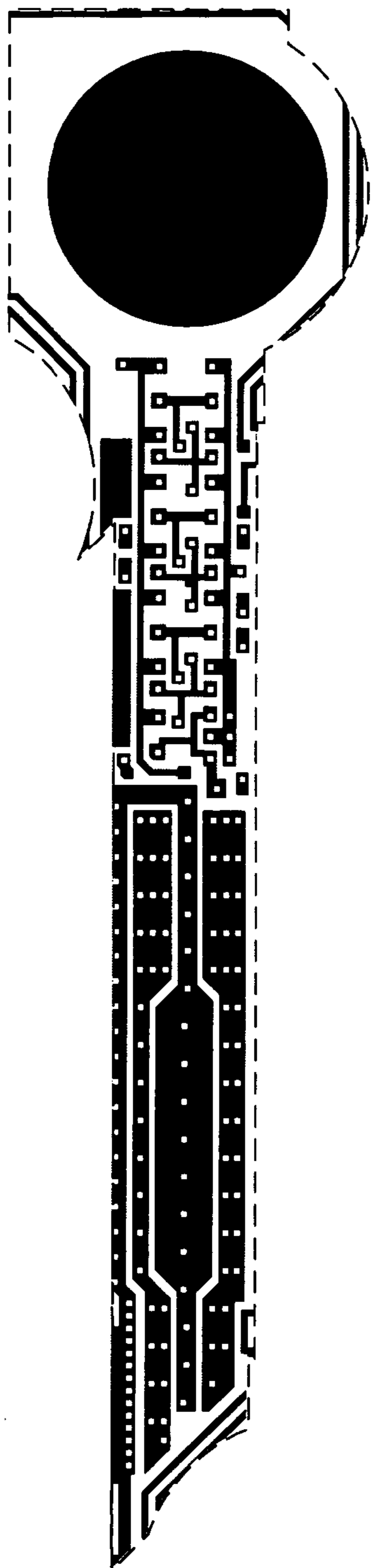
Metal 1 mask
