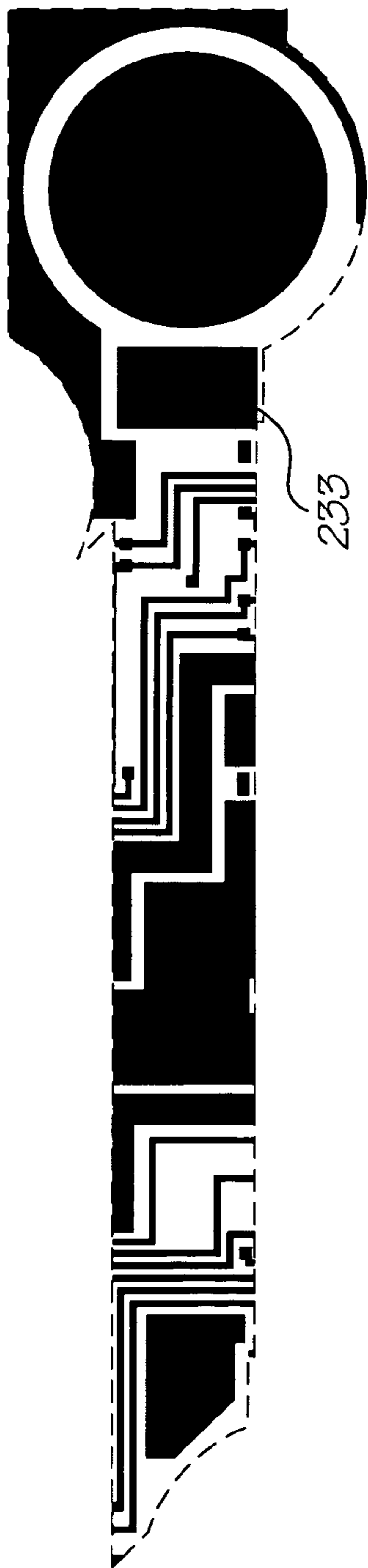
Metal 2 mask
