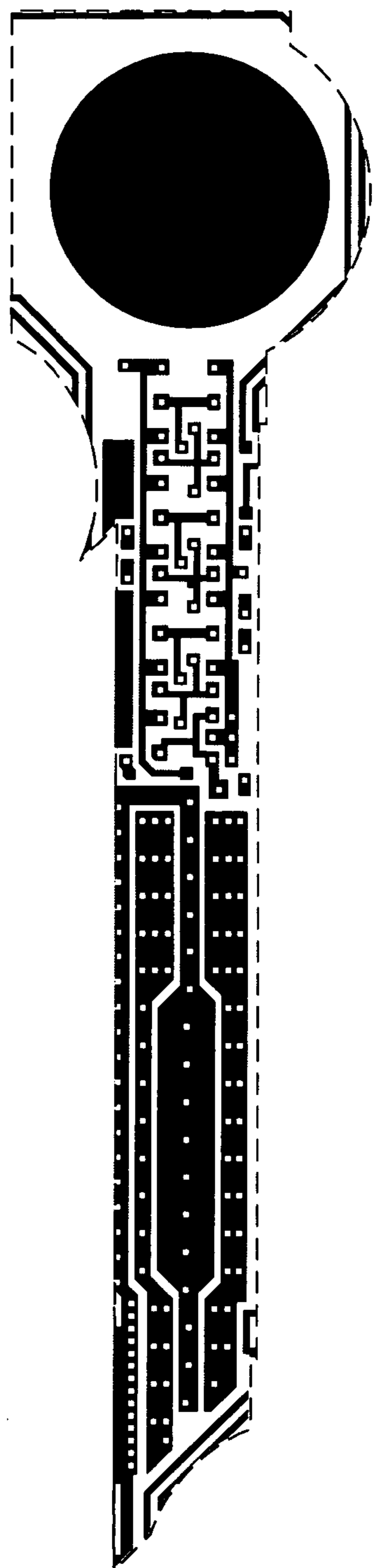
Metal 1 mask
