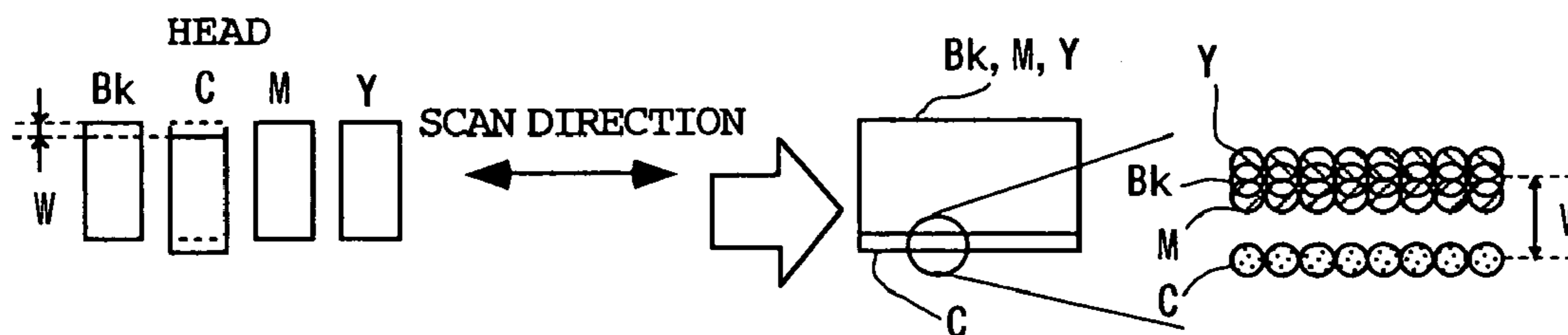
FIG. 14 (b) VERTICAL MOUNTING DEVIATION
