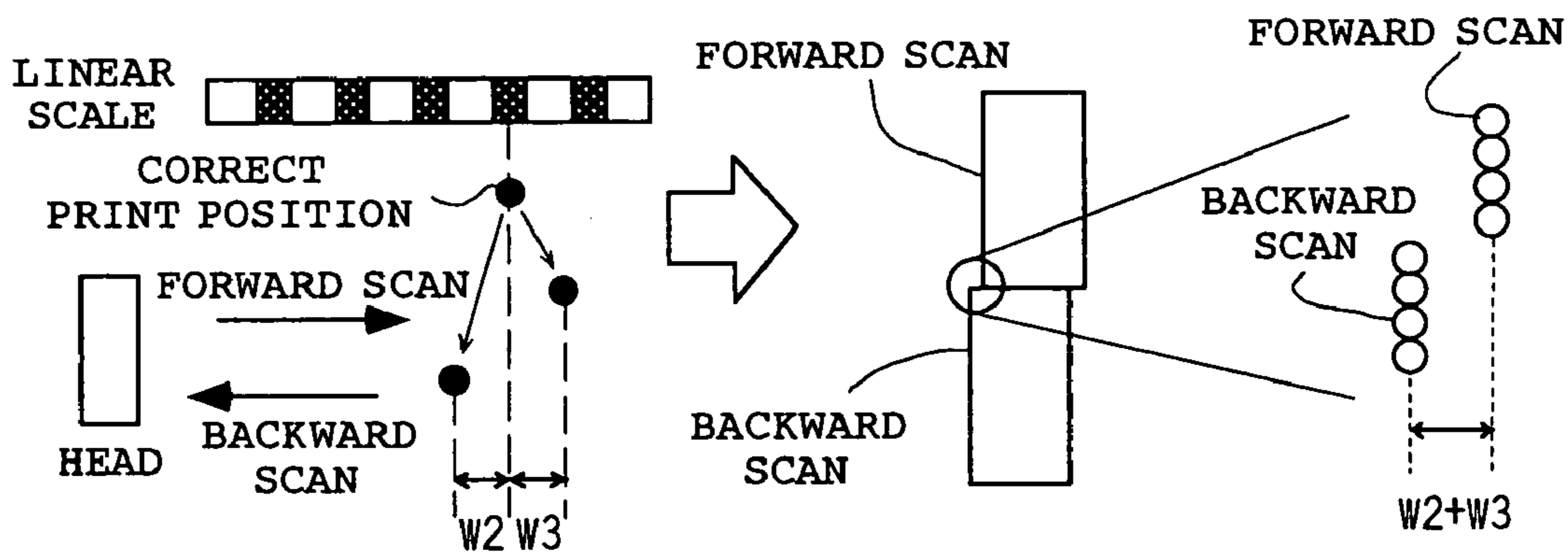
FIG. 14 (c) FORWARD/BACKWARD PRINT DEVIATION
