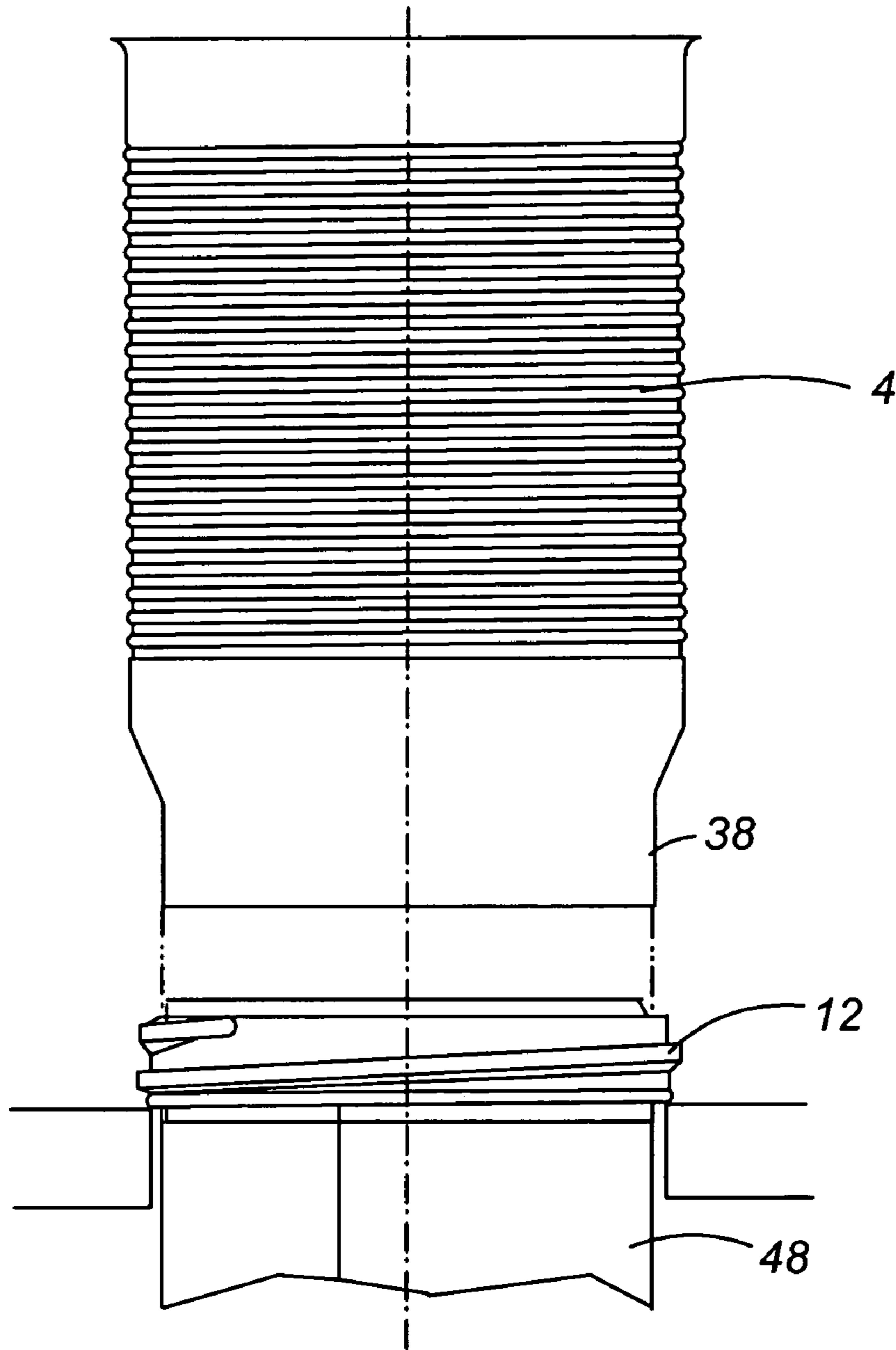
THREAD RING AND CAN ONTO EXPANDING MECHANISM
