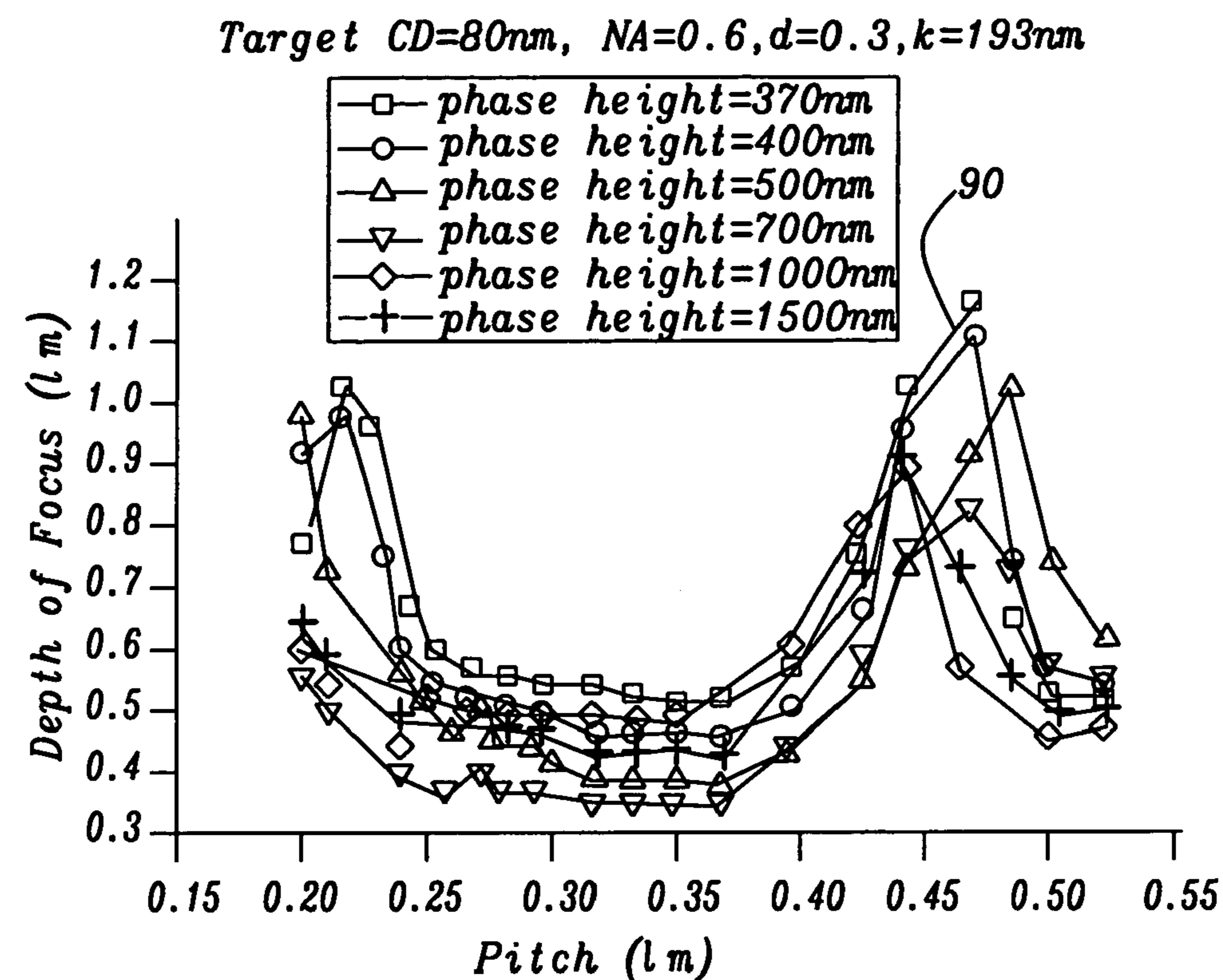
FIG. 9 – Prior Art
