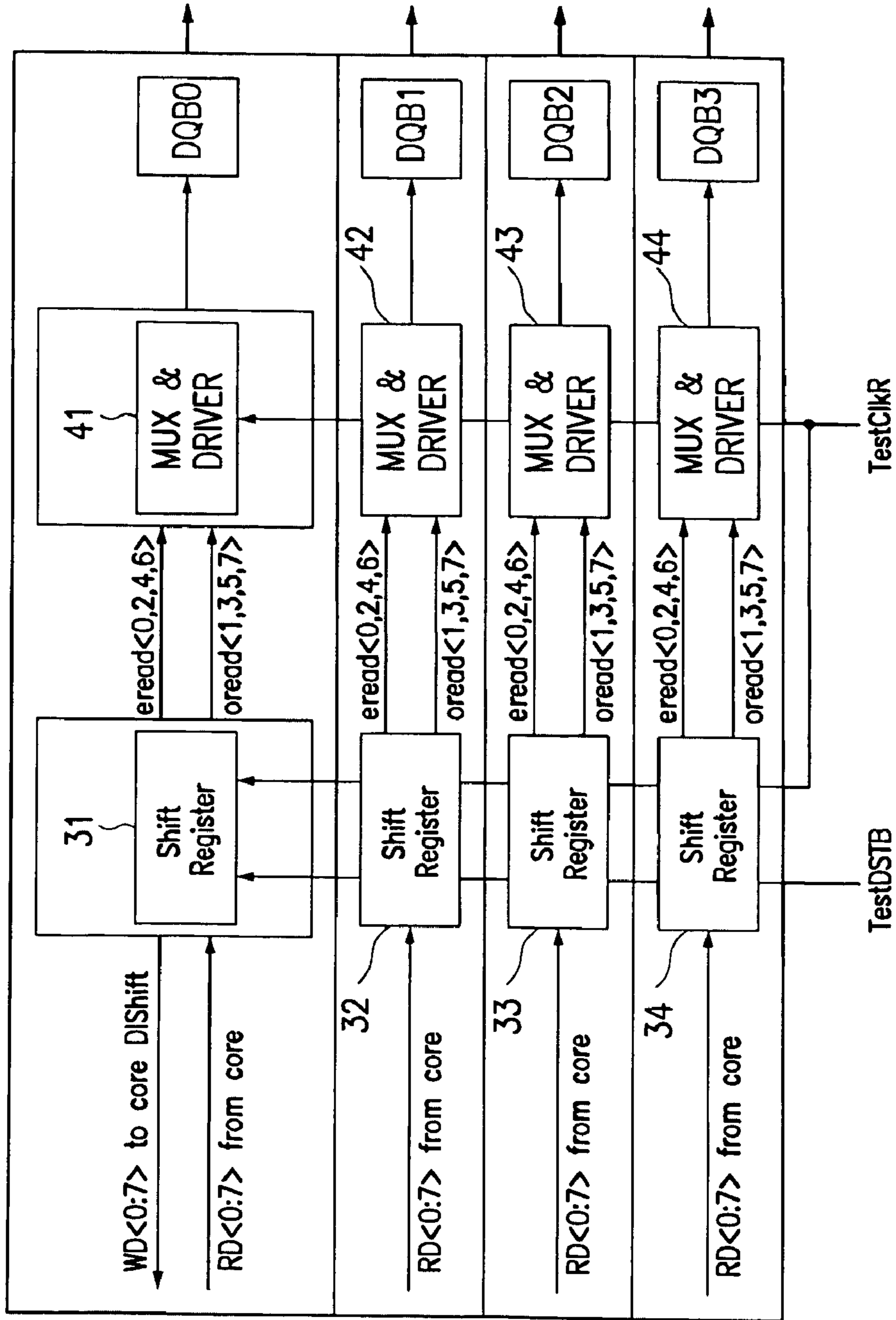
FIG. 2 (PRIOR ART)
