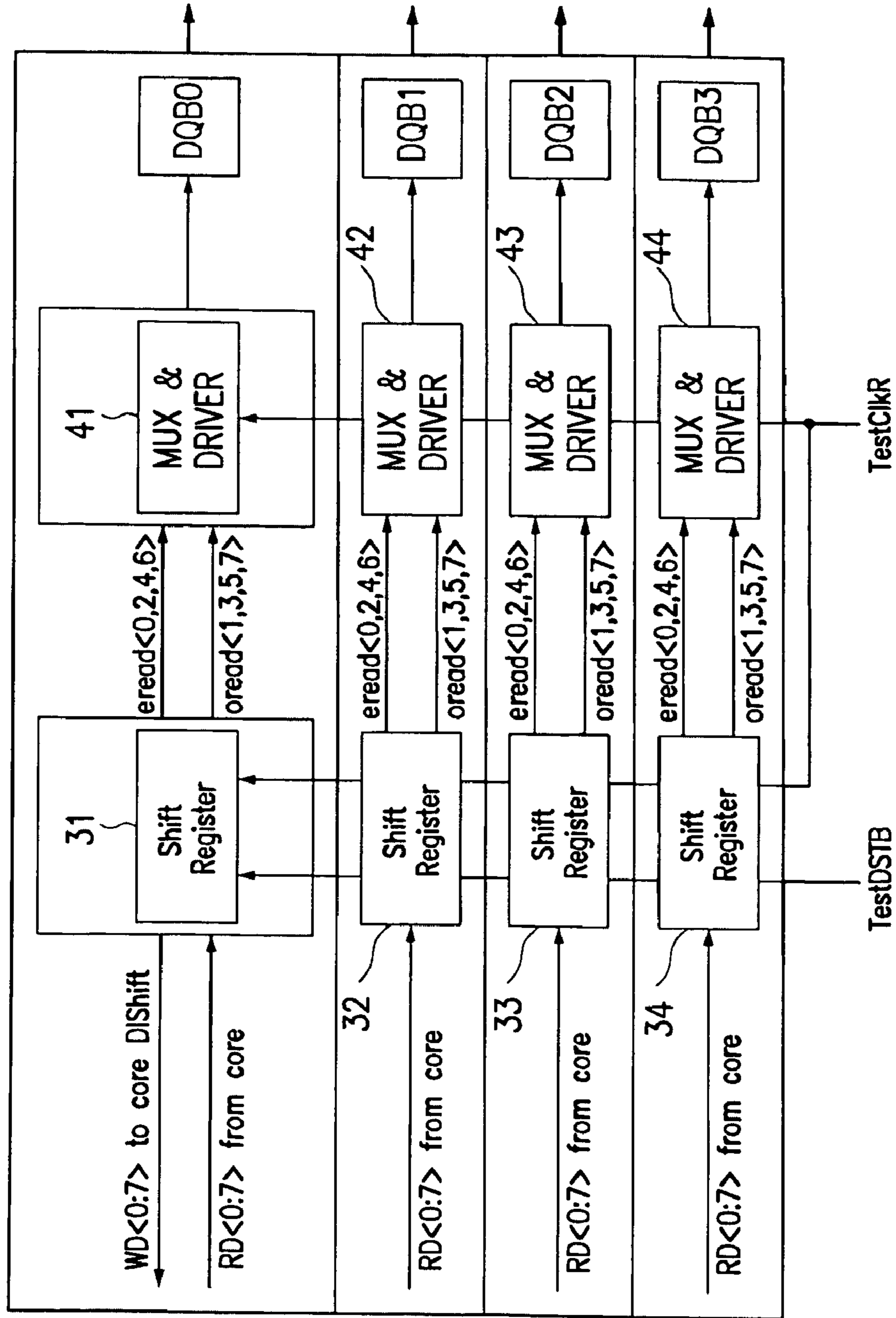
FIG. 2 (PRIOR ART)
