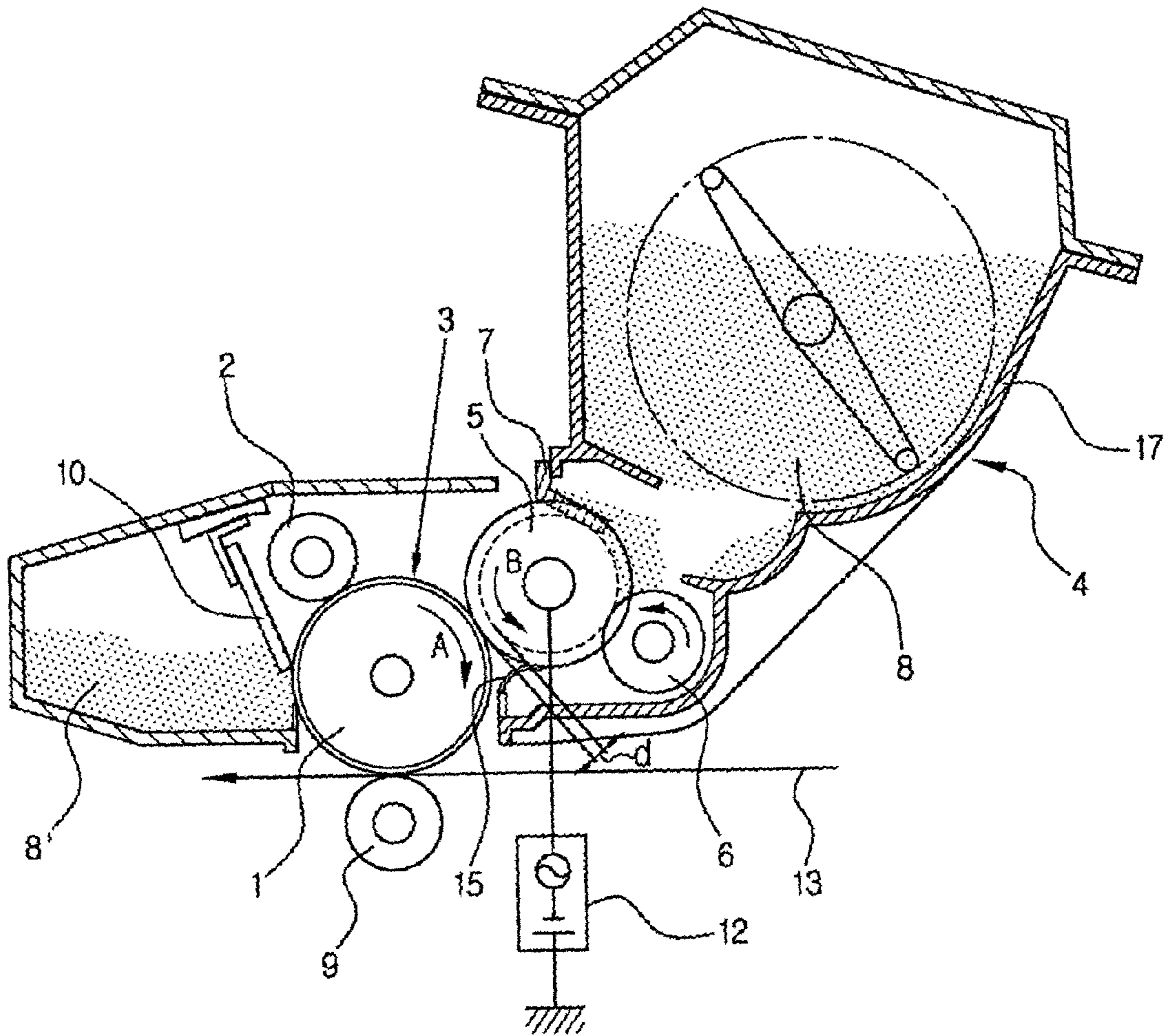
FIG. 1 (PRIOR ART)
