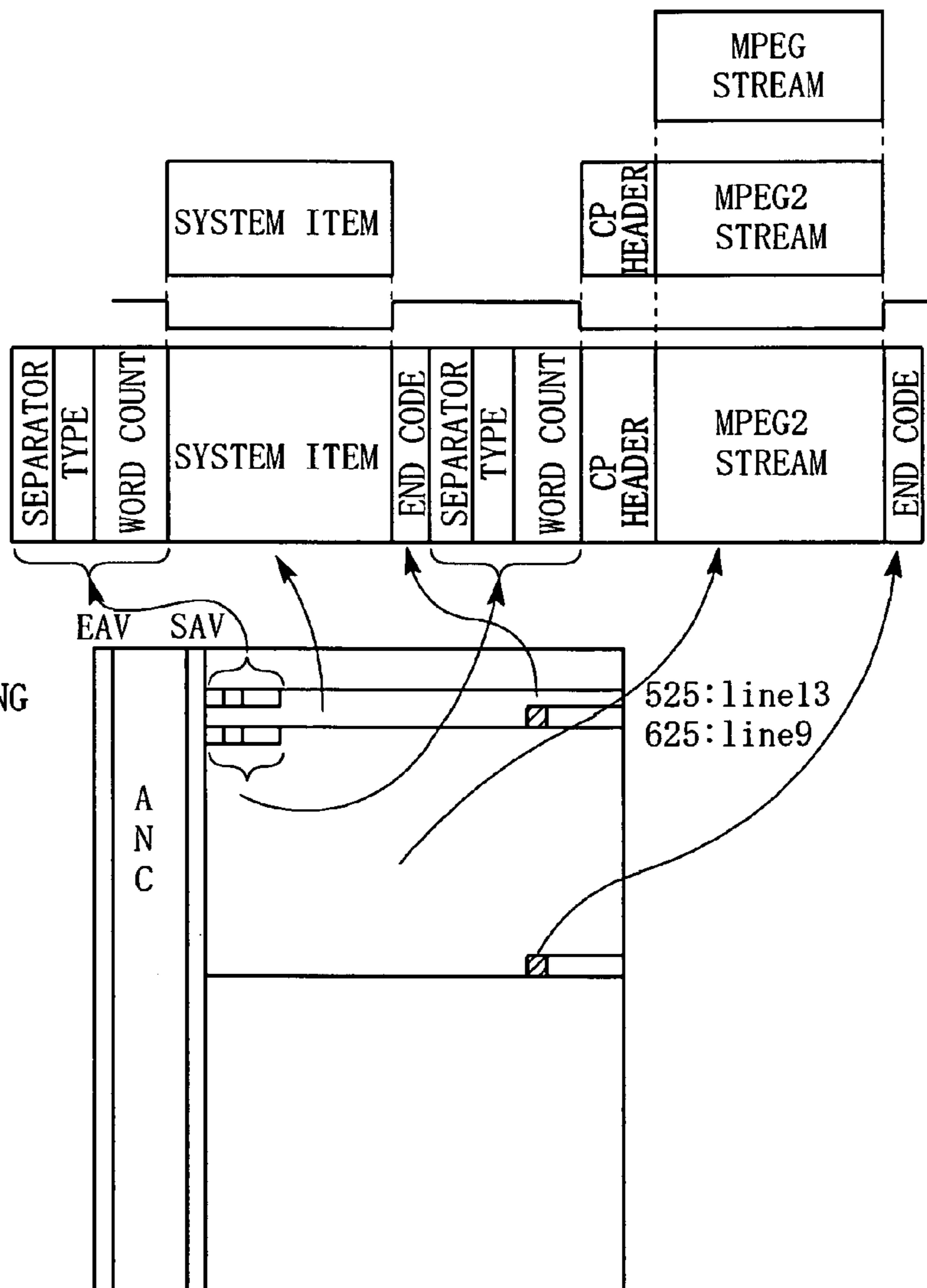
FIG. 31B SDTI-CP STREAM
