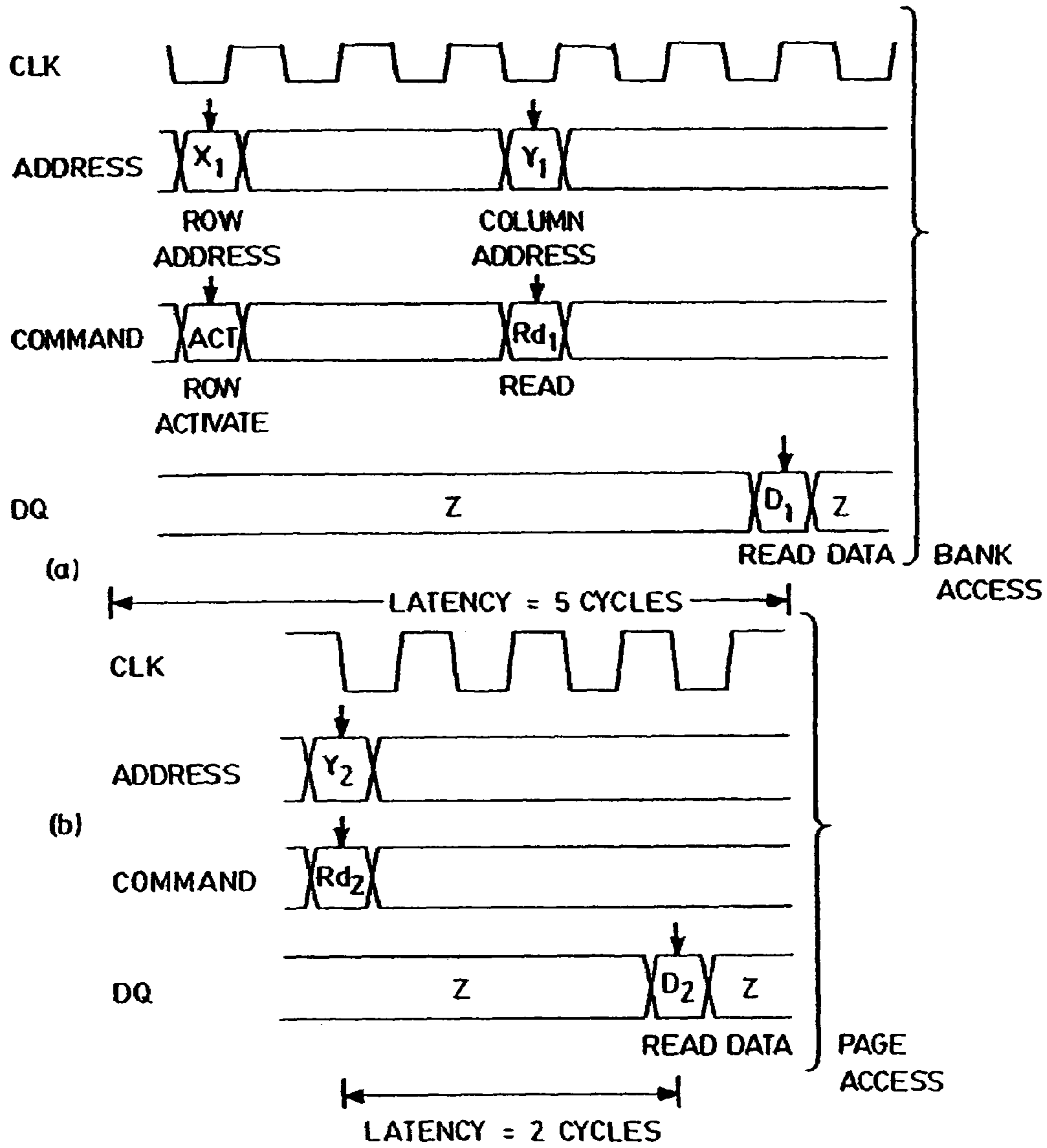
FIG. 1 PRIOR ART
