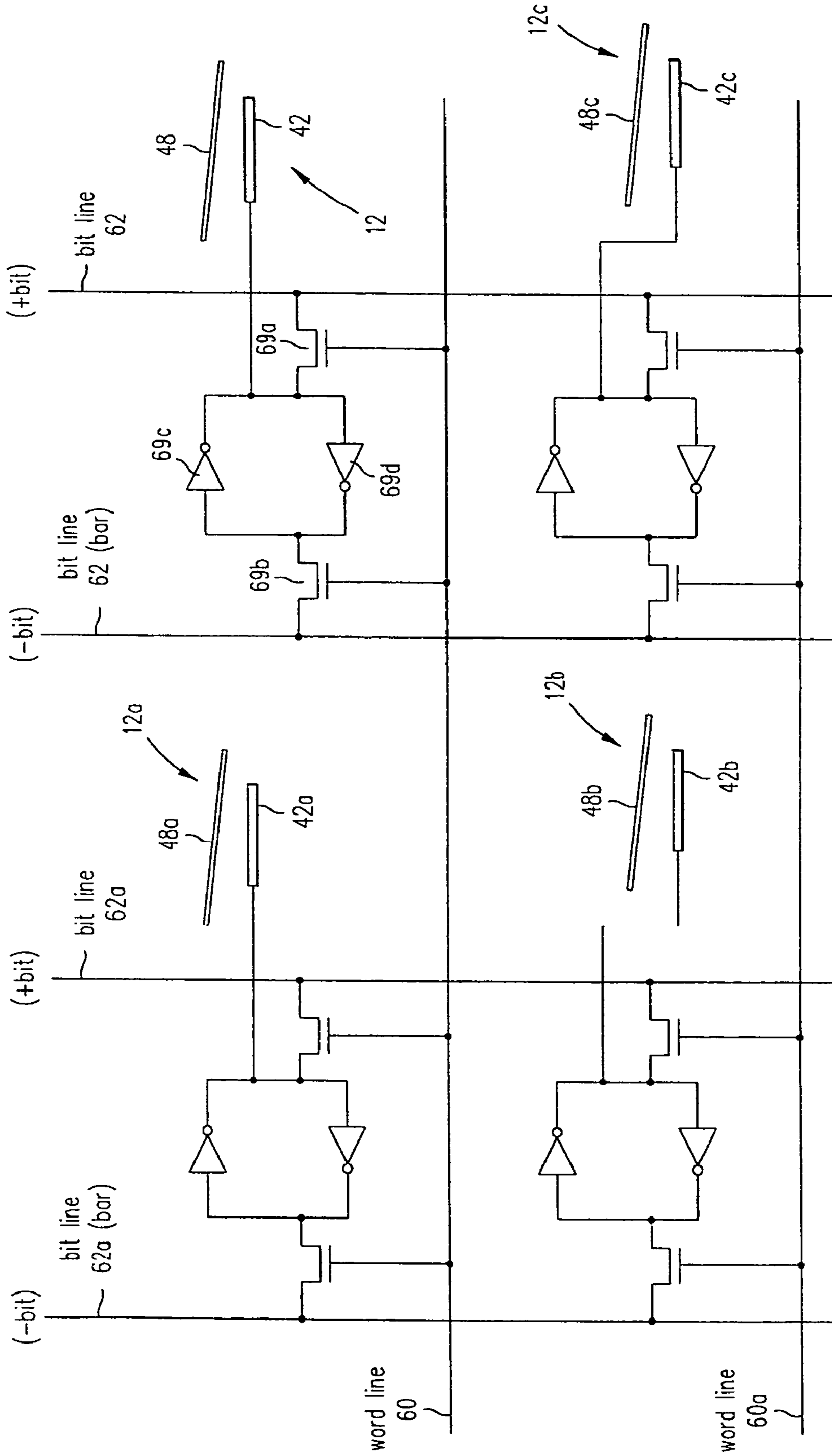
SRAM Implementation
