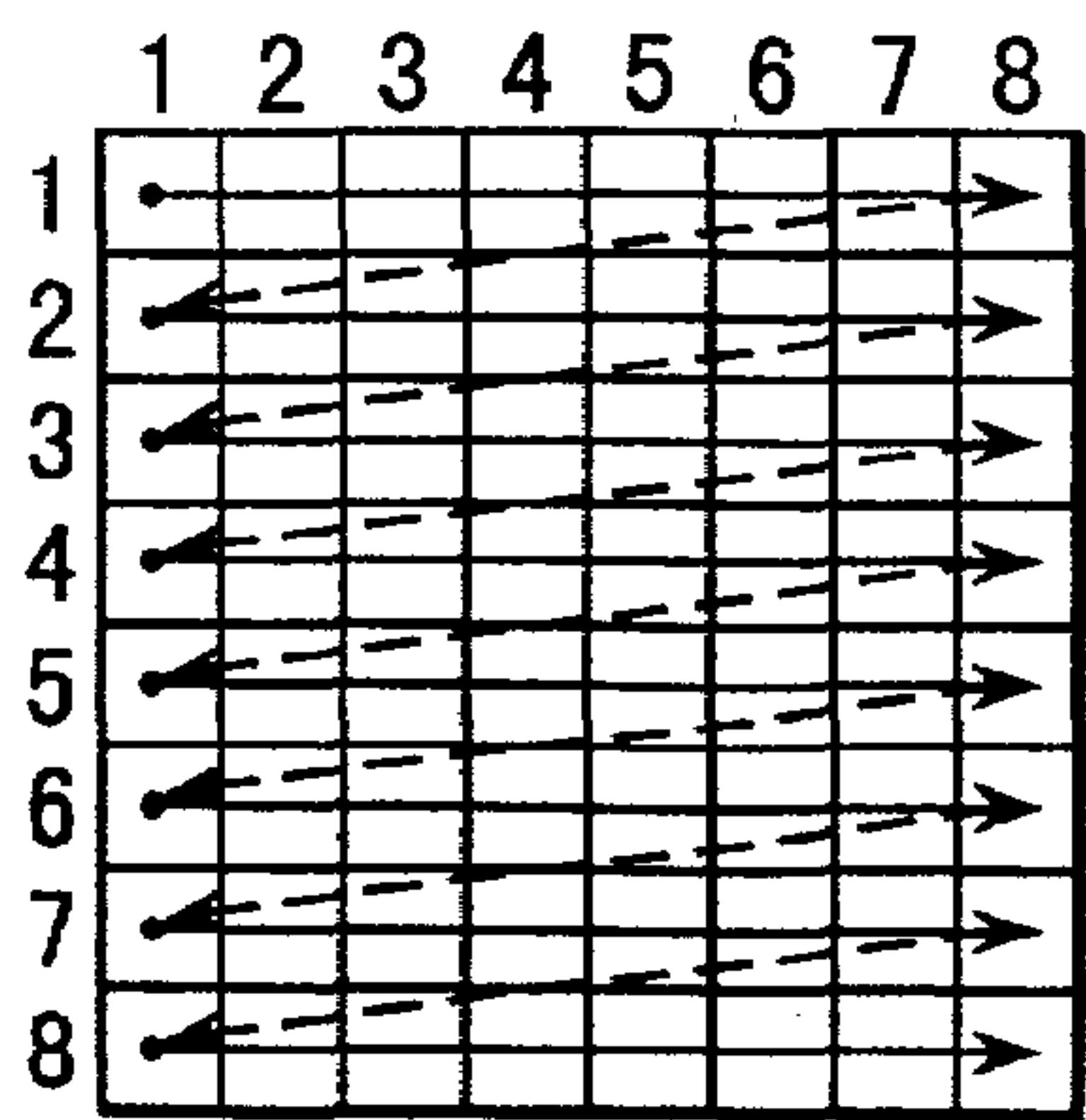
EXAMPLE OF READ SEQUENCE FOR 8x8 BLOCKS
