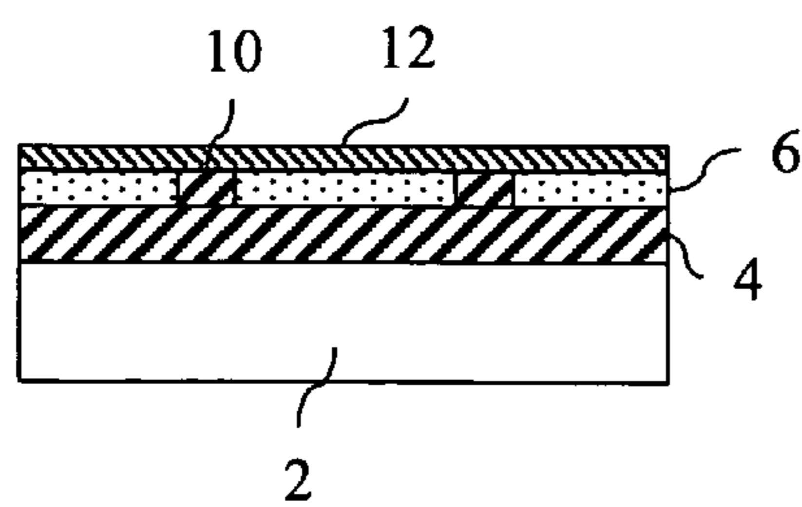
SECTION AA
