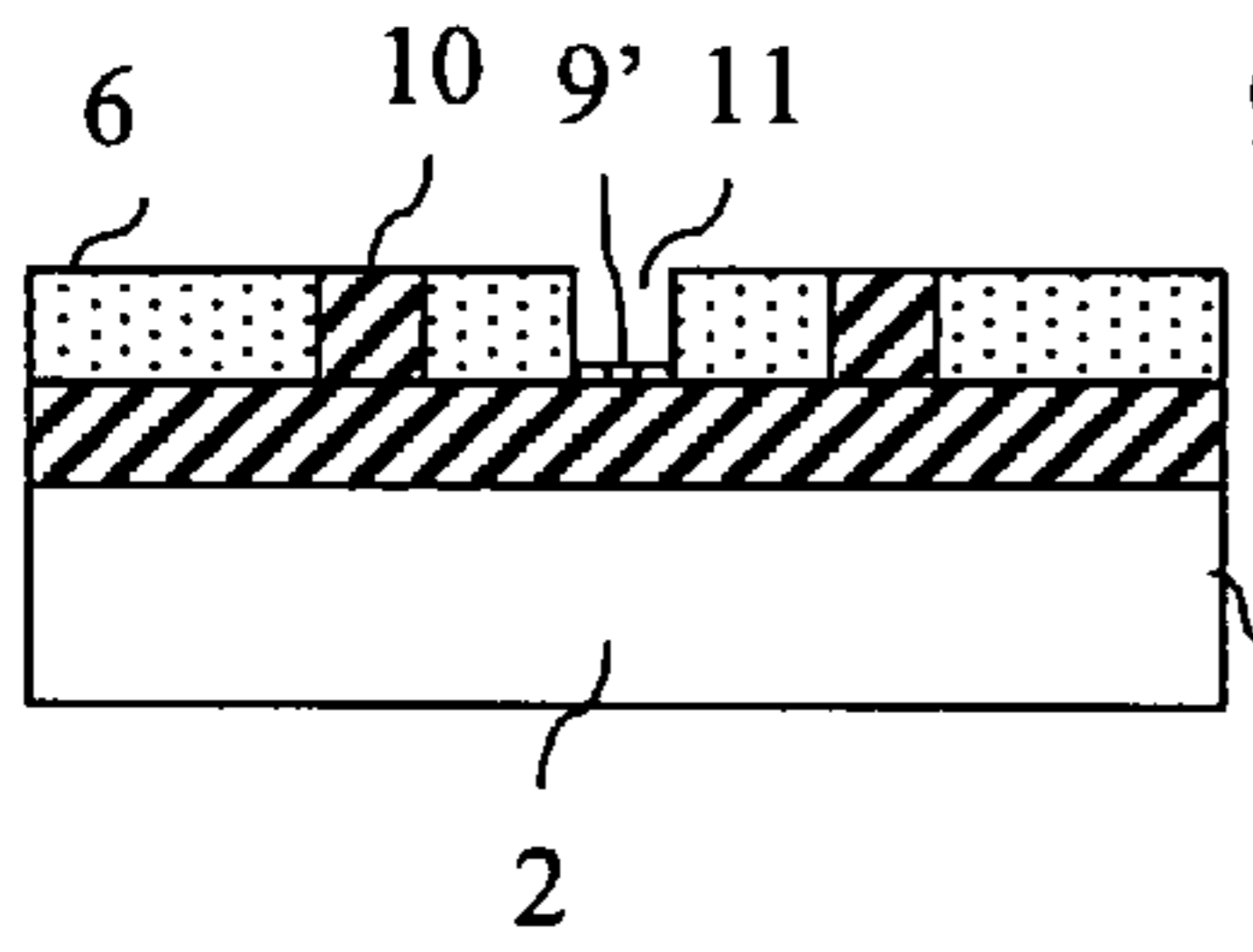
SECTION AA
