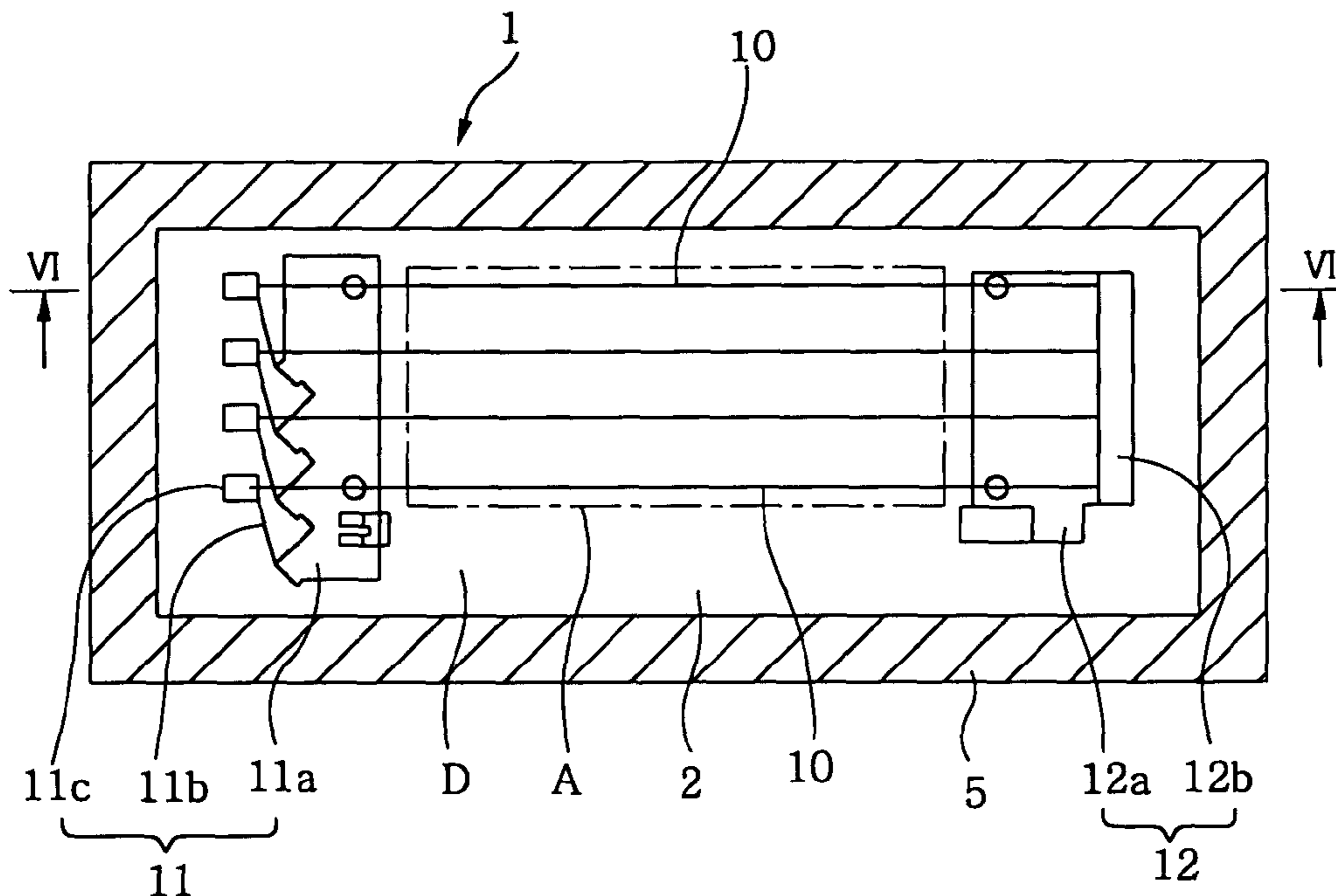
FIG. 5 (PRIOR ART)
