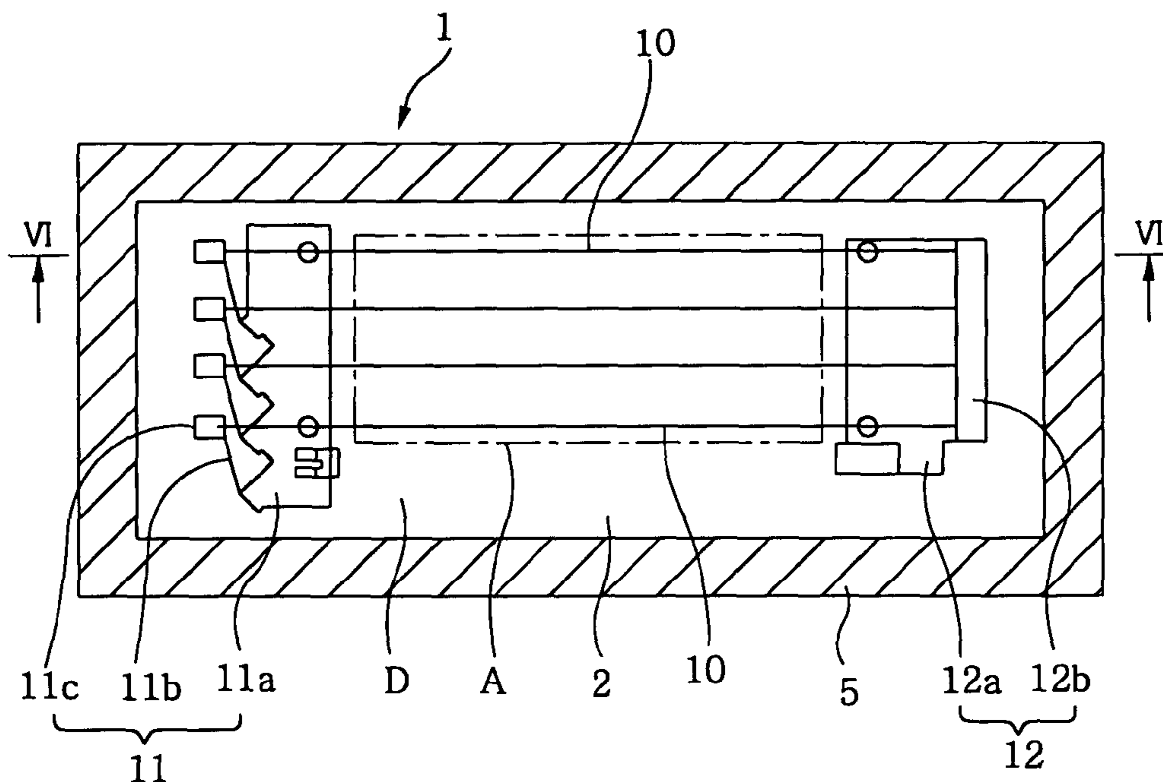
FIG. 5 (PRIOR ART)
