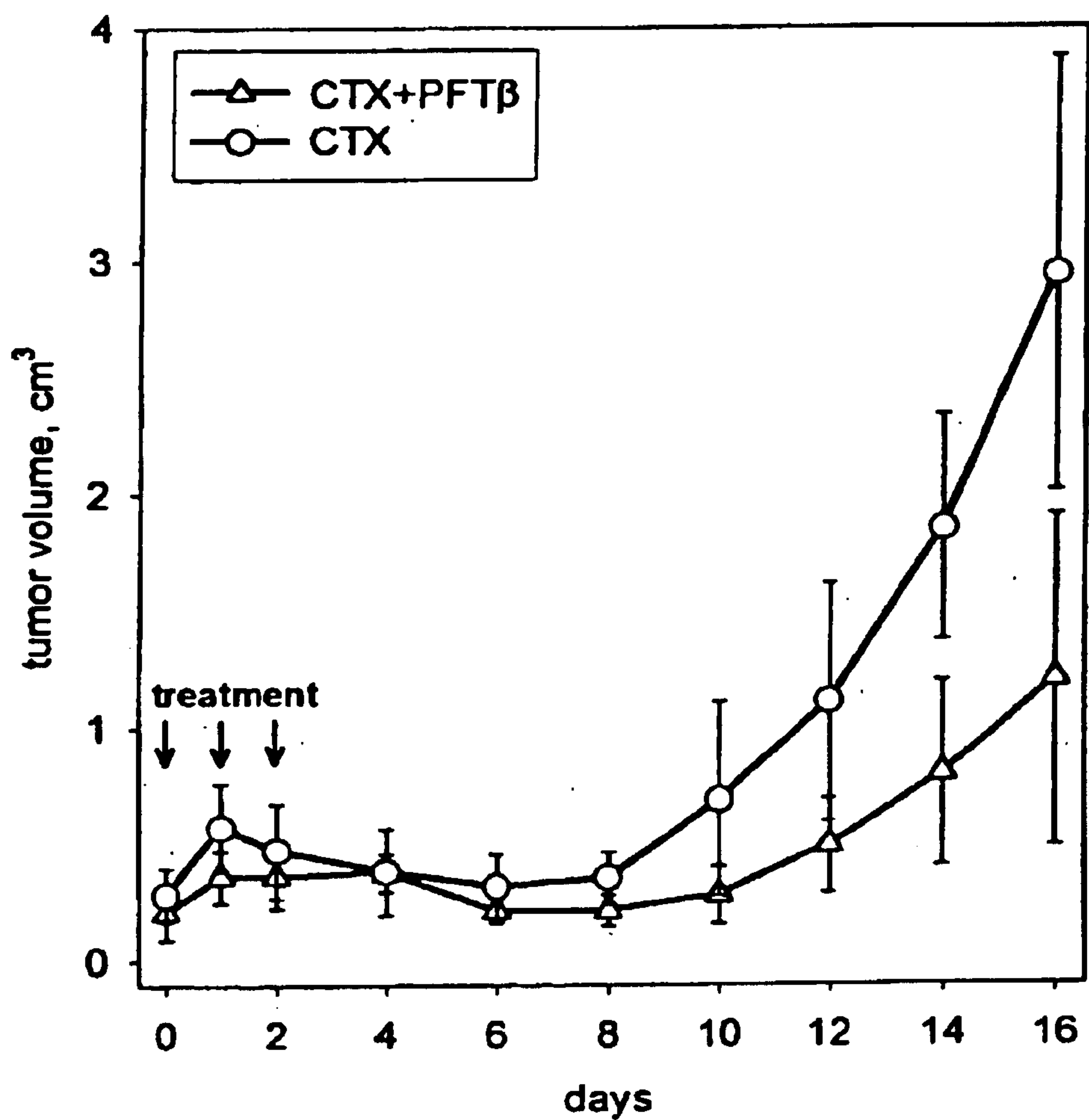
Effect of PFT \beta on LLC tumor response to cyclophosphamide in C57BL mice
