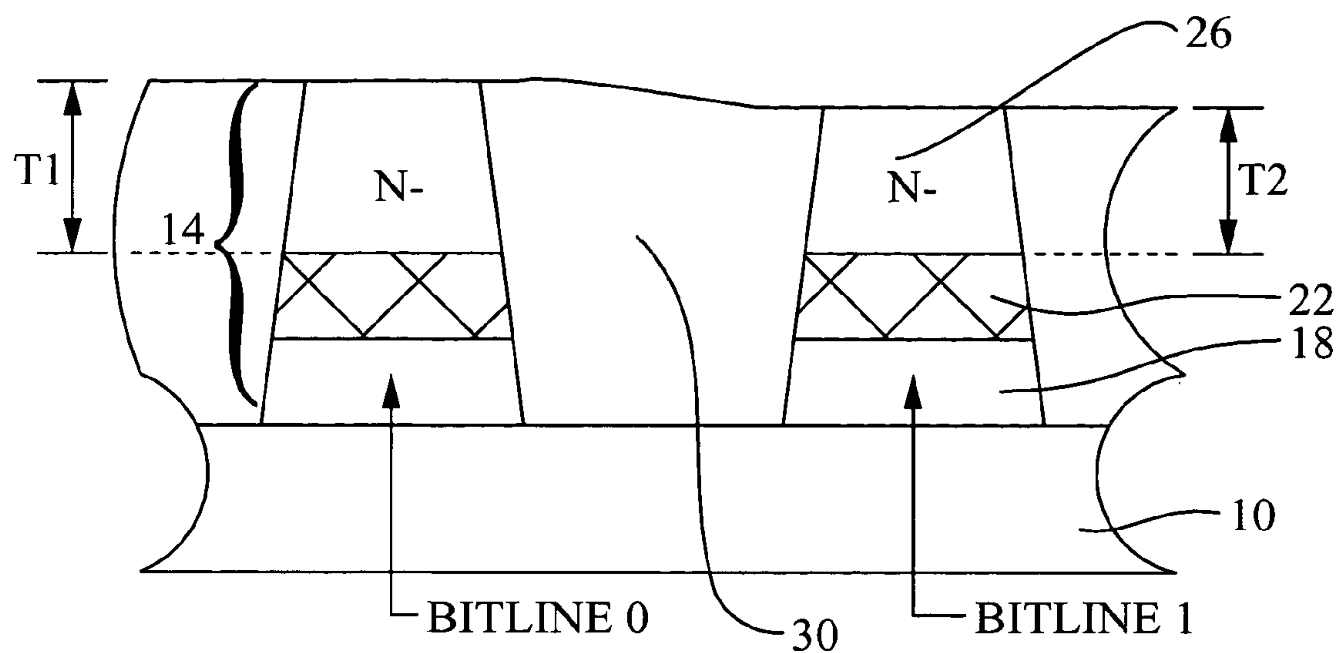
FIG. 3 Prior Art
