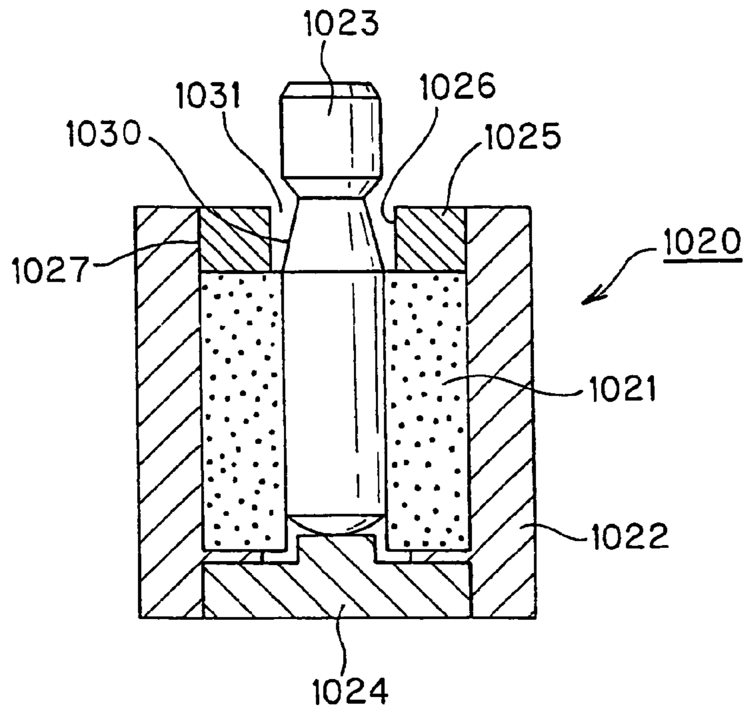
FIG. 1 PRIOR ART
