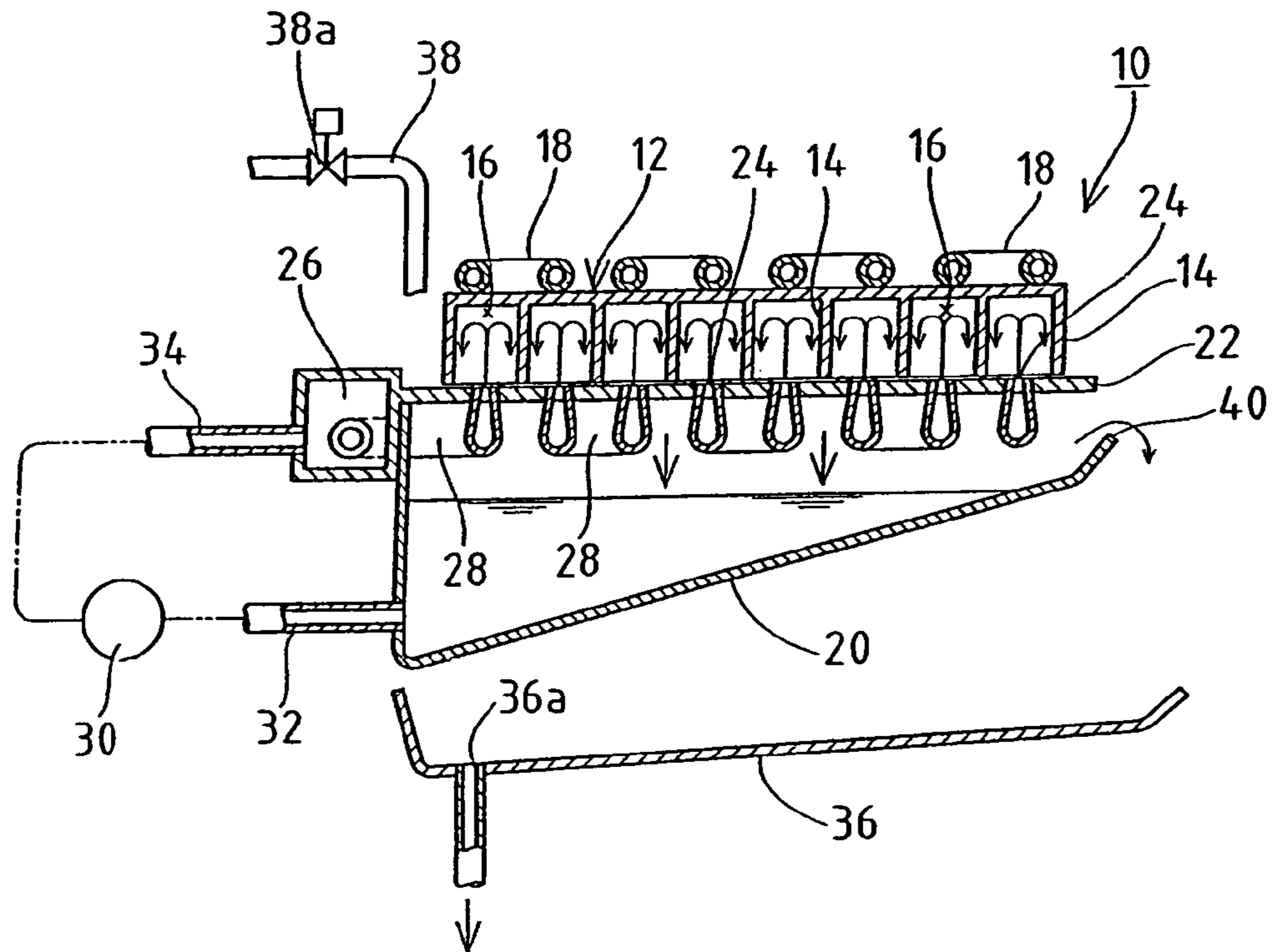
FIG. 10 PRIOR ART
