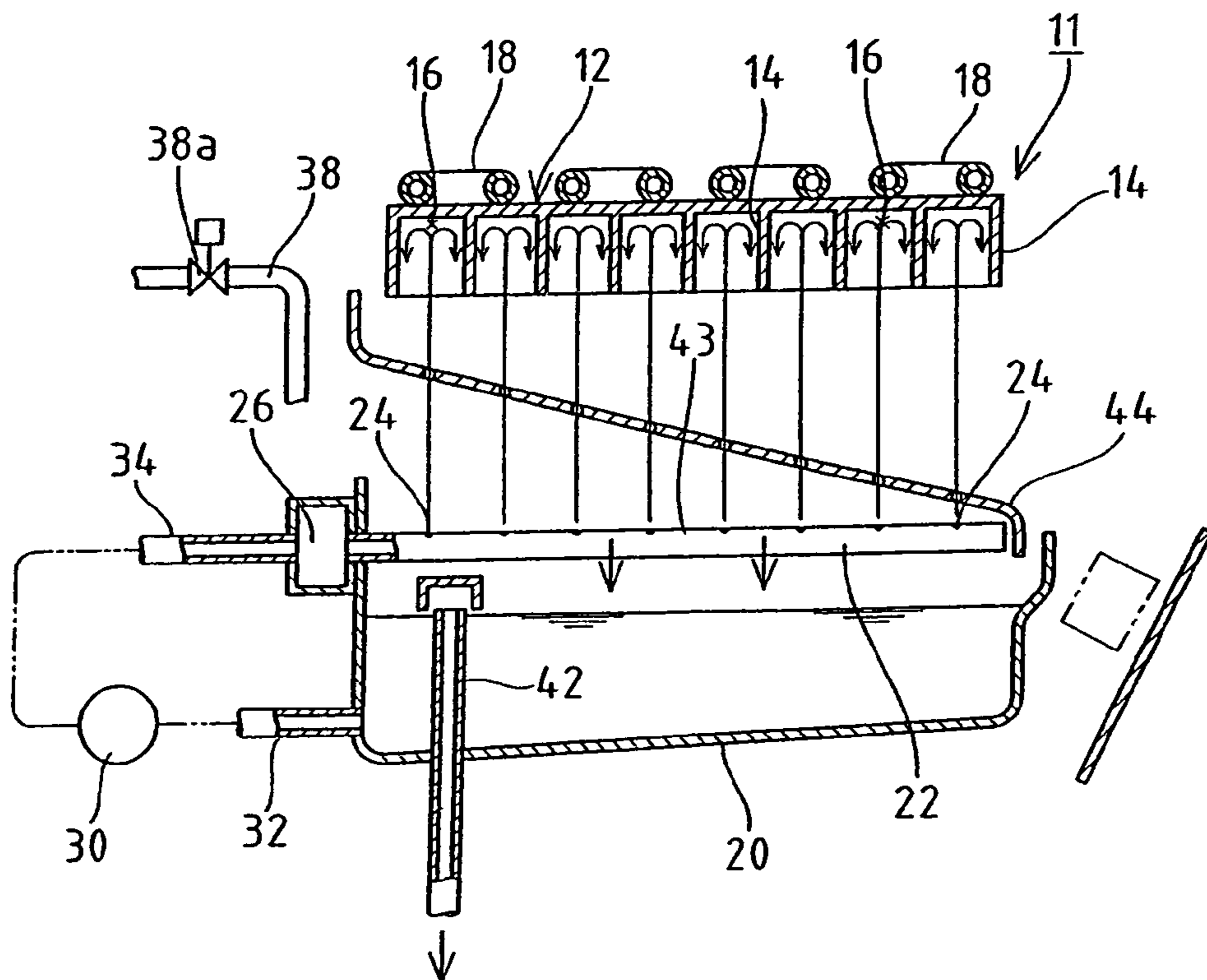
FIG. 11 PRIOR ART
