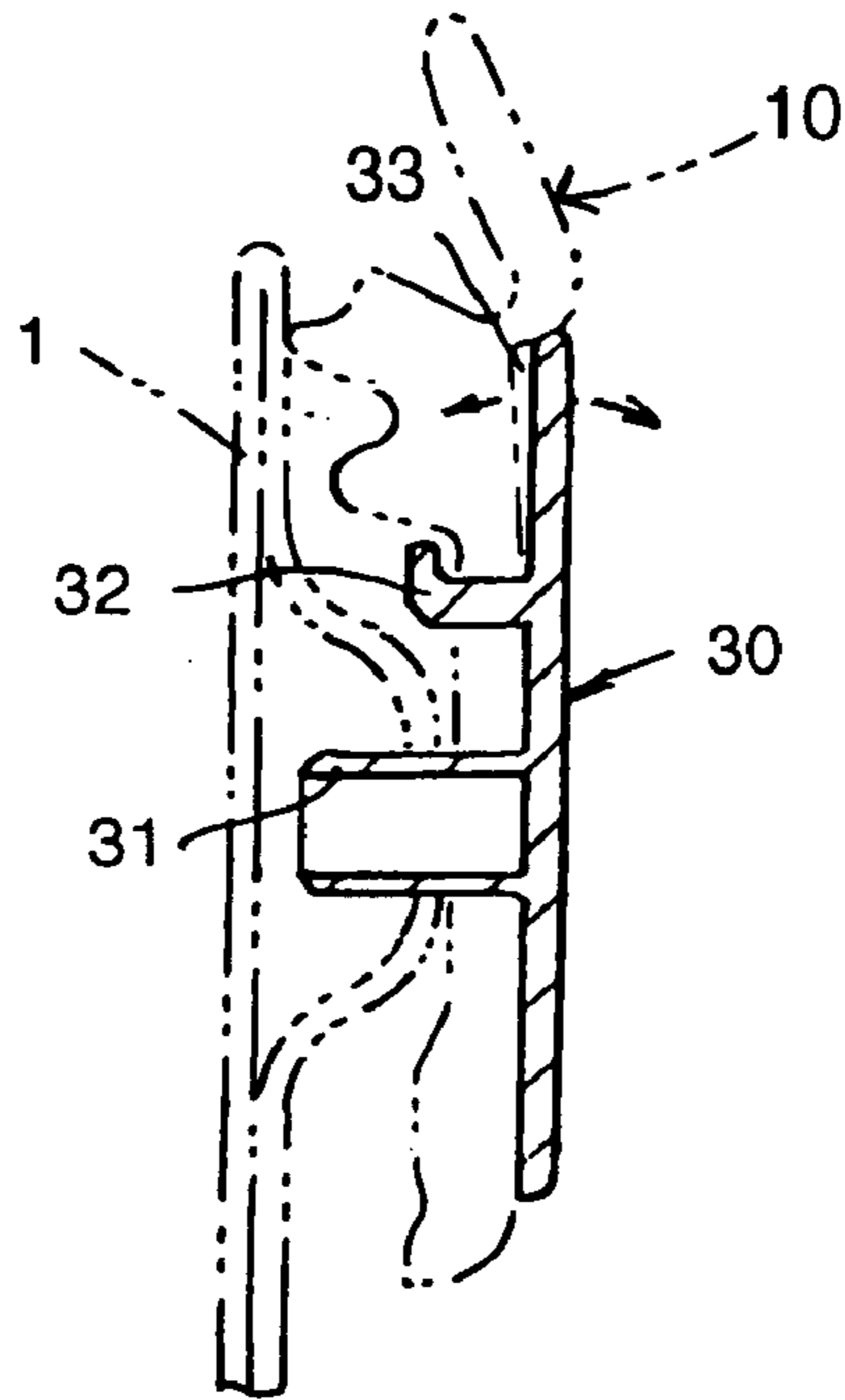
FIG. 3(PRIOR ART)
