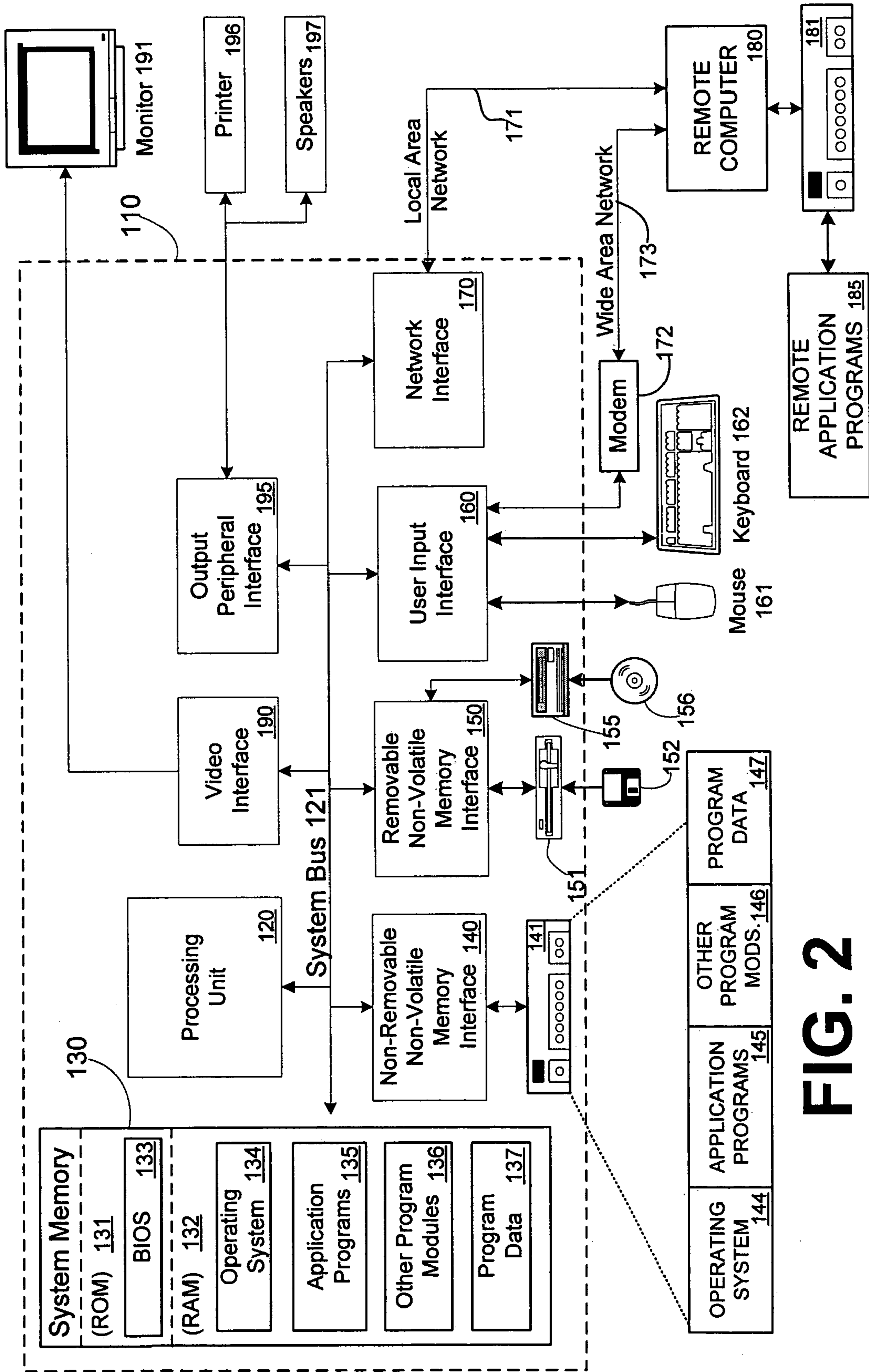
Computing Environment 100
