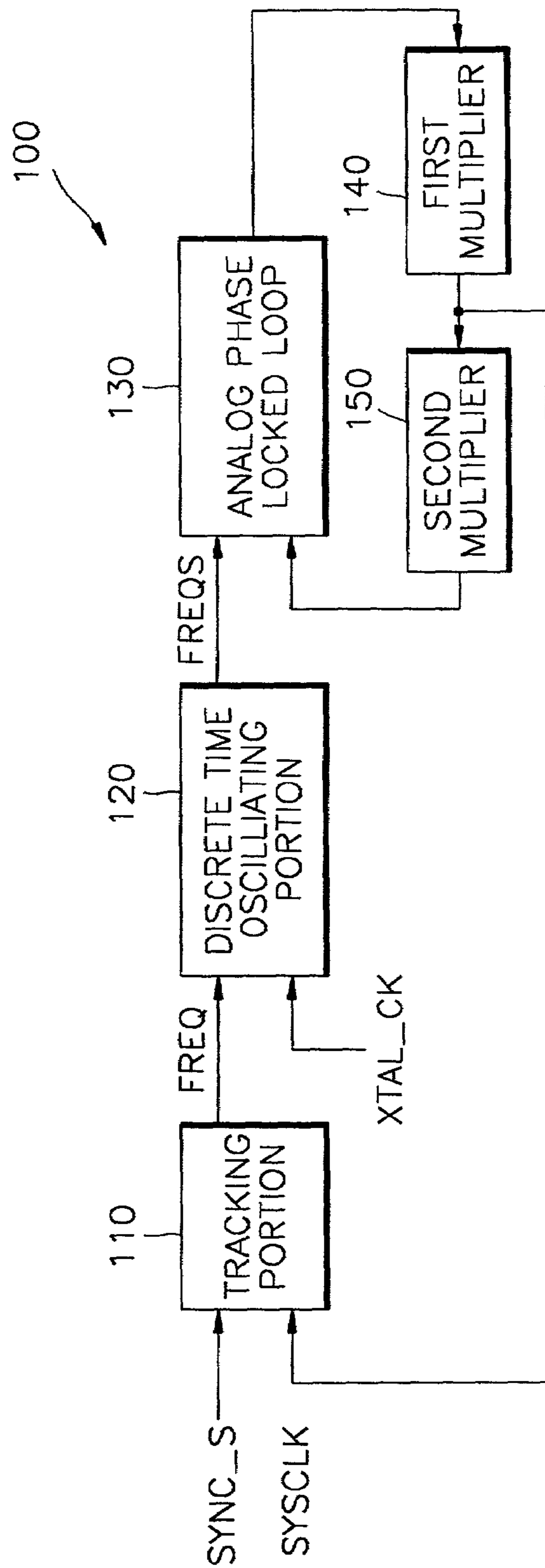
FIG. 1 (PRIOR ART)
