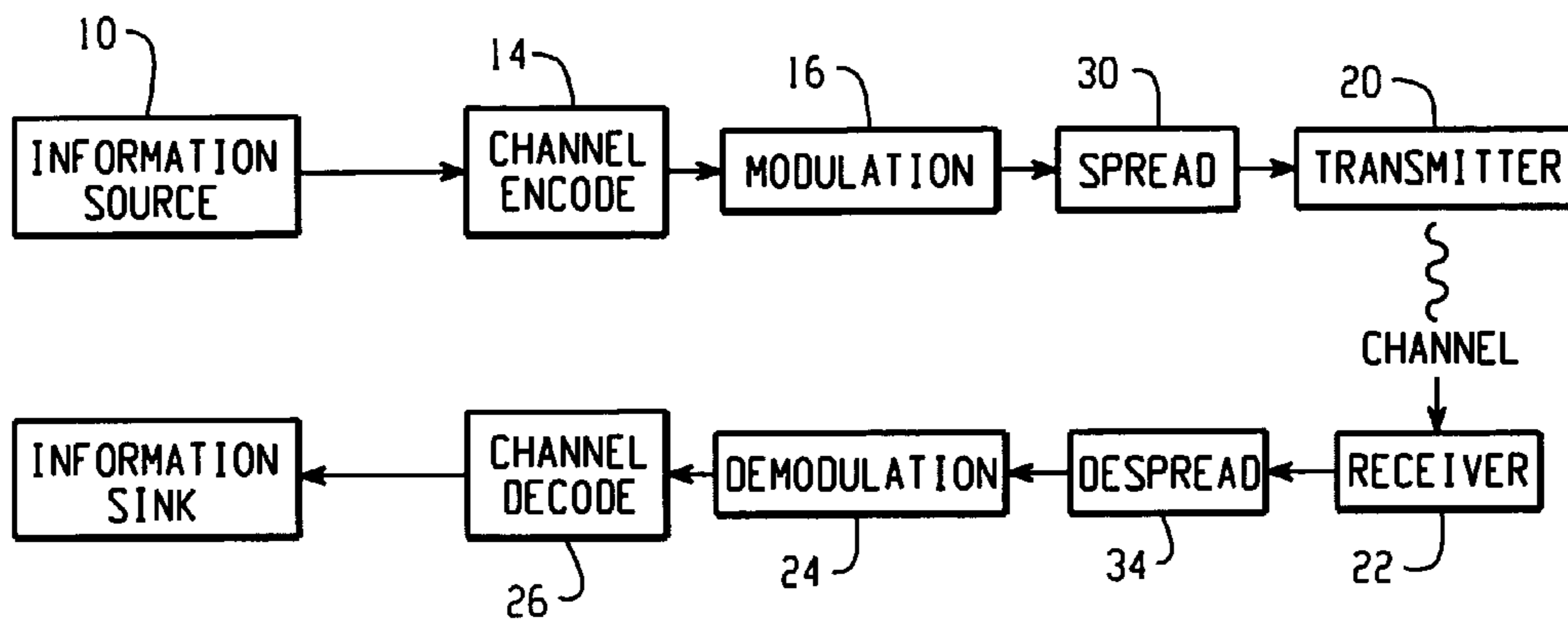
Fig. 1 PRIOR ART
