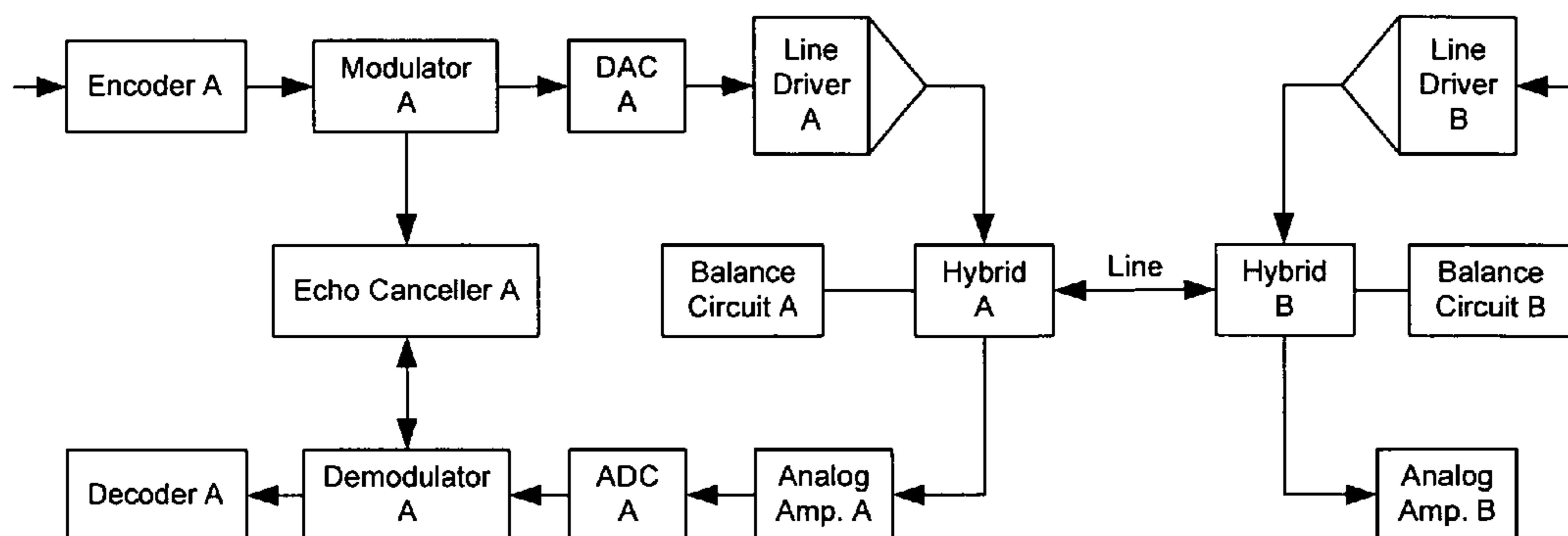
FIG. 1 (Prior Art)
