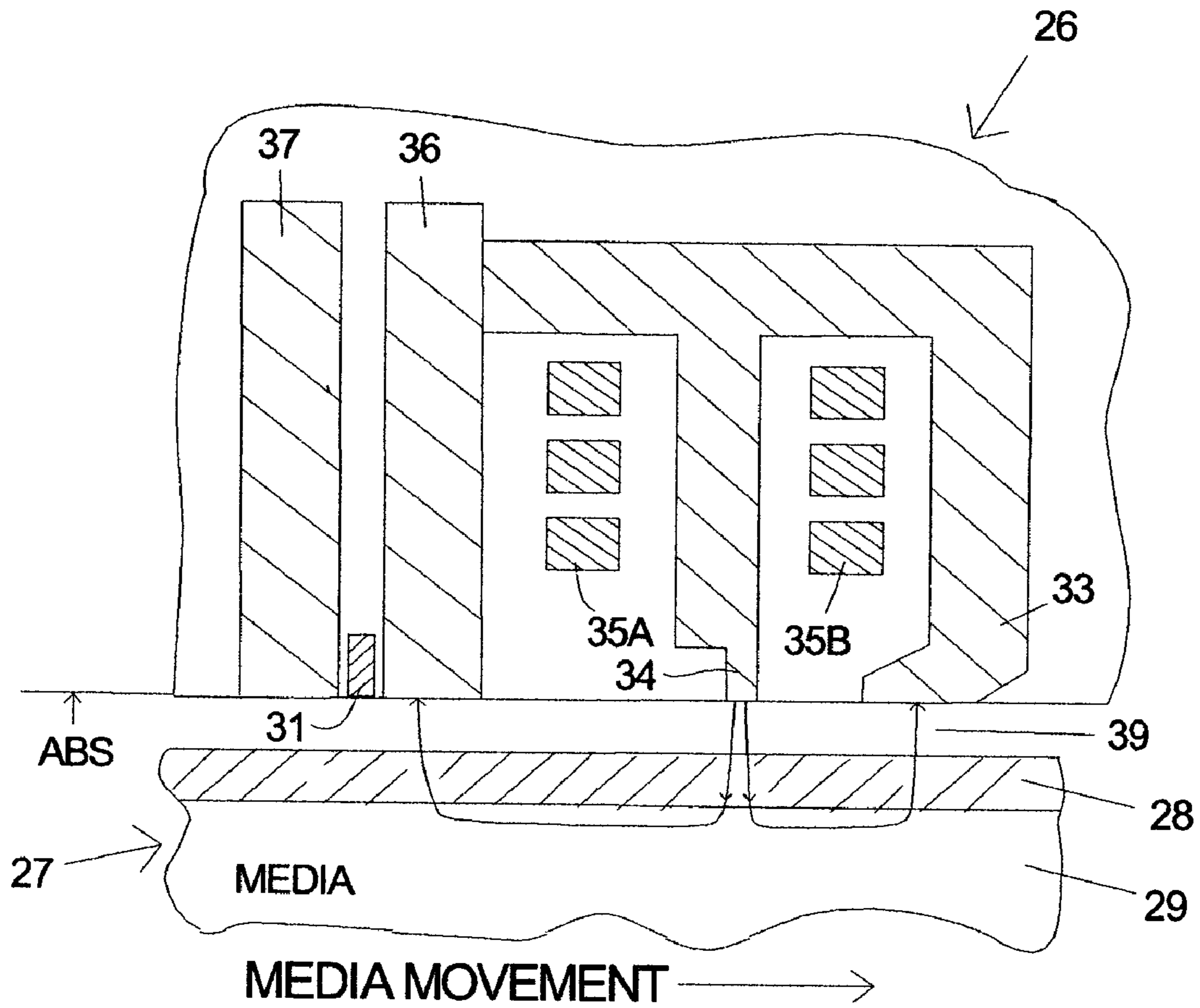
Fig. 1 (Prior Art)
