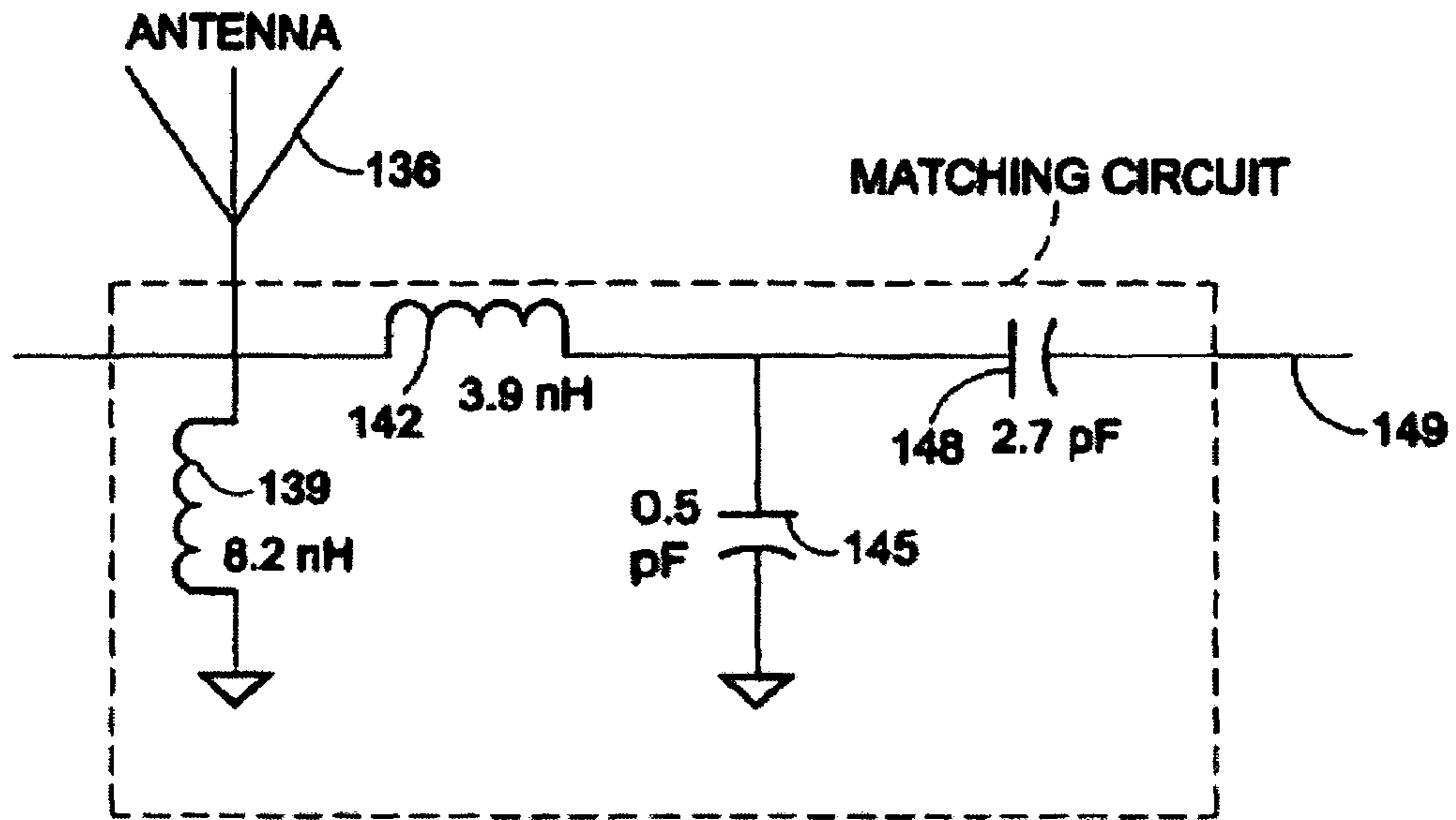
FIG. 7 ANTENNA MATCHING CIRCUIT
