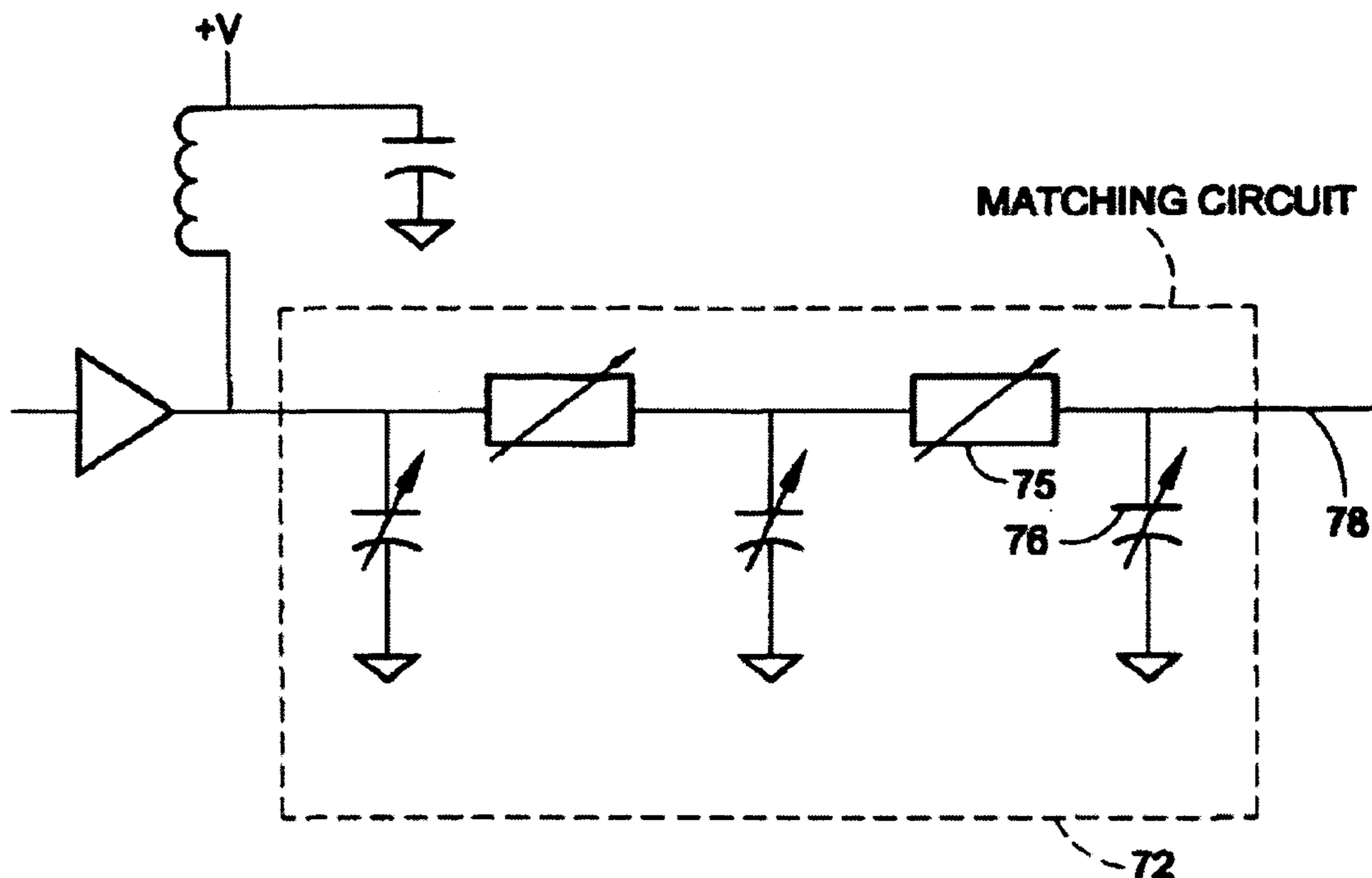
SINGLE BAND POWER AMPLIFIER MATCHING CIRCUIT
